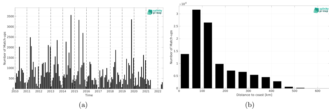
Figure 1: Number of match-ups between ICES and SMOS SSS L3 v8 - 18 Days (CATDS-CEC-LOCEAN) SSS as a function of time (a) and as function of the distance to coast (b) over the Arctic Ocean Pi-MEP region and for the full satellite product period.
