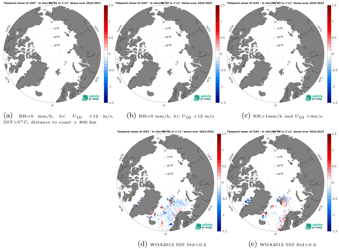
Figure 12: Temporal mean gridded over spatial boxes of size 1^{\circ}\times 1^{\circ} of \Delta\text{SSS} (SMOS SSS L3 v8 - 18 Days (CATDS-CEC-LOCEAN) - ICES) for 5 different subdatasets corresponding to: RR=0 mm/h, 3 < U_{10} < 12 m/s, SST > 5^{\circ}\text{C} , distance to coast > 800 km (a), RR=0 mm/h, 3 < U_{10} < 12 m/s (b), RR > 1 mm/h and U_{10} < 4 m/s (c), WOA2013 SSS Std < 0.2 (d), WOA2013 SSS Std > 0.2 (e).
