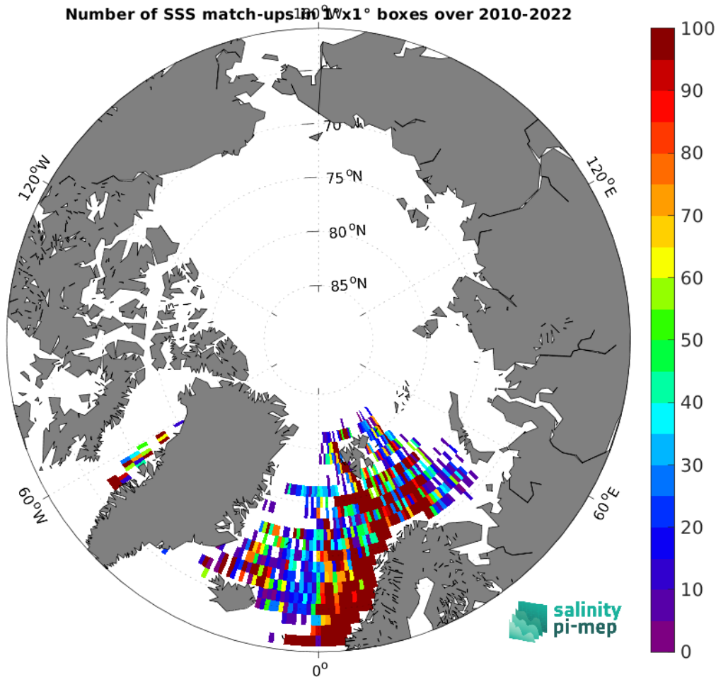
Figure 4: Number of SSS match-ups between ICES SSS and the SMOS SSS L3 v8 - 18 Days (CATDS-CEC-LOCEAN) SSS product for the Arctic Ocean Pi-MEP region over 1^\circ \times 1^\circ boxes and for the full satellite product period.
