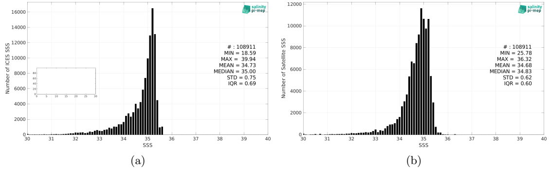
Figure 2: Histograms of SSS from ICES (a) and SMOS SSS L3 v8 - 18 Days (CATDS-CEC-LOCEAN) (b) considering all match-up pairs per bins of 0.1 over the Arctic Ocean Pi-MEP region and for the full satellite product period.
