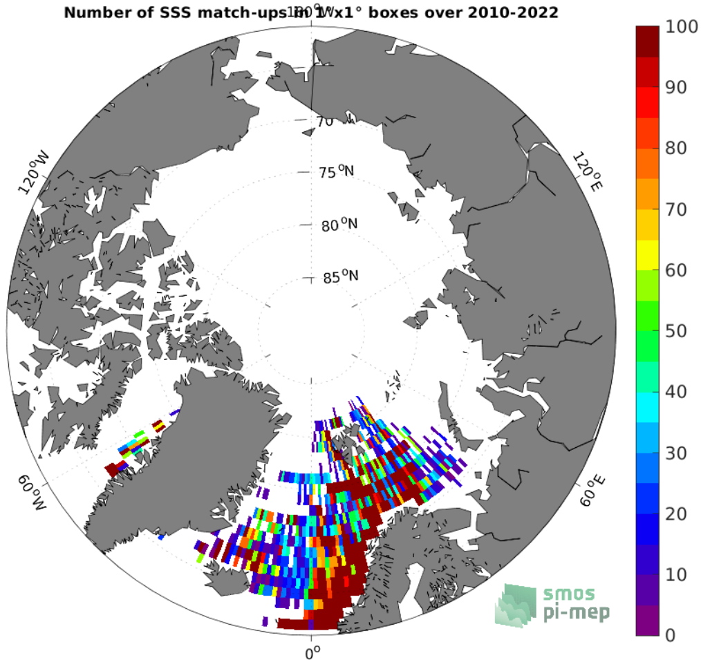
Figure 4: Number of SSS match-ups between ICES SSS and the SMOS SSS L3 v8 - 18 Days (CATDS-CECOS-LOCEAN) SSS product for the Arctic Ocean Pi-MEP region over 1^\circ \times 1^\circ boxes and for the full satellite product period.
