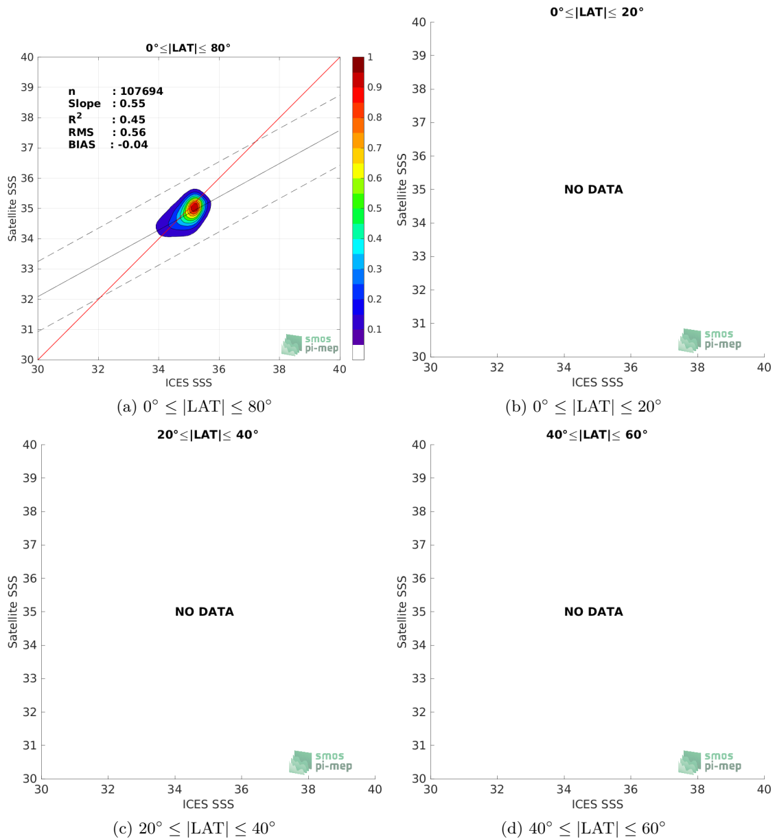
Figure 9: Contour maps of the concentration of SMOS SSS L3 v8 - 18 Days (CATDS-CECOS-LOCEAN) SSS (y-axis) versus ICES SSS (x-axis) at match-up pairs for different latitude bands. For each plot, the red line shows x=y . The black thin and dashed lines indicate a linear fit through the data cloud and the \pm 95\% confidence levels, respectively. The number match-up pairs n , the slope and R^2 coefficient of the linear fit, the root mean square (RMS) and the mean bias between satellite and in situ data are indicated for each latitude band in each plots.
