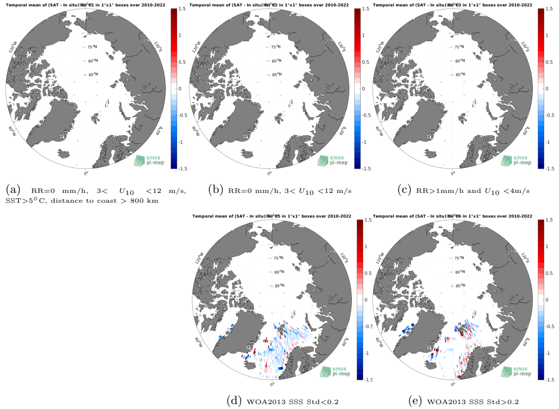
Figure 12: Temporal mean gridded over spatial boxes of size 1^{\circ}\times 1^{\circ} of \Delta\text{SSS} (SMOS SSS L3 v8 - 18 Days (CATDS-CECOS-LOCEAN) - ICES) for 5 different subdatasets corresponding to:RR=0 mm/h, 3 < U_{10} < 12 m/s, SST > 5^{\circ}\text{C} , distance to coast > 800 km (a), RR=0 mm/h, 3 < U_{10} < 12 m/s (b), RR > 1 mm/h and U_{10} < 4 m/s (c), WOA2013 SSS Std < 0.2 (d), WOA2013 SSS Std > 0.2 (e).
