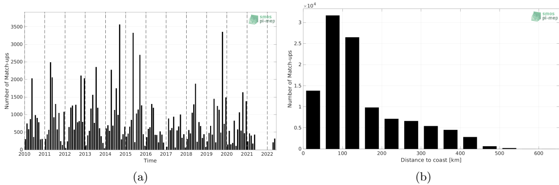
Figure 1: Number of match-ups between ICES and SMOS SSS L3 v8 - 18 Days (CATDS-CECOS-LOCEAN) SSS as a function of time (a) and as function of the distance to coast (b) over the Arctic Ocean Pi-MEP region and for the full satellite product period.
