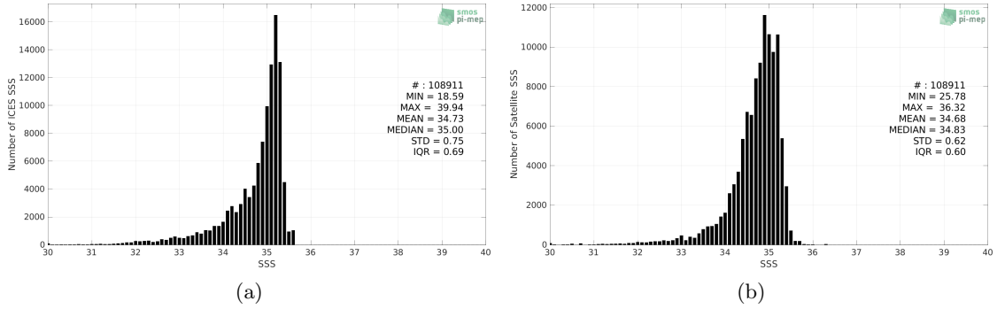
Figure 2: Histograms of SSS from ICES (a) and SMOS SSS L3 v8 - 18 Days (CATDS-CECOS-LOCEAN) (b) considering all match-up pairs per bins of 0.1 over the Arctic Ocean Pi-MEP region and for the full satellite product period.
