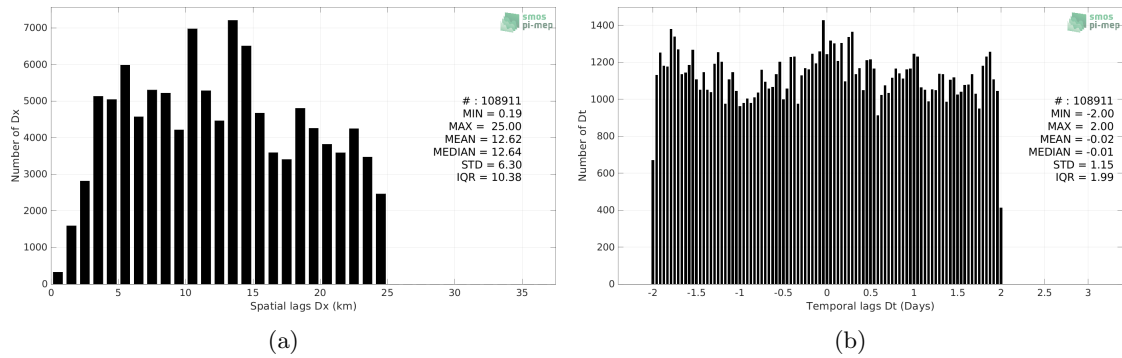
Figure 5: Histograms of the spatial (a) and temporal (b) lags between the location/time of the ICES measurement and the date of the corresponding SMOS SSS L3 v8 - 18 Days (CATDS-CECOS-LOCEAN) SSS pixel.
