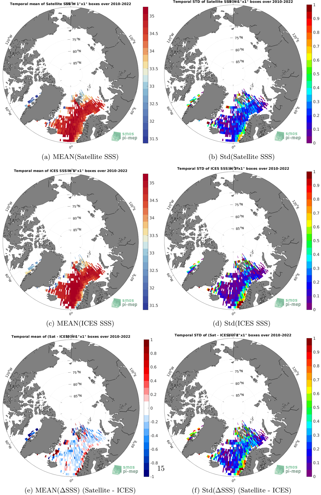
Figure 6: Temporal mean (left) and Std (right) of SSS from SMOS SSS L3 v8 - 18 Days (CATDS-CECOS-LOCEAN) (top), ICES (middle), and of \Delta SSS (Satellite - ICES). Only match-up pairs are used to generate these maps.
