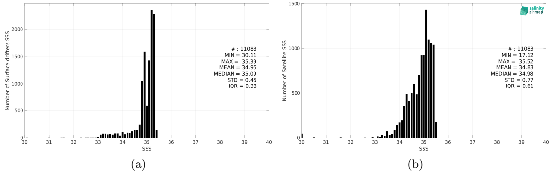
Figure 2: Histograms of SSS from Surface drifters (a) and SMOS SSS L3 v8 - 18 Days (CATDS-CEC-LOCEAN) (b) considering all match-up pairs per bins of 0.1 over the Arctic Ocean Pi-MEP region and for the full satellite product period.
