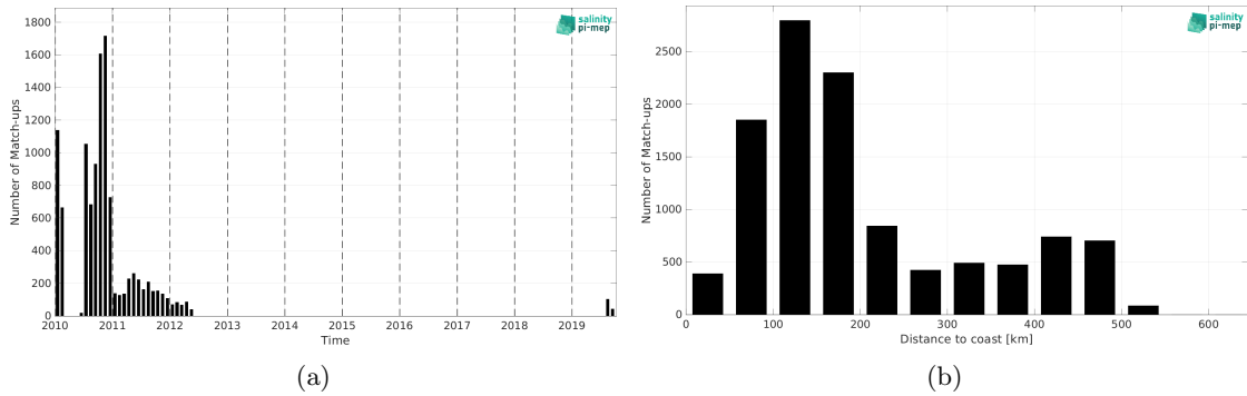
Figure 1: Number of match-ups between Surface drifters and SMOS SSS L3 v8 - 18 Days (CATDS-CEC-LOCEAN) SSS as a function of time (a) and as function of the distance to coast (b) over the Arctic Ocean Pi-MEP region and for the full satellite product period.
