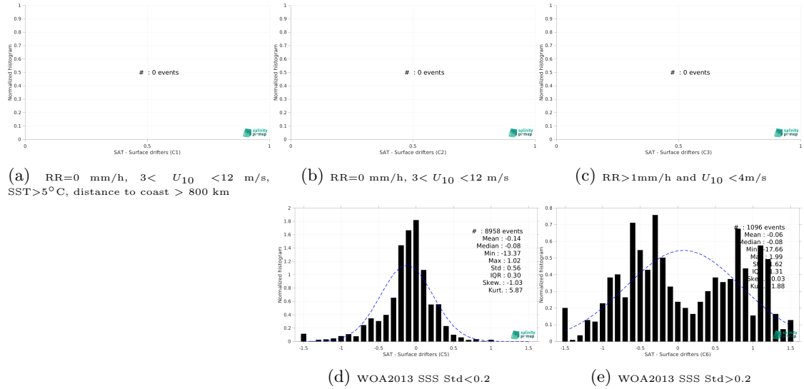
Figure 12: Normalized histogram of \Delta SSS (SMOS SSS L3 v8 - 18 Days (CATDS-CEC-LOCEAN) - Surface drifters) for 5 different subdatasets corresponding to: RR=0 mm/h, 3 < U_{10} < 12 m/s, SST > 5°C, distance to coast > 800 km (a), RR=0 mm/h, 3 < U_{10} < 12 m/s (b), RR > 1mm/h and U_{10} < 4 m/s (c), WOA2013 SSS Std < 0.2 (d), WOA2013 SSS Std > 0.2 (e).
