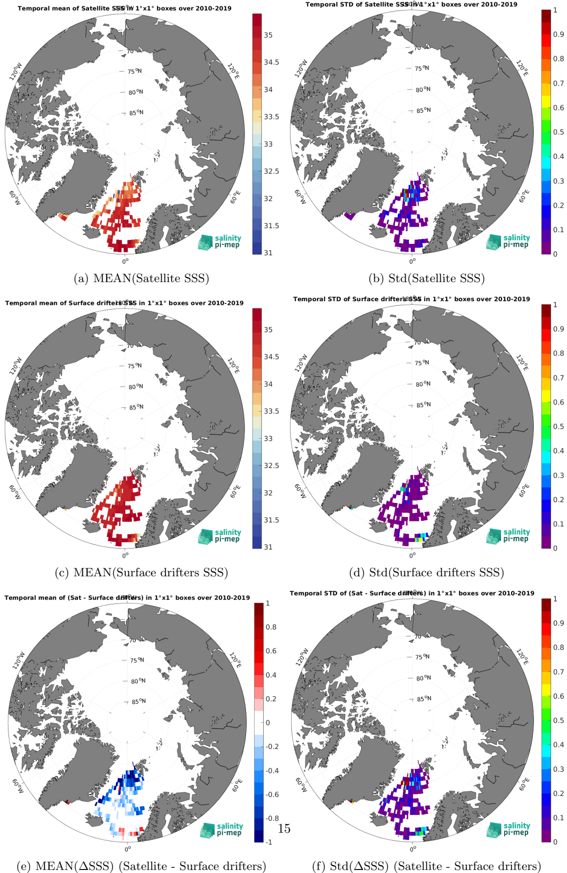
Figure 5: Temporal mean (left) and Std (right) of SSS from SMOS SSS L3 v8 - 18 Days (CATDS-CEC-LOCEAN) (top), Surface drifters (middle), and of \Delta SSS (Satellite - Surface drifters). Only match-up pairs are used to generate these maps.
