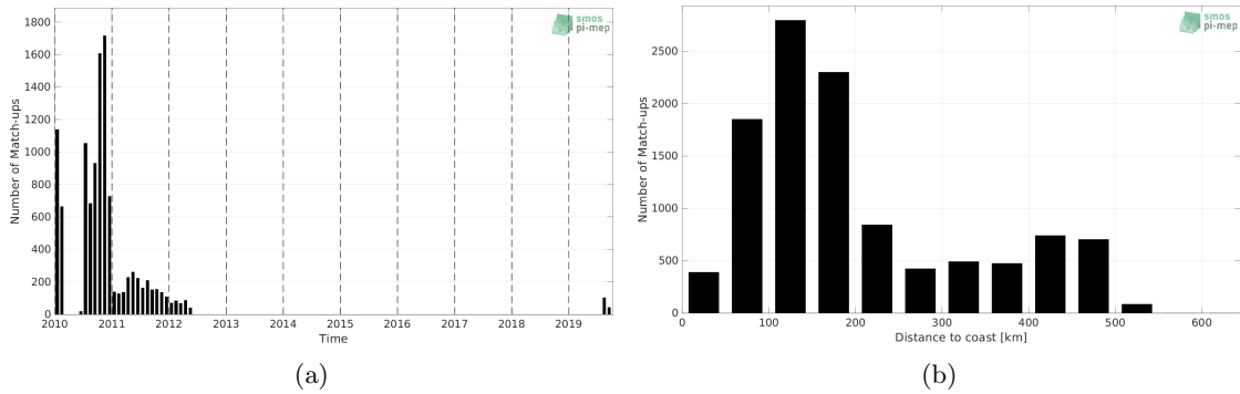
Figure 1: Number of match-ups between Surface drifters and SMOS SSS L3 v8 - 18 Days (CATDS-CECOS-LOCEAN) SSS as a function of time (a) and as function of the distance to coast (b) over the Arctic Ocean Pi-MEP region and for the full satellite product period.
