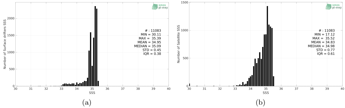
Figure 2: Histograms of SSS from Surface drifters (a) and SMOS SSS L3 v8 - 18 Days (CATDS-CECOS-LOCEAN) (b) considering all match-up pairs per bins of 0.1 over the Arctic Ocean Pi-MEP region and for the full satellite product period.
