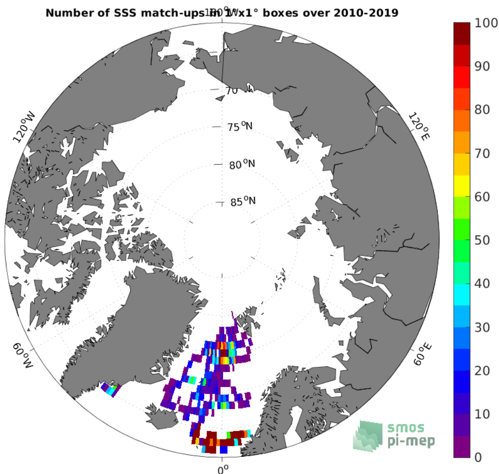
Figure 3: Number of SSS match-ups between Surface drifters SSS and the SMOS SSS L3 v8 - 18 Days (CATDS-CECOS-LOCEAN) SSS product for the Arctic Ocean Pi-MEP region over 1^{\circ} \times 1^{\circ} boxes and for the full satellite product period.
