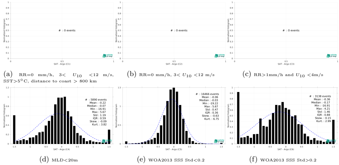
Figure 13: Normalized histogram of \Delta SSS (SMOS SSS L3 v8 - 18 Days (CATDS-CEC-LOCEAN) - Argo) for 6 different subdatasets corresponding to: RR=0 mm/h, 3 < U_{10} < 12 m/s, SST > 5°C, distance to coast > 800 km (a), RR=0 mm/h, 3 < U_{10} < 12 m/s (b), RR > 1mm/h and U_{10} < 4 m/s (c), MLD < 20m (d), WOA2013 SSS Std < 0.2 (e), WOA2013 SSS Std > 0.2 (f).
