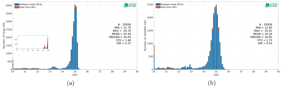
Figure 2: Histograms of SSS from Argo (a) and SMOS SSS L3 v8 - 18 Days (CATDS-CEC-LOCEAN) (b) considering all match-up pairs per bins of 0.1 over the Arctic Ocean Pi-MEP region and for the full satellite product period.
