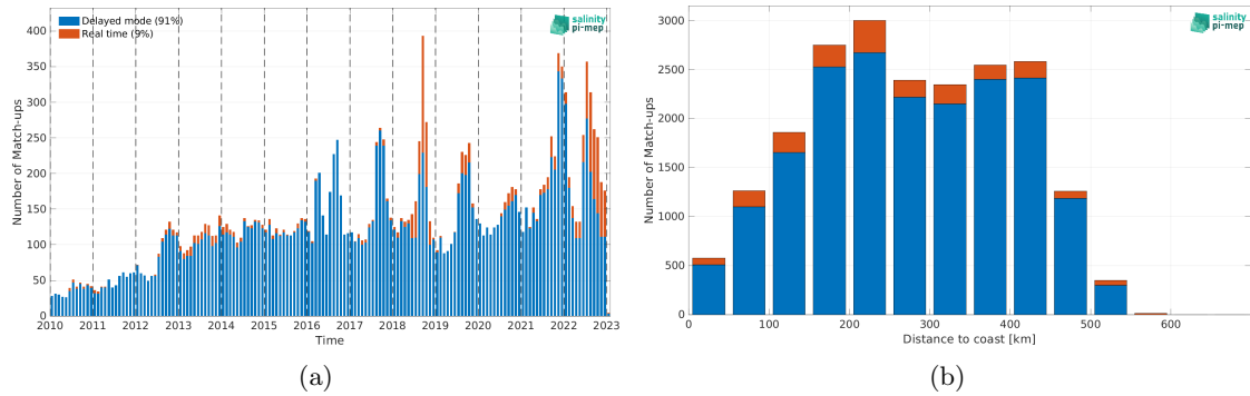
Figure 1: Number of match-ups between Argo and SMOS SSS L3 v8 - 18 Days (CATDS-CEC-LOCEAN) SSS as a function of time (a) and as function of the distance to coast (b) over the Arctic Ocean Pi-MEP region and for the full satellite product period.
