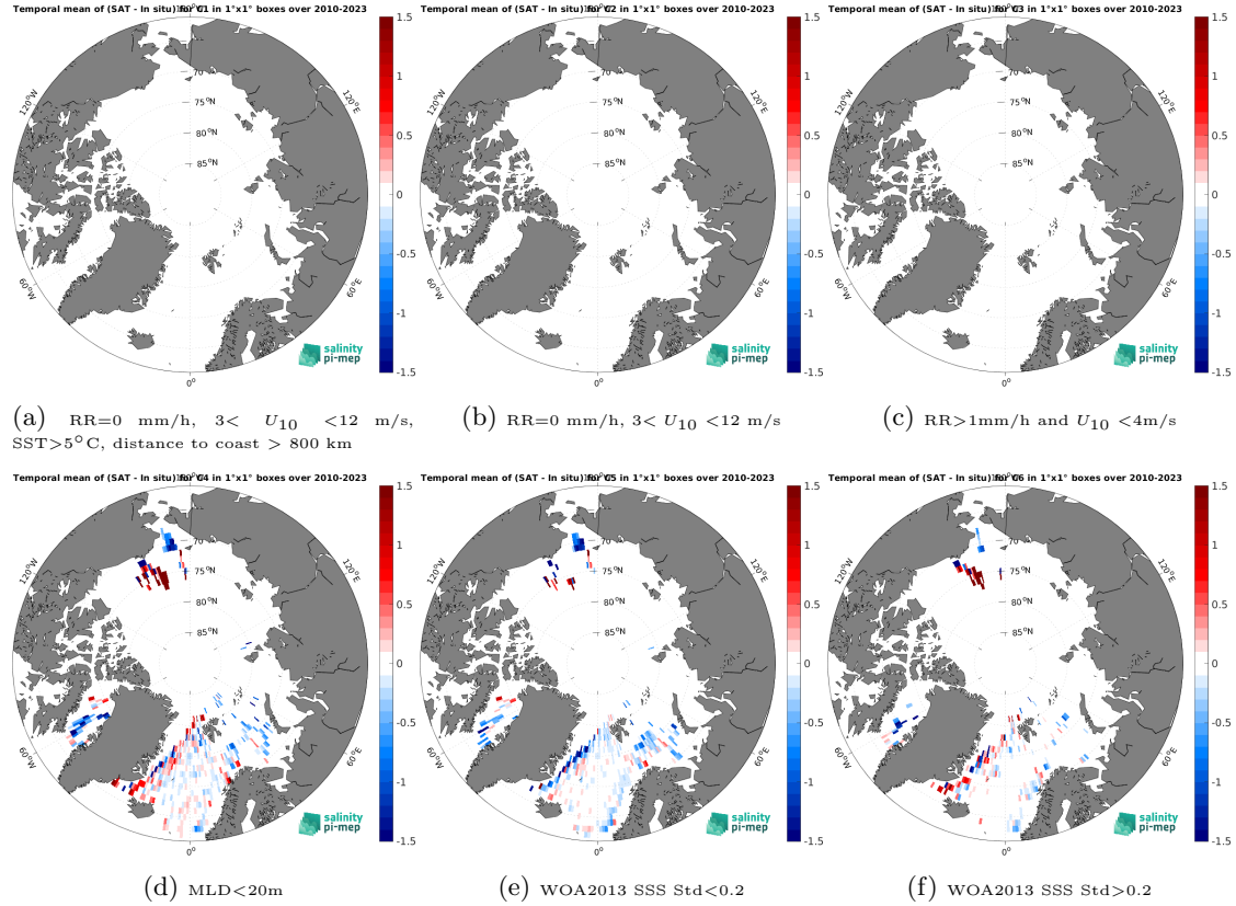
Figure 12: Temporal mean gridded over spatial boxes of size 1^{\circ}\times 1^{\circ} of \Delta\text{SSS} (SMOS SSS L3 v8 - 18 Days (CATDS-CEC-LOCEAN) - Argo) for 6 different subdatasets corresponding to: RR=0 mm/h, 3 < U_{10} < 12 m/s, SST > 5^{\circ}\text{C} , distance to coast > 800 km (a), RR=0 mm/h, 3 < U_{10} < 12 m/s (b), RR > 1 mm/h and U_{10} < 4 m/s (c),MLD < 20\text{m} (d),WOA2013 SSS Std < 0.2 (e),WOA2013 SSS Std > 0.2 (f).
