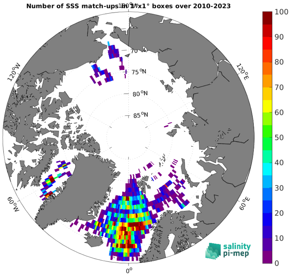
Figure 4: Number of SSS match-ups between Argo SSS and the SMOS SSS L3 v8 - 18 Days (CATDS-CEC-LOCEAN) SSS product for the Arctic Ocean Pi-MEP region over 1^\circ \times 1^\circ boxes and for the full satellite product period.
