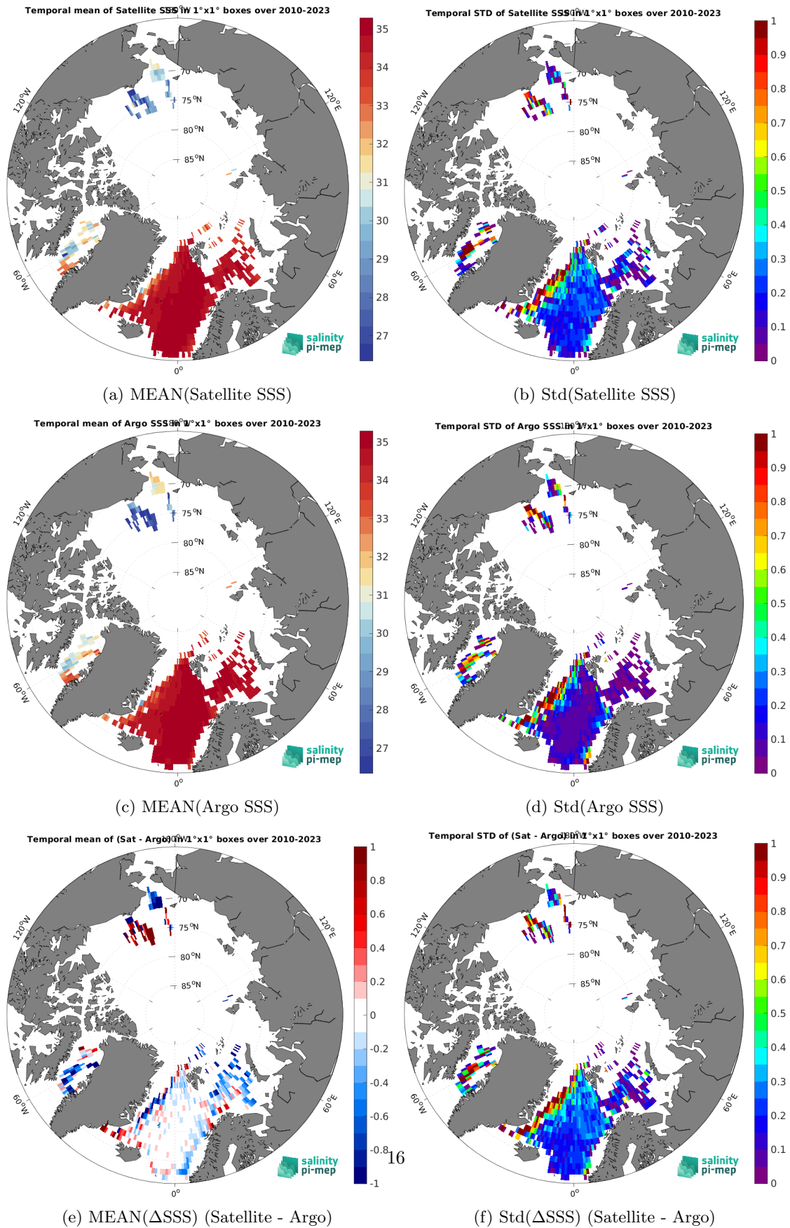
Figure 6: Temporal mean (left) and Std (right) of SSS from SMOS SSS L3 v8 - 18 Days (CATDS-CEC-LOCEAN) (top), Argo (middle), and of \Delta SSS (Satellite - Argo). Only match-up pairs are used to generate these maps.
