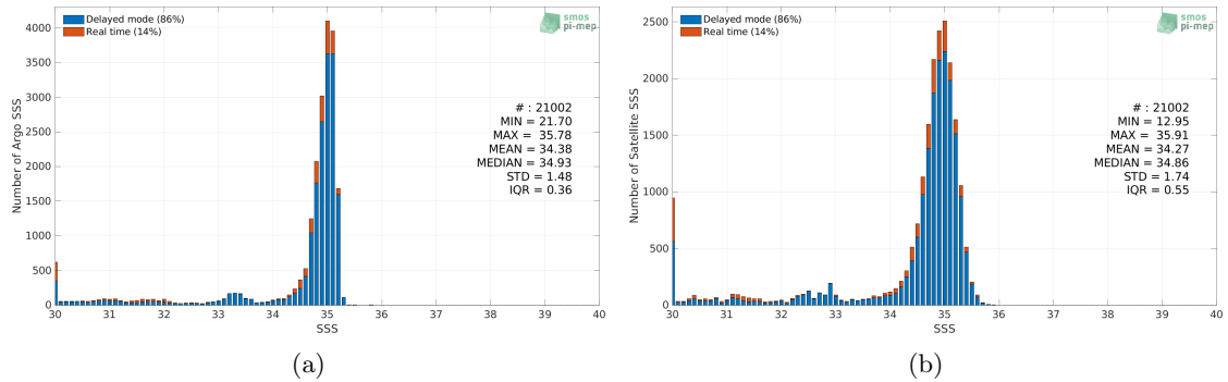
Figure 2: Histograms of SSS from Argo (a) and SMOS SSS L3 v8 - 18 Days (CATDS-CECOS-LOCEAN) (b) considering all match-up pairs per bins of 0.1 over the Arctic Ocean Pi-MEP region and for the full satellite product period.
