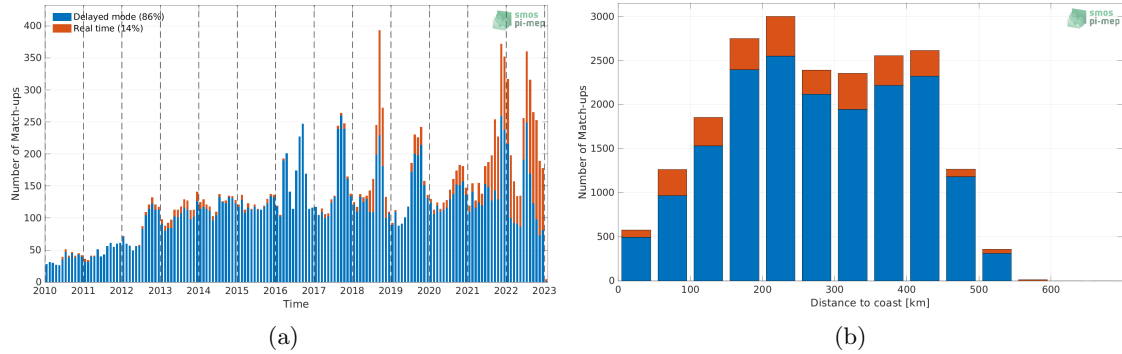
Figure 1: Number of match-ups between Argo and SMOS SSS L3 v8 - 18 Days (CATDS-CECOS-LOCEAN) SSS as a function of time (a) and as function of the distance to coast (b) over the Arctic Ocean Pi-MEP region and for the full satellite product period.
