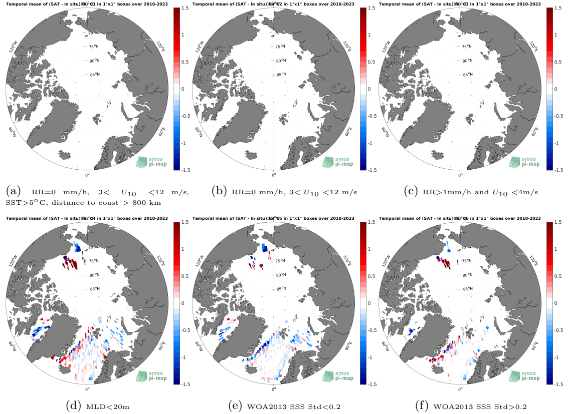
Figure 12: Temporal mean gridded over spatial boxes of size 1^{\circ}\times 1^{\circ} of \Delta\text{SSS} (SMOS SSS L3 v8 - 18 Days (CATDS-CECOS-LOCEAN) - Argo) for 6 different subdatasets corresponding to: RR=0 mm/h, 3 < U_{10} < 12 m/s, SST > 5^{\circ}\text{C} , distance to coast > 800 km (a), RR=0 mm/h, 3 < U_{10} < 12 m/s (b), RR > 1\text{mm/h} and U_{10} < 4\text{m/s} (c), MLD < 20\text{m} (d), WOA2013 SSS Std < 0.2 (e), WOA2013 SSS Std > 0.2 (f).
