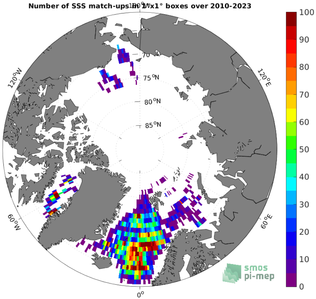
Figure 4: Number of SSS match-ups between Argo SSS and the SMOS SSS L3 v8 - 18 Days (CATDS-CECOS-LOCEAN) SSS product for the Arctic Ocean Pi-MEP region over 1^\circ \times 1^\circ boxes and for the full satellite product period.
