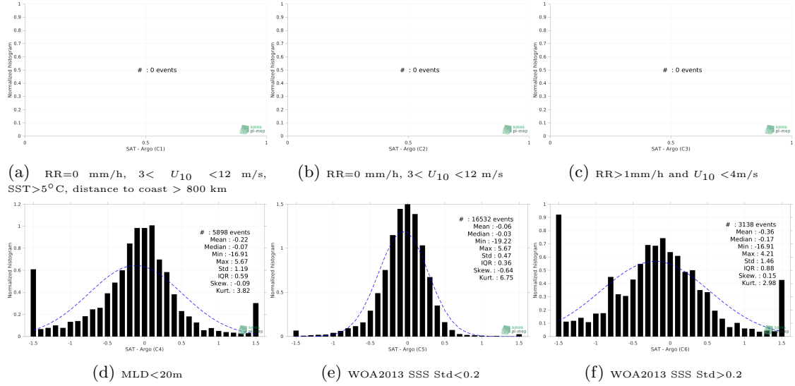
Figure 13: Normalized histogram of \Delta\text{SSS} (SMOS SSS L3 v8 - 18 Days (CATDS-CECOS-LOCEAN) - Argo) for 6 different subdatasets corresponding to: RR=0 mm/h, 3 < U_{10} < 12 m/s, SST > 5^{\circ}\text{C} , distance to coast > 800 km (a), RR=0 mm/h, 3 < U_{10} < 12 m/s (b), RR > 1\text{mm/h} and U_{10} < 4\text{m/s} (c), MLD < 20\text{m} (d), WOA2013 SSS Std < 0.2 (e), WOA2013 SSS Std > 0.2 (f).
