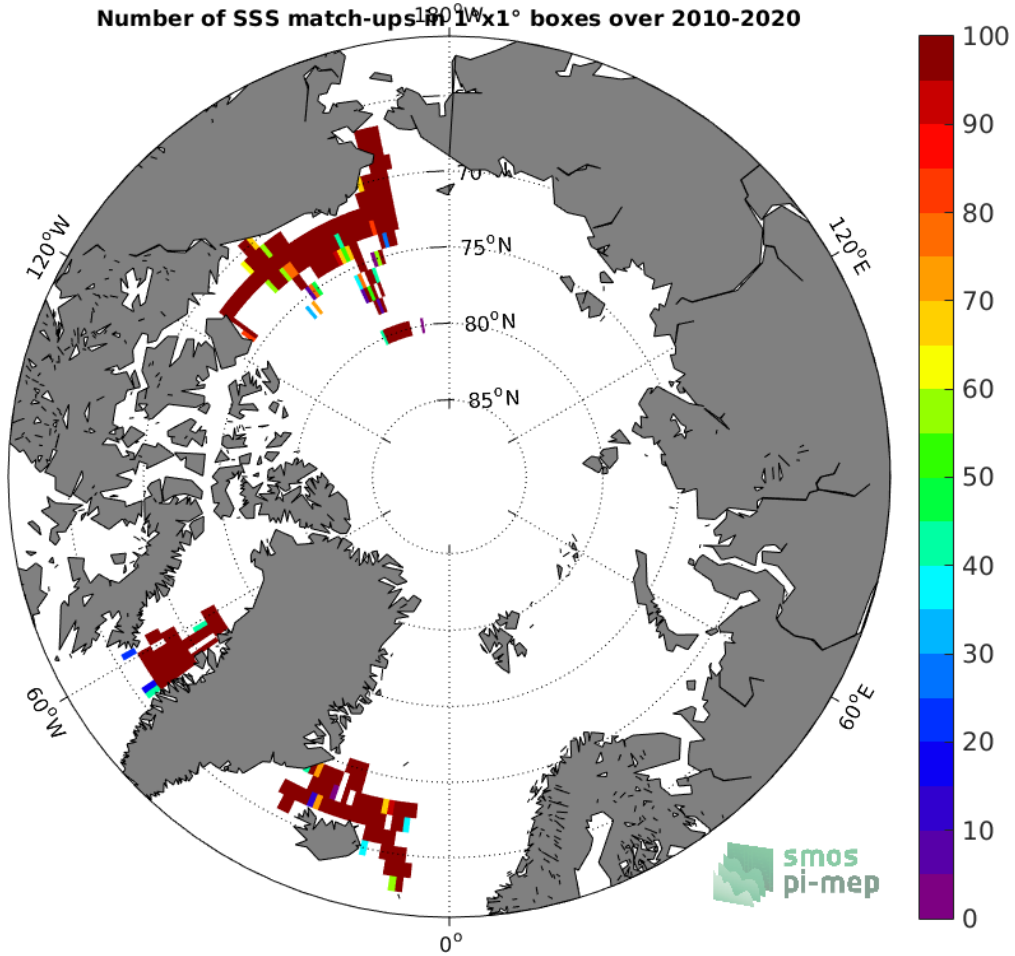
Figure 4: Number of SSS match-ups between TSG (SAMOS) SSS and the SMOS SSS L3 v7 - 9 Days (CATDS-CECOS-LOCEAN) SSS product for the Arctic Ocean Pi-MEP region over 1^\circ \times 1^\circ boxes and for the full satellite product period.
