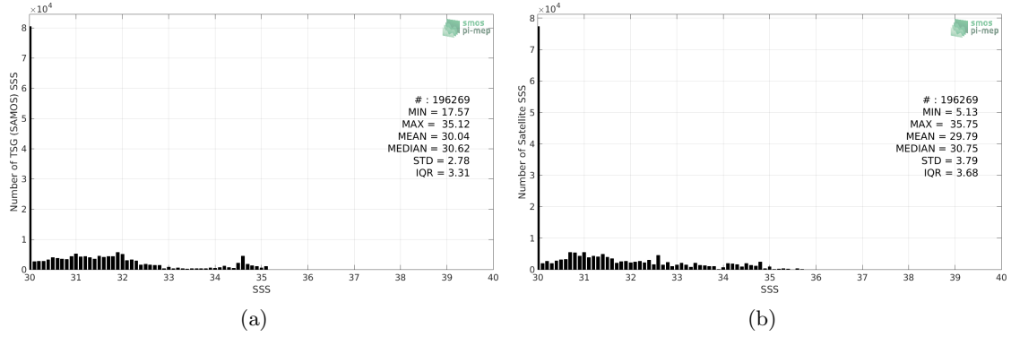
Figure 2: Histograms of SSS from TSG (SAMOS) (a) and SMOS SSS L3 v7 - 9 Days (CATDS-CECOS-LOCEAN) (b) considering all match-up pairs per bins of 0.1 over the Arctic Ocean Pi-MEP region and for the full satellite product period.
