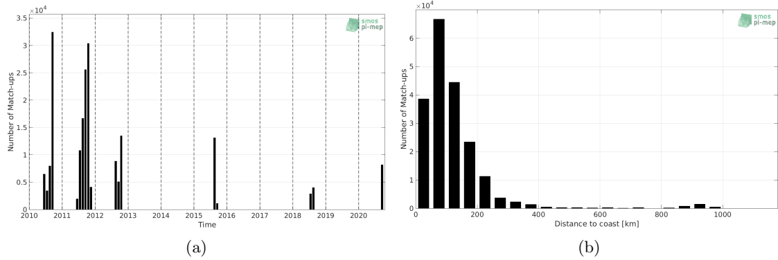
Figure 1: Number of match-ups between TSG (SAMOS) and SMOS SSS L3 v7 - 9 Days (CATDS-CECOS-LOCEAN) SSS as a function of time (a) and as function of the distance to coast (b) over the Arctic Ocean Pi-MEP region and for the full satellite product period.
