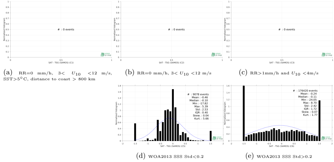
Figure 13: Normalized histogram of \Delta\text{SSS} (SMOS SSS L3 v7 - 9 Days (CATDS-CECOS-LOCEAN) - TSG (SAMOS)) for 5 different subdatasets corresponding to: RR=0 mm/h, 3 < U_{10} < 12 m/s, SST > 5^\circ\text{C} , distance to coast > 800 km (a), RR=0 mm/h, 3 < U_{10} < 12 m/s (b), RR > 1 mm/h and U_{10} < 4 m/s (c), WOA2013 SSS Std < 0.2 (d), WOA2013 SSS Std > 0.2 (e).
