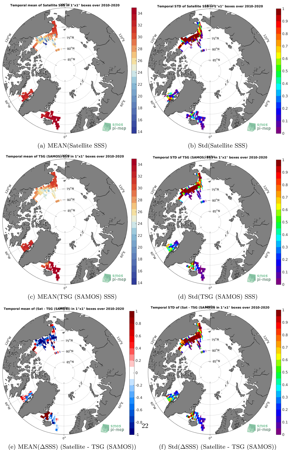
Figure 6: Temporal mean (left) and Std (right) of SSS from SMOS SSS L3 v7 - 9 Days (CATDS-CECOS-LOCEAN) (top), TSG (SAMOS) (middle), and of \Delta SSS (Satellite - TSG (SAMOS)). Only match-up pairs are used to generate these maps.
