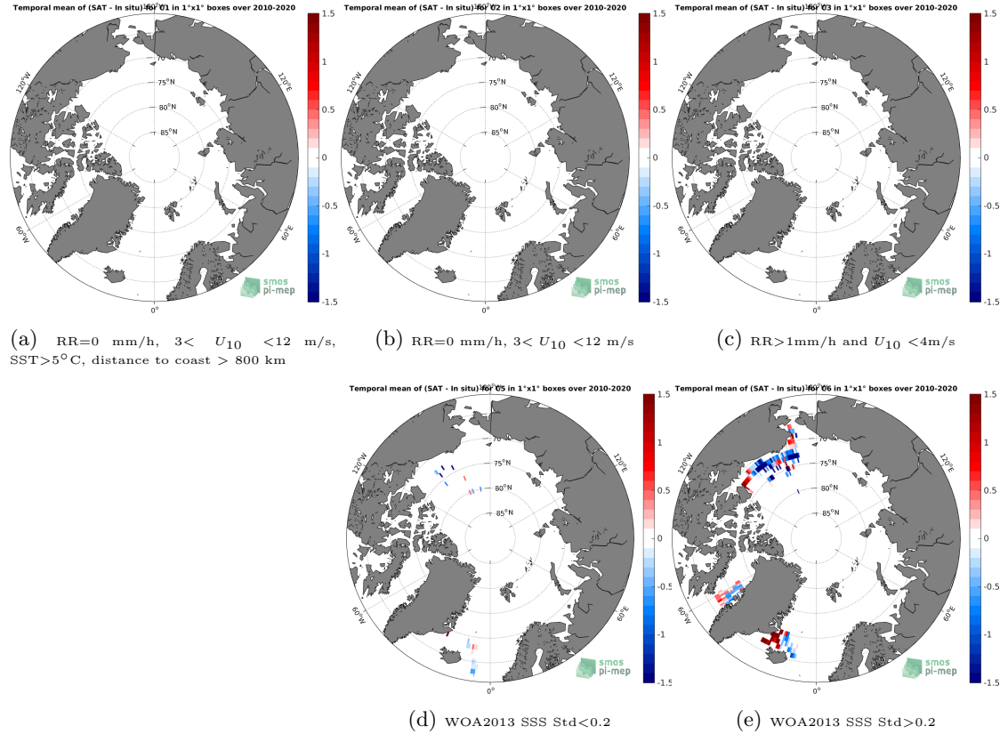
Figure 12: Temporal mean gridded over spatial boxes of size 1^{\circ} \times 1^{\circ} of \Delta\text{SSS} (SMOS SSS L3 v7 - 9 Days (CATDS-CECOS-LOCEAN) - TSG (SAMOS)) for 5 different subdatasets corresponding to: RR=0 mm/h, 3 < U_{10} < 12 m/s, SST > 5^{\circ}\text{C} , distance to coast > 800 km (a), RR=0 mm/h, 3 < U_{10} < 12 m/s (b), RR > 1 mm/h and U_{10} < 4 m/s (c), WOA2013 SSS Std < 0.2 (d), WOA2013 SSS Std > 0.2 (e).
