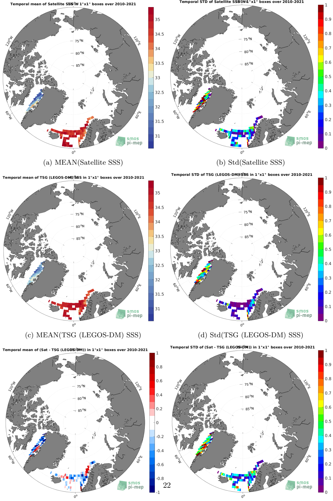
(e) MEAN( \Delta SSS) (Satellite - TSG (LEGOS-DM)) (f) Std( \Delta SSS) (Satellite - TSG (LEGOS-DM)) Figure 6: Temporal mean (left) and Std (right) of SSS from SMOS SSS L3 v7 - 9 Days (CATDS-CECOS-LOCEAN) (top), TSG (LEGOS-DM) (middle), and of \Delta SSS (Satellite - TSG (LEGOS-DM)). Only match-up pairs are used to generate these maps.
