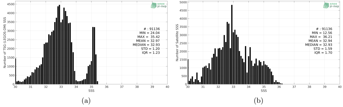
Figure 2: Histograms of SSS from TSG (LEGOS-DM) (a) and SMOS SSS L3 v7 - 9 Days (CATDS-CECOS-LOCEAN) (b) considering all match-up pairs per bins of 0.1 over the Arctic Ocean Pi-MEP region and for the full satellite product period.
