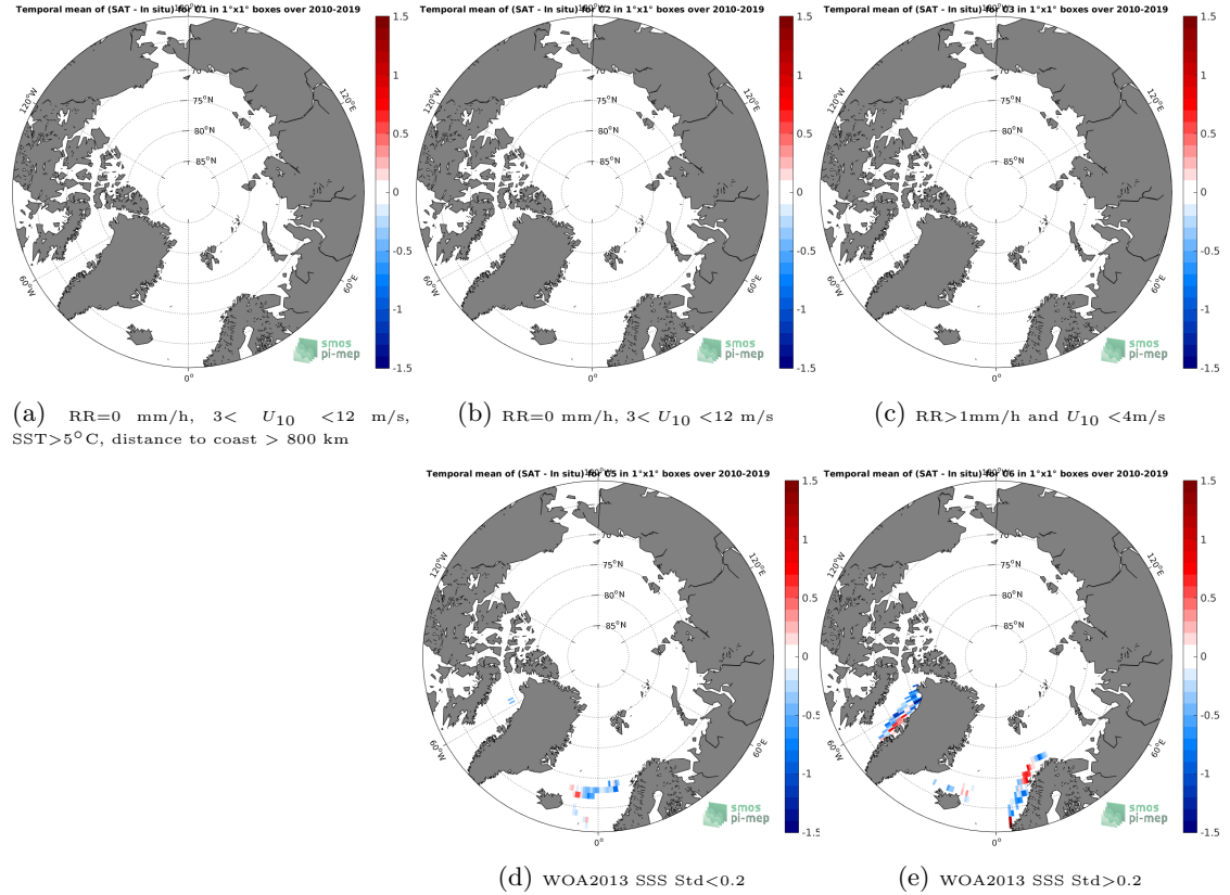
Figure 12: Temporal mean gridded over spatial boxes of size 1^{\circ} \times 1^{\circ} of \Delta\text{SSS} (SMOS SSS L3 v7 - 9 Days (CATDS-CECOS-LOCEAN) - TSG (LEGOS-DM)) for 5 different subdatasets corresponding to: \text{RR}=0 mm/h, 3 < U_{10} < 12 m/s, \text{SST} > 5^{\circ}\text{C} , distance to coast > 800 km (a), \text{RR}=0 mm/h, 3 < U_{10} < 12 m/s (b), \text{RR} > 1 mm/h and U_{10} < 4 m/s (c), WOA2013 SSS Std < 0.2 (d), WOA2013 SSS Std > 0.2 (e).
