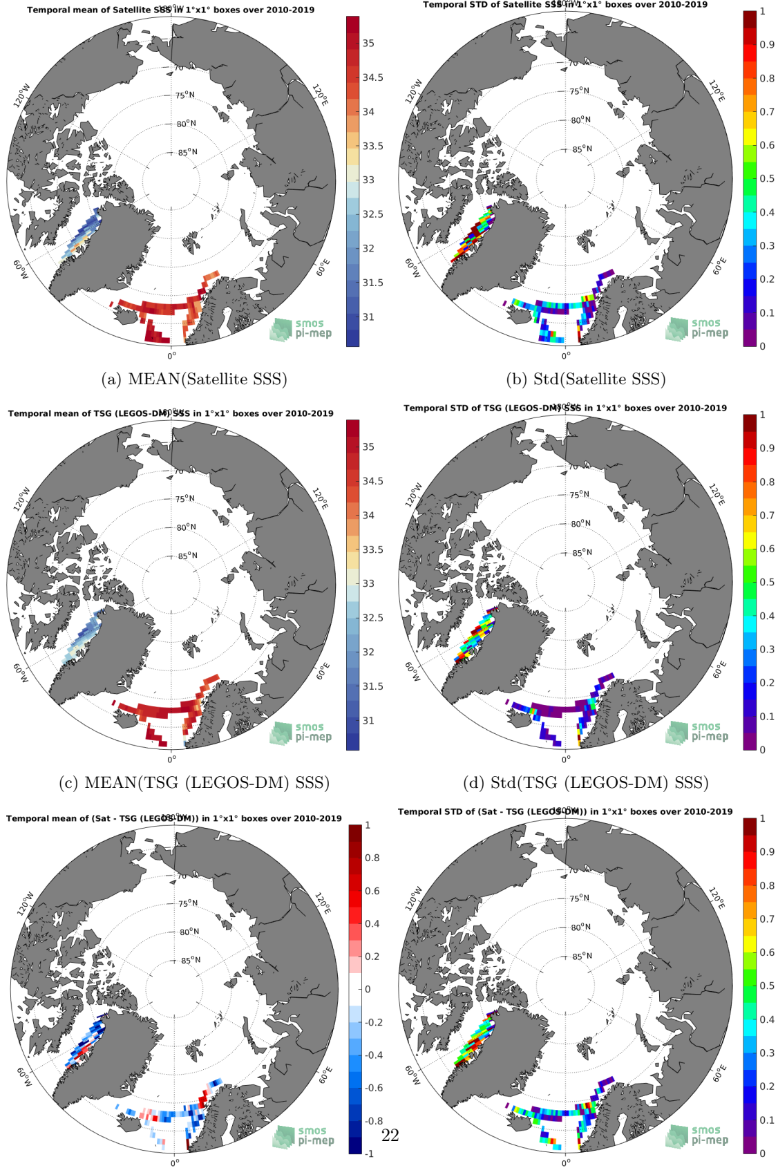
Figure 6: Temporal mean (left) and Std (right) of SSS from SMOS SSS L3 v7 - 9 Days (CATDS-CECOS-LOCEAN) (top), TSG (LEGOS-DM) (middle), and of \Delta SSS (Satellite - TSG (LEGOS-DM)). Only match-up pairs are used to generate these maps.
