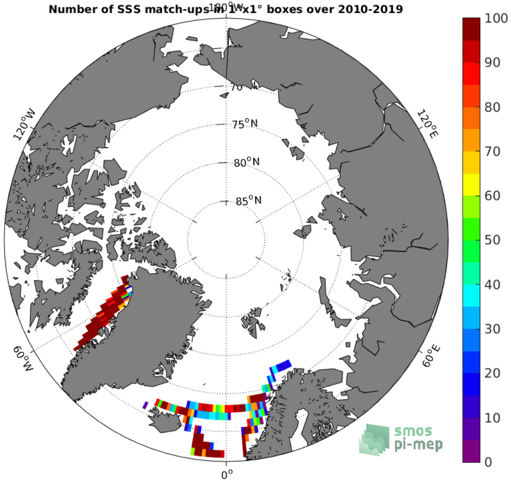
Figure 4: Number of SSS match-ups between TSG (LEGOS-DM) SSS and the SMOS SSS L3 v7 - 9 Days (CATDS-CECOS-LOCEAN) SSS product for the Arctic Ocean Pi-MEP region over 1^\circ \times 1^\circ boxes and for the full satellite product period.
