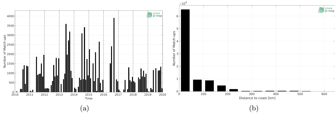
Figure 1: Number of match-ups between TSG (LEGOS-DM) and SMOS SSS L3 v7 - 9 Days (CATDS-CECOS-LOCEAN) SSS as a function of time (a) and as function of the distance to coast (b) over the Arctic Ocean Pi-MEP region and for the full satellite product period.
