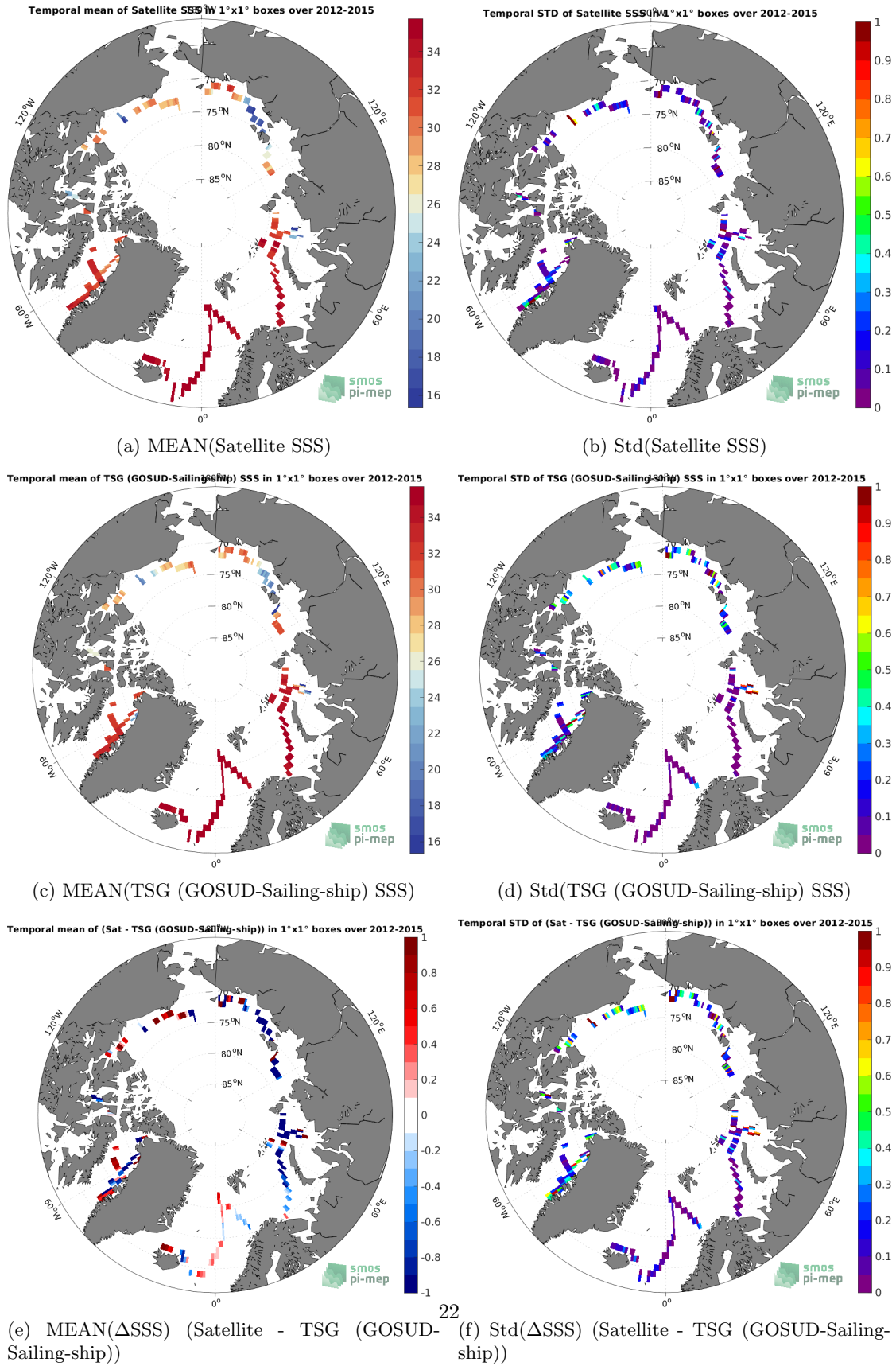
Figure 6: Temporal mean (left) and Std (right) of SSS from SMOS SSS L3 v7 - 9 Days (CATDS-CECOS-LOCEAN) (top), TSG (GOSUD-Sailing-ship) (middle), and of \Delta SSS (Satellite - TSG (GOSUD-Sailing-ship)). Only match-up pairs are used to generate these maps.
