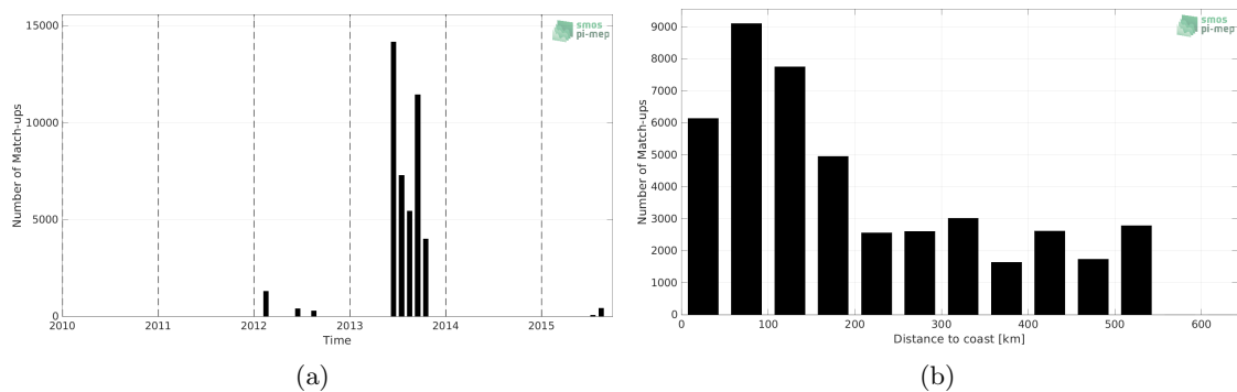
Figure 1: Number of match-ups between TSG (GOSUD-Sailing-ship) and SMOS SSS L3 v7 - 9 Days (CATDS-CECOS-LOCEAN) SSS as a function of time (a) and as function of the distance to coast (b) over the Arctic Ocean Pi-MEP region and for the full satellite product period.
