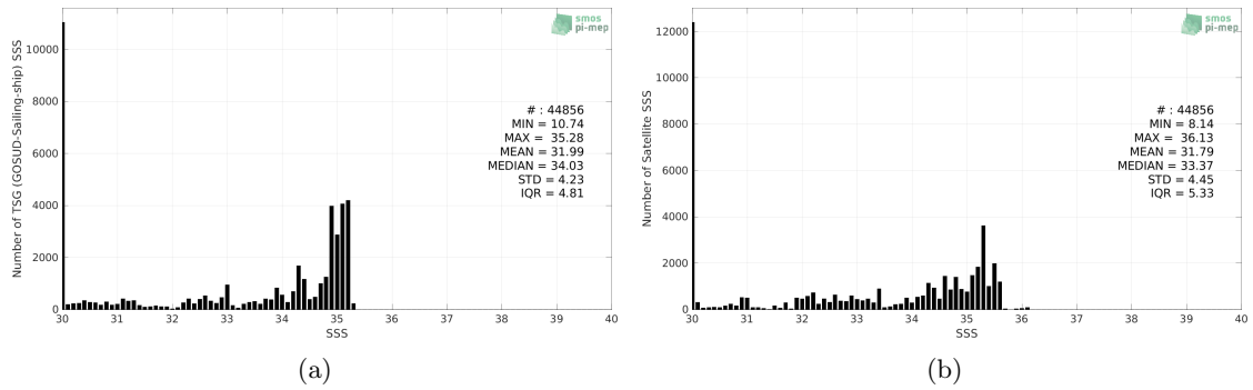
Figure 2: Histograms of SSS from TSG (GOSUD-Sailing-ship) (a) and SMOS SSS L3 v7 - 9 Days (CATDS-CECOS-LOCEAN) (b) considering all match-up pairs per bins of 0.1 over the Arctic Ocean Pi-MEP region and for the full satellite product period.
