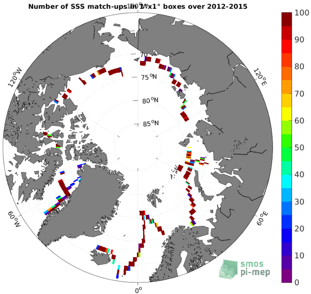
Figure 4: Number of SSS match-ups between TSG (GOSUD-Sailing-ship) SSS and the SMOS SSS L3 v7 - 9 Days (CATDS-CECOS-LOCEAN) SSS product for the Arctic Ocean Pi-MEP region over 1^\circ \times 1^\circ boxes and for the full satellite product period.
