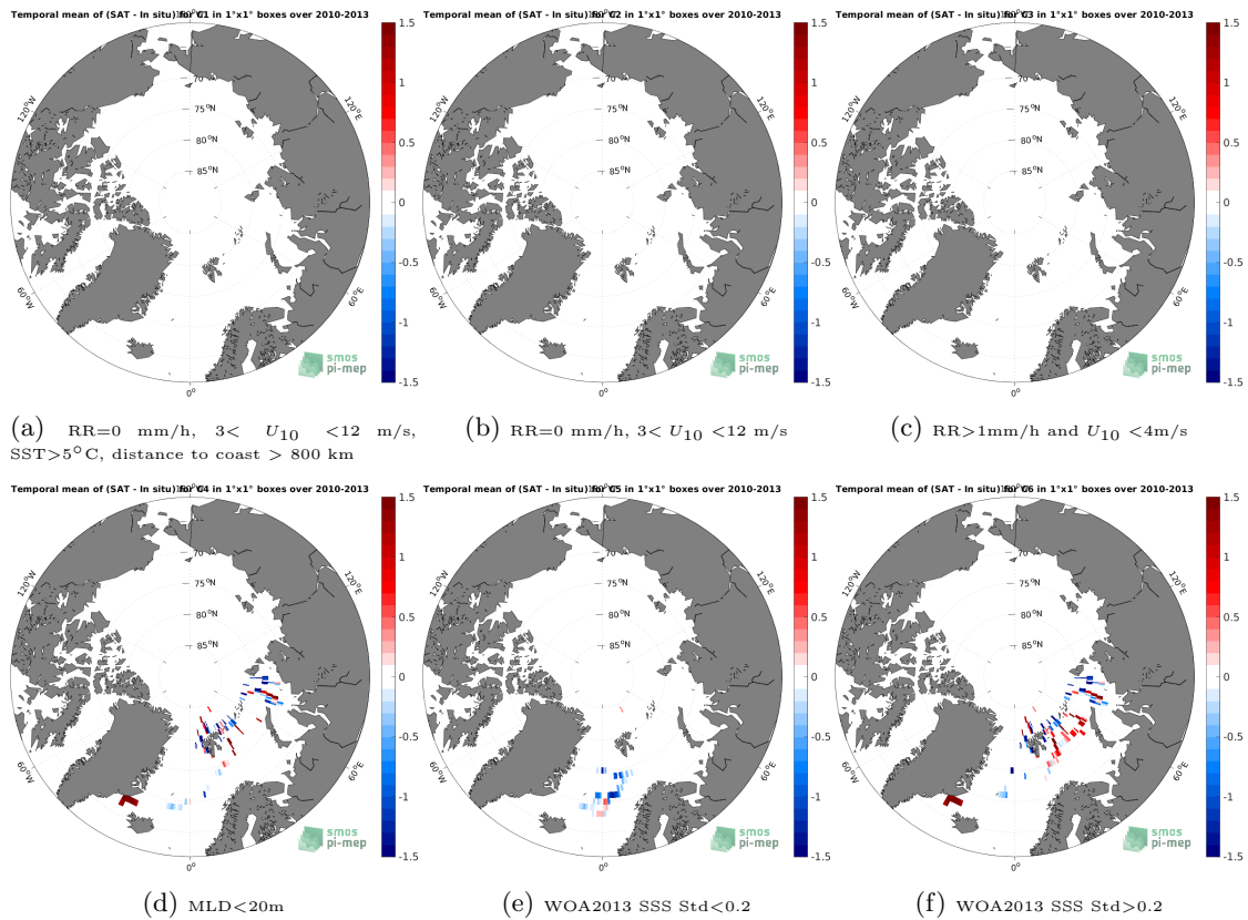
Figure 12: Temporal mean gridded over spatial boxes of size 1^{\circ}\times 1^{\circ} of \Delta\text{SSS} (SMOS SSS L3 v7 - 9 Days (CATDS-CECOS-LOCEAN) - Marine mammals) for 6 different subdatasets corresponding to: RR=0 mm/h, 3 < U_{10} < 12 m/s, SST > 5^{\circ}\text{C} , distance to coast > 800 km (a), RR=0 mm/h, 3 < U_{10} < 12 m/s (b), RR > 1\text{mm/h} and U_{10} < 4\text{m/s} (c), MLD < 20\text{m} (d), WOA2013 SSS Std < 0.2 (e), WOA2013 SSS Std > 0.2 (f).
