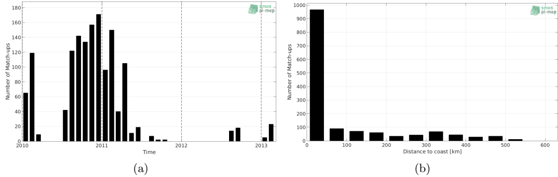
Figure 1: Number of match-ups between Marine mammals and SMOS SSS L3 v7 - 9 Days (CATDS-CECOS-LOCEAN) SSS as a function of time (a) and as function of the distance to coast (b) over the Arctic Ocean Pi-MEP region and for the full satellite product period.
