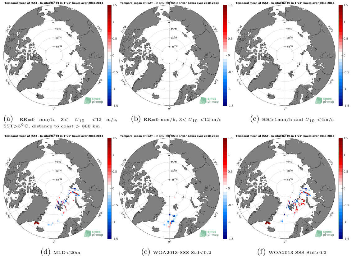
Figure 12: Temporal mean gridded over spatial boxes of size 1^{\circ} \times 1^{\circ} of \Delta\text{SSS} (SMOS SSS L3 v7 - 9 Days (CATDS-CECOS-LOCEAN) - Marine mammals) for 6 different subdatasets corresponding to: RR=0 mm/h, 3 < U_{10} < 12 m/s, SST >5^{\circ}\text{C} , distance to coast > 800 km (a), RR=0 mm/h, 3 < U_{10} < 12 m/s (b), RR >1\text{mm/h} and U_{10} < 4\text{m/s} (c), MLD <20\text{m} (d), WOA2013 SSS Std <0.2 (e), WOA2013 SSS Std >0.2 (f).
