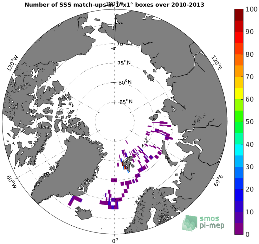
Figure 4: Number of SSS match-ups between Marine mammals SSS and the SMOS SSS L3 v7 - 9 Days (CATDS-CECOS-LOCEAN) SSS product for the Arctic Ocean Pi-MEP region over 1^\circ \times 1^\circ boxes and for the full satellite product period.
