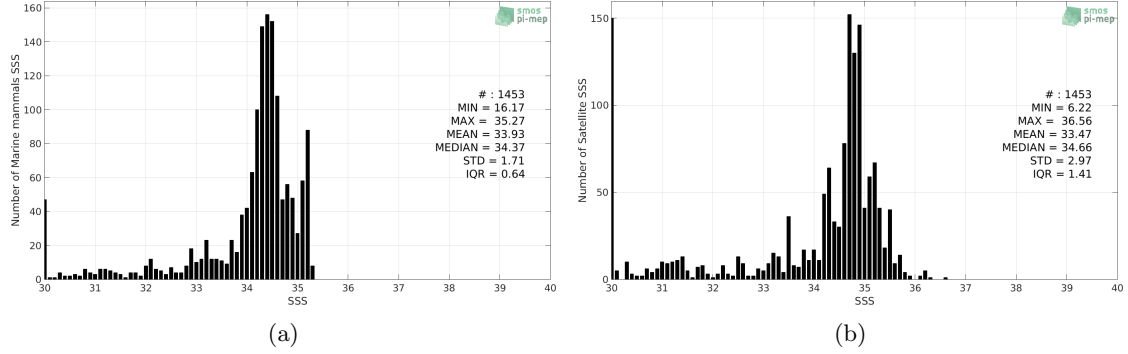
Figure 2: Histograms of SSS from Marine mammals (a) and SMOS SSS L3 v7 - 9 Days (CATDS-CECOS-LOCEAN) (b) considering all match-up pairs per bins of 0.1 over the Arctic Ocean Pi-MEP region and for the full satellite product period.
