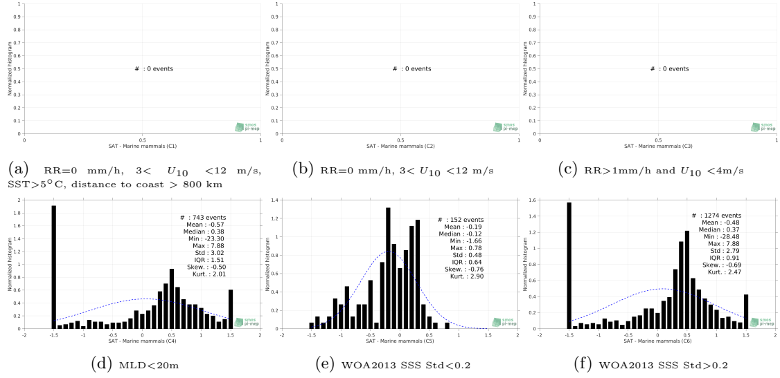
Figure 13: Normalized histogram of \Delta\text{SSS} (SMOS SSS L3 v7 - 9 Days (CATDS-CECOS-LOCEAN) - Marine mammals) for 6 different subdatasets corresponding to: RR=0 mm/h, 3 < U_{10} < 12 m/s, SST > 5^\circ\text{C} , distance to coast > 800 km (a), RR=0 mm/h, 3 < U_{10} < 12 m/s (b), RR > 1 mm/h and U_{10} < 4 m/s (c), MLD < 20 m (d), WOA2013 SSS Std < 0.2 (e), WOA2013 SSS Std > 0.2 (f).
