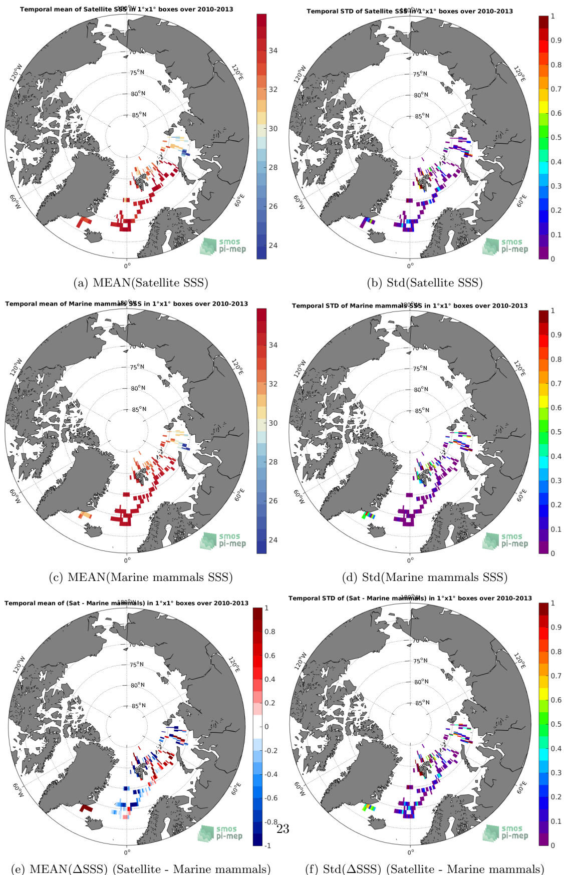
Figure 6: Temporal mean (left) and Std (right) of SSS from SMOS SSS L3 v7 - 9 Days (CATDS-CECOS-LOCEAN) (top), Marine mammals (middle), and of \Delta SSS (Satellite - Marine mammals). Only match-up pairs are used to generate these maps.
