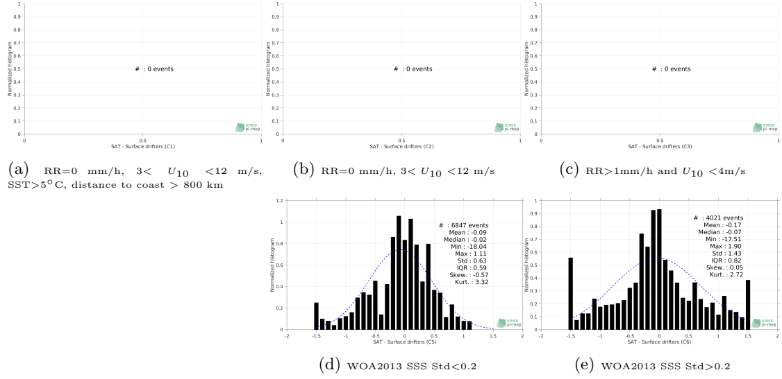
Figure 12: Normalized histogram of \Delta\text{SSS} (SMOS SSS L3 v7 - 9 Days (CATDS-CECOS-LOCEAN) - Surface drifters) for 5 different subdatasets corresponding to: RR=0 mm/h, 3 < U_{10} < 12 m/s, SST > 5^\circ\text{C} , distance to coast > 800 km (a), RR=0 mm/h, 3 < U_{10} < 12 m/s (b), RR > 1\text{mm/h} and U_{10} < 4\text{m/s} (c), WOA2013 SSS Std<0.2 (d), WOA2013 SSS Std>0.2 (e).
