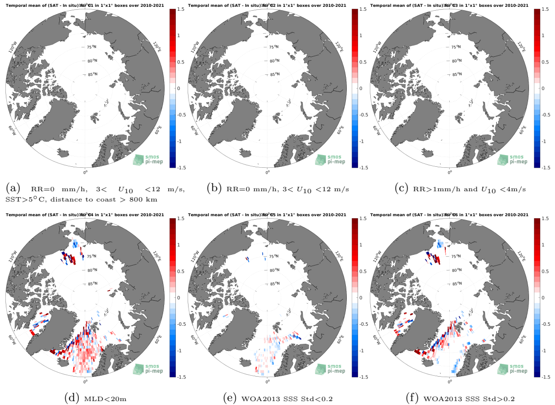
Figure 12: Temporal mean gridded over spatial boxes of size 1^{\circ}\times 1^{\circ} of \Delta\text{SSS} (SMOS SSS L3 v7 - 9 Days (CATDS-CECOS-LOCEAN) - Argo) for 6 different subdatasets corresponding to: RR=0 mm/h, 3 < U_{10} < 12 m/s, SST > 5^{\circ}\text{C} , distance to coast > 800 km (a), RR=0 mm/h, 3 < U_{10} < 12 m/s (b), RR > 1 mm/h and U_{10} < 4 m/s (c), MLD < 20\text{m} (d), WOA2013 SSS Std < 0.2 (e), WOA2013 SSS Std > 0.2 (f).
