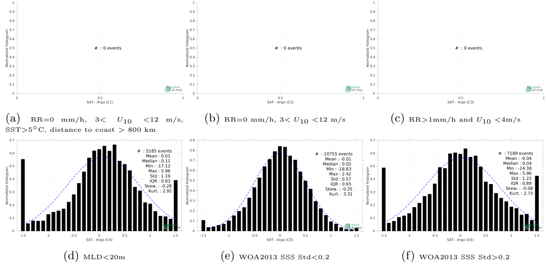
Figure 13: Normalized histogram of \Delta\text{SSS} (SMOS SSS L3 v7 - 9 Days (CATDS-CECOS-LOCEAN) - Argo) for 6 different subdatasets corresponding to: RR=0 mm/h, 3 < U_{10} < 12 m/s, SST > 5^{\circ}\text{C} , distance to coast > 800 km (a), RR=0 mm/h, 3 < U_{10} < 12 m/s (b), RR > 1\text{mm/h} and U_{10} < 4\text{m/s} (c), MLD < 20\text{m} (d), WOA2013 SSS Std < 0.2 (e), WOA2013 SSS Std > 0.2 (f).
