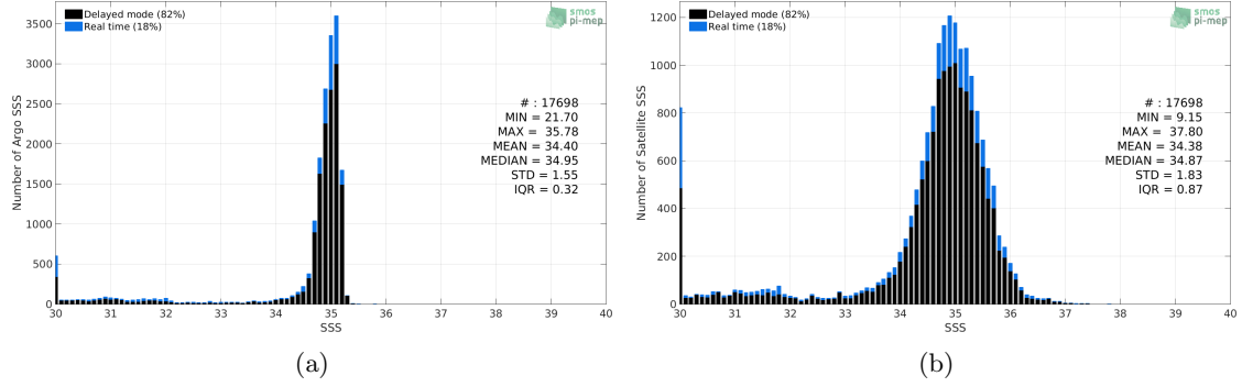
Figure 2: Histograms of SSS from Argo (a) and SMOS SSS L3 v7 - 9 Days (CATDS-CECOS-LOCEAN) (b) considering all match-up pairs per bins of 0.1 over the Arctic Ocean Pi-MEP region and for the full satellite product period.
