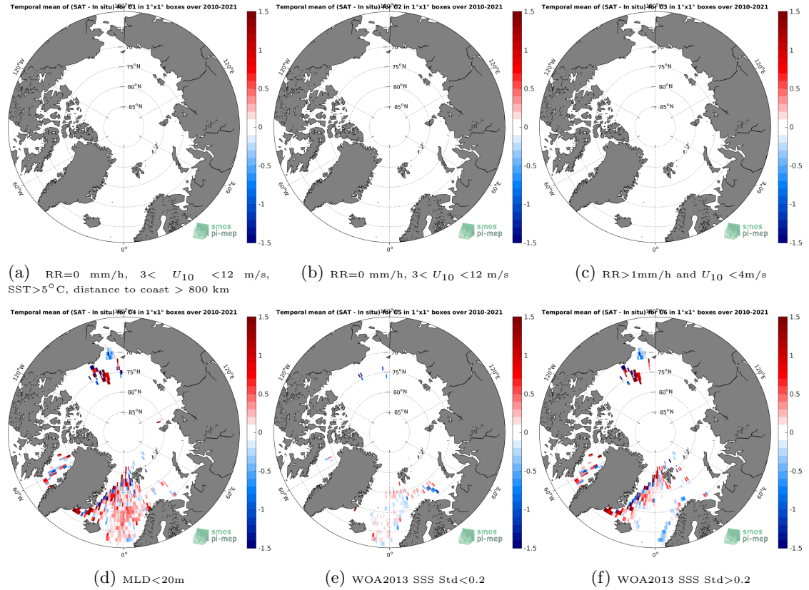
Figure 12: Temporal mean gridded over spatial boxes of size 1^{\circ} \times 1^{\circ} of \Delta\text{SSS} (SMOS SSS L3 v7 - 9 Days (CATDS-CECOS-LOCEAN) - Argo) for 6 different subdatasets corresponding to:RR=0 mm/h, 3 < U_{10} < 12 m/s, SST >5^{\circ}\text{C} , distance to coast > 800 km (a), RR=0 mm/h, 3 < U_{10} < 12 m/s (b), RR >1 mm/h and U_{10} < 4 m/s (c),MLD <20 m (d),WOA2013 SSS Std <0.2 (e),WOA2013 SSS Std >0.2 (f).
