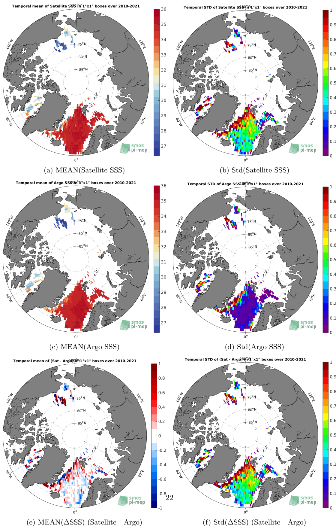
Figure 6: Temporal mean (left) and Std (right) of SSS from SMOS SSS L3 v7 - 9 Days (CATDS-CECOS-LOCEAN) (top), Argo (middle), and of \Delta SSS (Satellite - Argo). Only match-up pairs are used to generate these maps.
