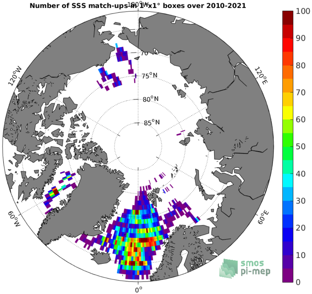
Figure 4: Number of SSS match-ups between Argo SSS and the SMOS SSS L3 v7 - 9 Days (CATDS-CECOS-LOCEAN) SSS product for the Arctic Ocean Pi-MEP region over 1^\circ \times 1^\circ boxes and for the full satellite product period.
