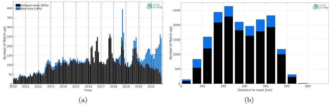
Figure 1: Number of match-ups between Argo and SMOS SSS L3 v7 - 9 Days (CATDS-CECOS-LOCEAN) SSS as a function of time (a) and as function of the distance to coast (b) over the Arctic Ocean Pi-MEP region and for the full satellite product period.
