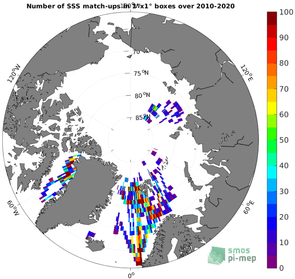
Figure 4: Number of SSS match-ups between TSG (Polarstern) SSS and the SMOS SSS L3 v7 - 18 Days (CATDS-CECOS-LOCEAN) SSS product for the Arctic Ocean Pi-MEP region over 1^\circ \times 1^\circ boxes and for the full satellite product period.
