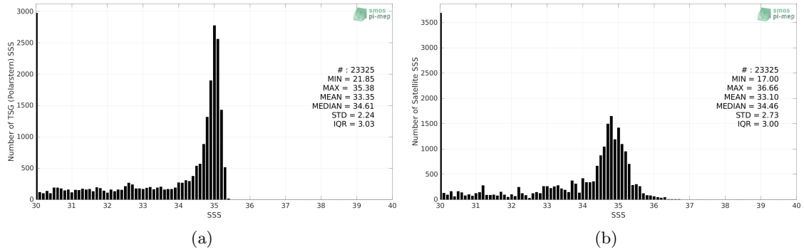
Figure 2: Histograms of SSS from TSG (Polarstern) (a) and SMOS SSS L3 v7 - 18 Days (CATDS-CECOS-LOCEAN) (b) considering all match-up pairs per bins of 0.1 over the Arctic Ocean Pi-MEP region and for the full satellite product period.
