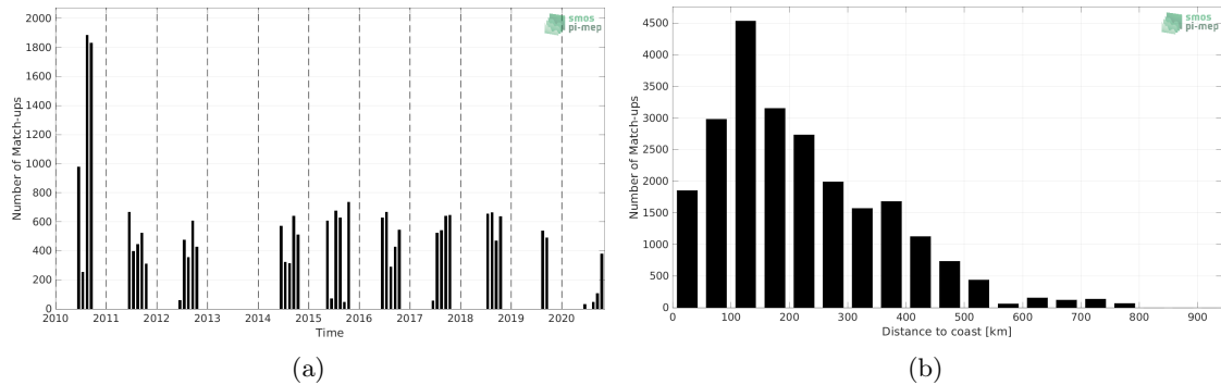
Figure 1: Number of match-ups between TSG (Polarstern) and SMOS SSS L3 v7 - 18 Days (CATDS-CECOS-LOCEAN) SSS as a function of time (a) and as function of the distance to coast (b) over the Arctic Ocean Pi-MEP region and for the full satellite product period.
