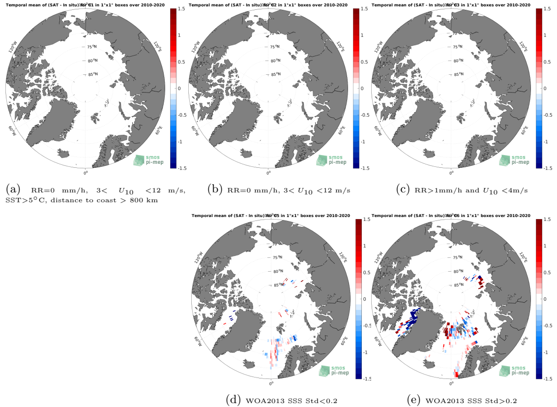
Figure 12: Temporal mean gridded over spatial boxes of size 1^{\circ}\times 1^{\circ} of \Delta\text{SSS} (SMOS SSS L3 v7 - 18 Days (CATDS-CECOS-LOCEAN) - TSG (Polarstern)) for 5 different subdatasets corresponding to:RR=0 mm/h, 3 < U_{10} < 12 m/s, SST >5^{\circ}\text{C} , distance to coast > 800 km (a), RR=0 mm/h, 3 < U_{10} < 12 m/s (b), RR >1 mm/h and U_{10} < 4 m/s (c), WOA2013 SSS Std <0.2 (d), WOA2013 SSS Std >0.2 (e).
