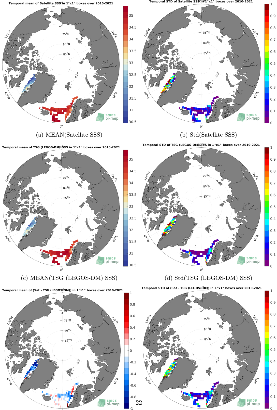
(e) MEAN( \Delta SSS) (Satellite - TSG (LEGOS-DM)) (f) Std( \Delta SSS) (Satellite - TSG (LEGOS-DM)) Figure 6: Temporal mean (left) and Std (right) of SSS from SMOS SSS L3 v7 - 18 Days (CATDS-CECOS-LOCEAN) (top), TSG (LEGOS-DM) (middle), and of \Delta SSS (Satellite - TSG (LEGOS-DM)). Only match-up pairs are used to generate these maps.
