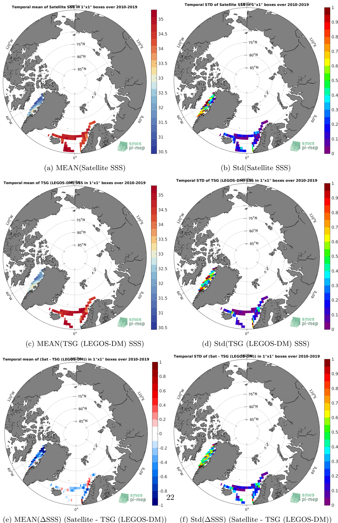
Figure 6: Temporal mean (left) and Std (right) of SSS from SMOS SSS L3 v7 - 18 Days (CATDS-CECOS-LOCEAN) (top), TSG (LEGOS-DM) (middle), and of \Delta SSS (Satellite - TSG (LEGOS-DM)). Only match-up pairs are used to generate these maps.
