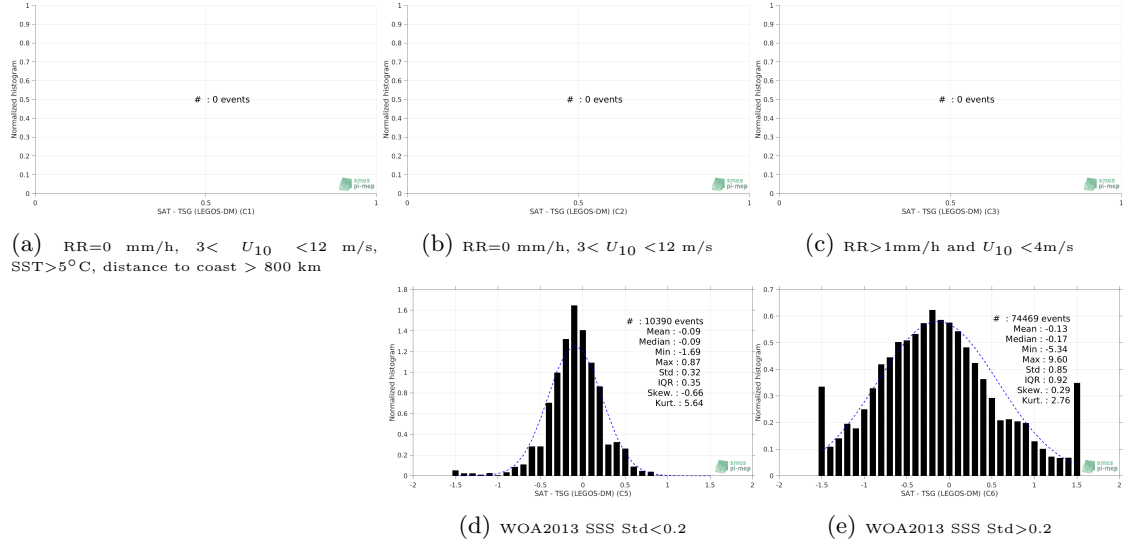
Figure 13: Normalized histogram of \Delta\text{SSS} (SMOS SSS L3 v7 - 18 Days (CATDS-CECOS-LOCEAN) - TSG (LEGOS-DM)) for 5 different subdatasets corresponding to: RR=0 mm/h, 3 < U_{10} < 12 m/s, SST > 5^\circ\text{C} , distance to coast > 800 km (a), RR=0 mm/h, 3 < U_{10} < 12 m/s (b), RR > 1\text{mm/h} and U_{10} < 4\text{m/s} (c), WOA2013 SSS Std<0.2 (d), WOA2013 SSS Std>0.2 (e).
