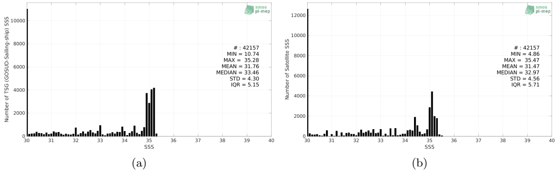
Figure 2: Histograms of SSS from TSG (GOSUD-Sailing-ship) (a) and SMOS SSS L3 v7 - 18 Days (CATDS-CECOS-LOCEAN) (b) considering all match-up pairs per bins of 0.1 over the Arctic Ocean Pi-MEP region and for the full satellite product period.
