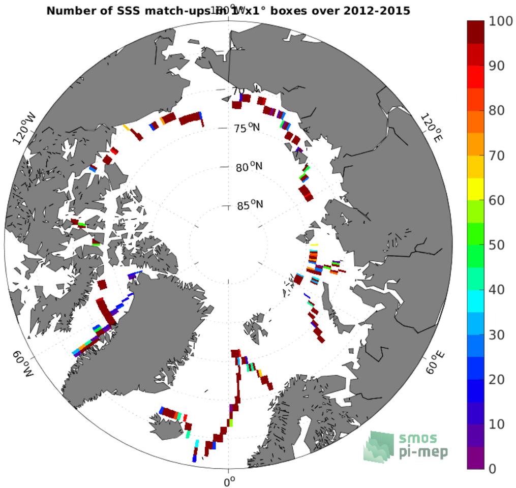
Figure 4: Number of SSS match-ups between TSG (GOSUD-Sailing-ship) SSS and the SMOS SSS L3 v7 - 18 Days (CATDS-CECOS-LOCEAN) SSS product for the Arctic Ocean Pi-MEP region over 1^{\circ} \times 1^{\circ} boxes and for the full satellite product period.
