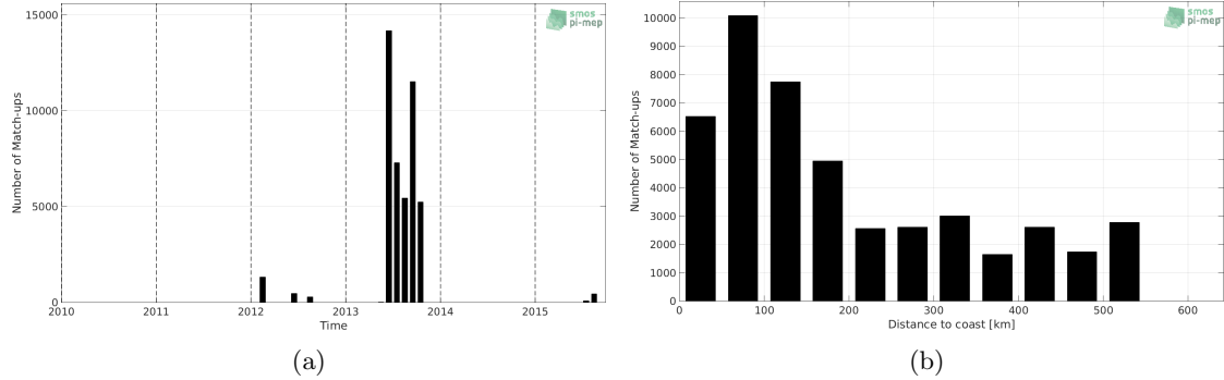
Figure 1: Number of match-ups between TSG (GOSUD-Sailing-ship) and SMOS SSS L3 v7 - 18 Days (CATDS-CECOS-LOCEAN) SSS as a function of time (a) and as function of the distance to coast (b) over the Arctic Ocean Pi-MEP region and for the full satellite product period.
