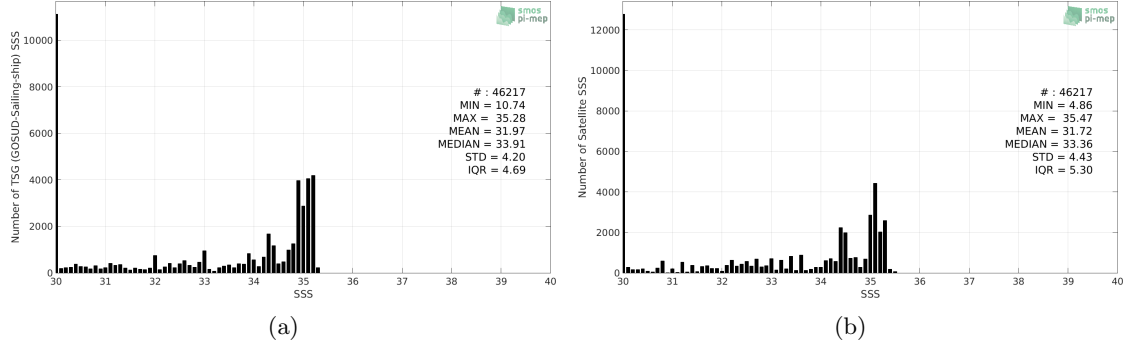
Figure 2: Histograms of SSS from TSG (GOSUD-Sailing-ship) (a) and SMOS SSS L3 v7 - 18 Days (CATDS-CECOS-LOCEAN) (b) considering all match-up pairs per bins of 0.1 over the Arctic Ocean Pi-MEP region and for the full satellite product period.
