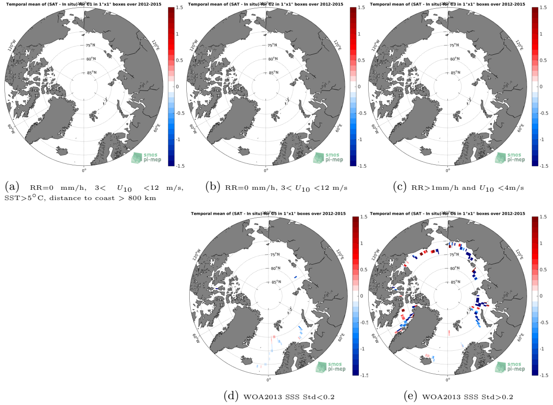
Figure 12: Temporal mean gridded over spatial boxes of size 1^\circ \times 1^\circ of \Delta SSS (SMOS SSS L3 v7 - 18 Days (CATDS-CECOS-LOCEAN) - TSG (GOSUD-Sailing-ship)) for 5 different subdatasets corresponding to: RR=0 mm/h, 3 < U_{10} < 12 m/s, SST>5°C, distance to coast > 800 km (a), RR=0 mm/h, 3 < U_{10} < 12 m/s (b), RR>1mm/h and U_{10} < 4 m/s (c), WOA2013 SSS Std<0.2 (d), WOA2013 SSS Std>0.2 (e).
