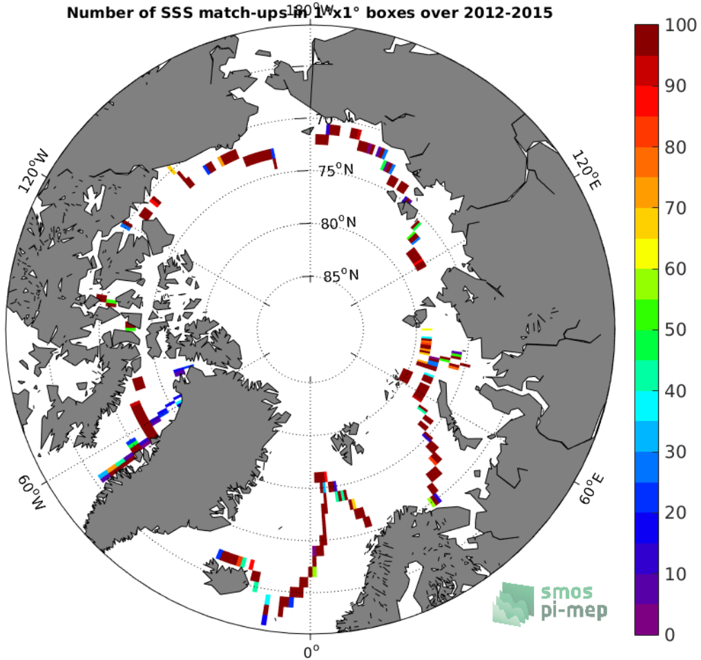
Figure 4: Number of SSS match-ups between TSG (GOSUD-Sailing-ship) SSS and the SMOS SSS L3 v7 - 18 Days (CATDS-CECOS-LOCEAN) SSS product for the Arctic Ocean Pi-MEP region over 1^\circ \times 1^\circ boxes and for the full satellite product period.
