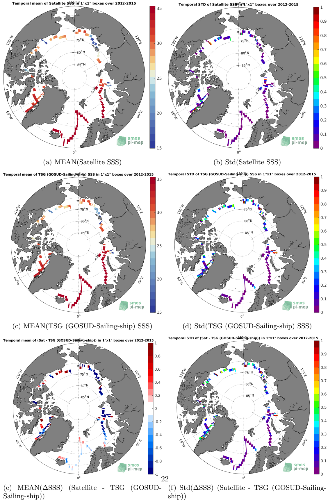
Figure 6: Temporal mean (left) and Std (right) of SSS from SMOS SSS L3 v7 - 18 Days (CATDS-CECOS-LOCEAN) (top), TSG (GOSUD-Sailing-ship) (middle), and of \Delta SSS (Satellite - TSG (GOSUD-Sailing-ship)). Only match-up pairs are used to generate these maps.
