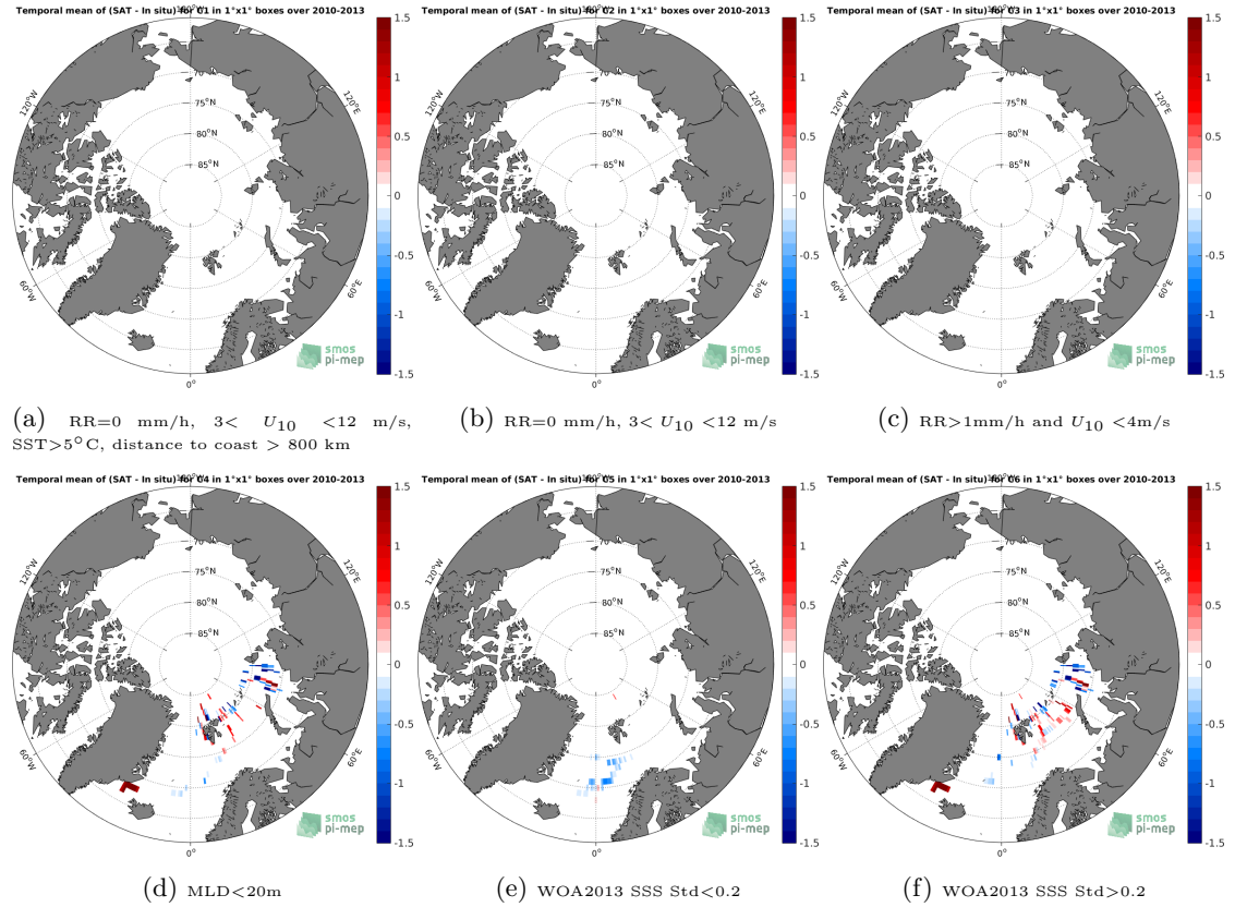
Figure 12: Temporal mean gridded over spatial boxes of size 1^{\circ} \times 1^{\circ} of \Delta\text{SSS} (SMOS SSS L3 v7 - 18 Days (CATDS-CECOS-LOCEAN) - Marine mammals) for 6 different subdatasets corresponding to:RR=0 mm/h, 3 < U_{10} < 12 m/s, SST >5^{\circ}\text{C} , distance to coast > 800 km (a), RR=0 mm/h, 3 < U_{10} < 12 m/s (b), RR >1 mm/h and U_{10} < 4 m/s (c),MLD <20 m (d),WOA2013 SSS Std <0.2 (e),WOA2013 SSS Std >0.2 (f).
