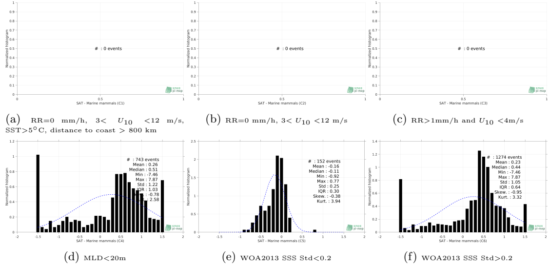
Figure 13: Normalized histogram of \Delta\text{SSS} (SMOS SSS L3 v7 - 18 Days (CATDS-CECOS-LOCEAN) - Marine mammals) for 6 different subdatasets corresponding to: RR=0 mm/h, 3 < U_{10} < 12 m/s, SST > 5^{\circ}\text{C} , distance to coast > 800 km (a), RR=0 mm/h, 3 < U_{10} < 12 m/s (b), RR > 1\text{mm/h} and U_{10} < 4\text{m/s} (c), MLD < 20\text{m} (d), WOA2013 SSS Std < 0.2 (e), WOA2013 SSS Std > 0.2 (f).
