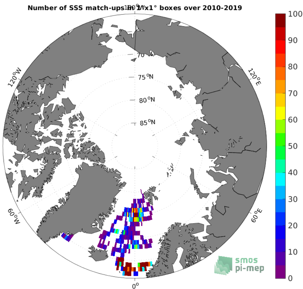
Figure 3: Number of SSS match-ups between Surface drifters SSS and the SMOS SSS L3 v7 - 18 Days (CATDS-CECOS-LOCEAN) SSS product for the Arctic Ocean Pi-MEP region over 1^{\circ} \times 1^{\circ} boxes and for the full satellite product period.
