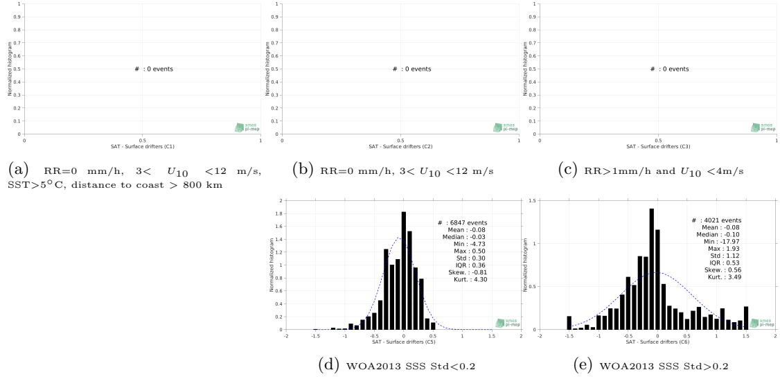
Figure 12: Normalized histogram of \Delta\text{SSS} (SMOS SSS L3 v7 - 18 Days (CATDS-CECOS-LOCEAN) - Surface drifters) for 5 different subdatasets corresponding to: RR=0 mm/h, 3 < U_{10} < 12 m/s, SST > 5^\circ\text{C} , distance to coast > 800 km (a), RR=0 mm/h, 3 < U_{10} < 12 m/s (b), RR > 1\text{mm/h} and U_{10} < 4\text{m/s} (c), WOA2013 SSS Std<0.2 (d), WOA2013 SSS Std>0.2 (e).
