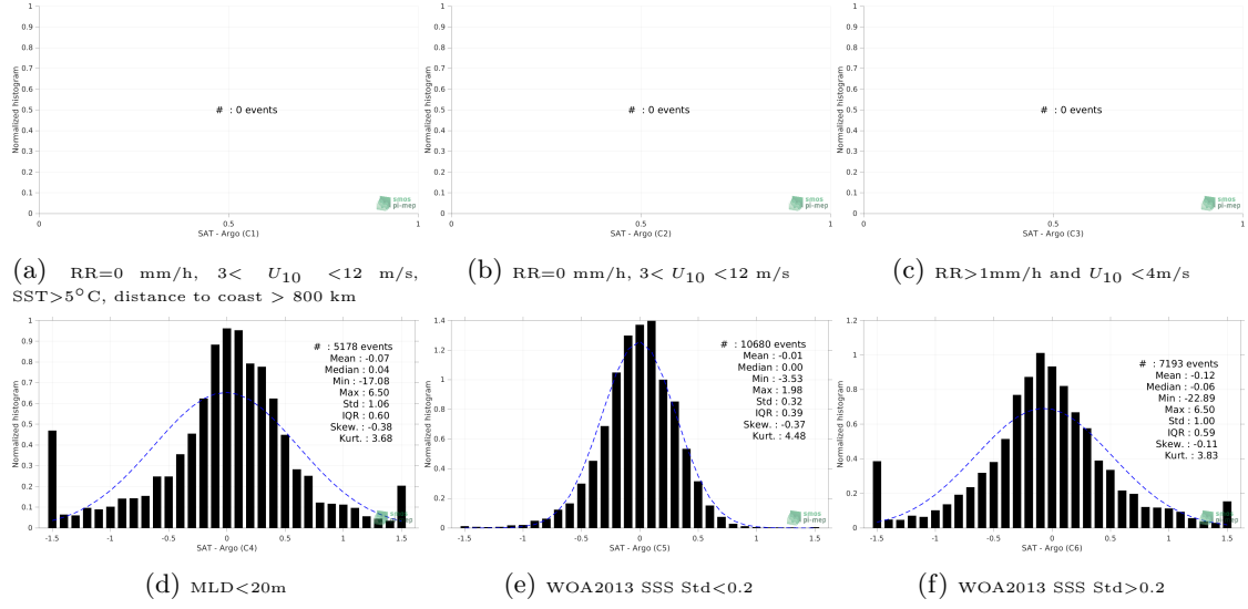
Figure 13: Normalized histogram of \Delta\text{SSS} (SMOS SSS L3 v7 - 18 Days (CATDS-CECOS-LOCEAN) - Argo) for 6 different subdatasets corresponding to: RR=0 mm/h, 3 < U_{10} < 12 m/s, SST > 5^{\circ}\text{C} , distance to coast > 800 km (a), RR=0 mm/h, 3 < U_{10} < 12 m/s (b), RR > 1\text{mm/h} and U_{10} < 4\text{m/s} (c), MLD < 20\text{m} (d), WOA2013 SSS Std < 0.2 (e), WOA2013 SSS Std > 0.2 (f).
