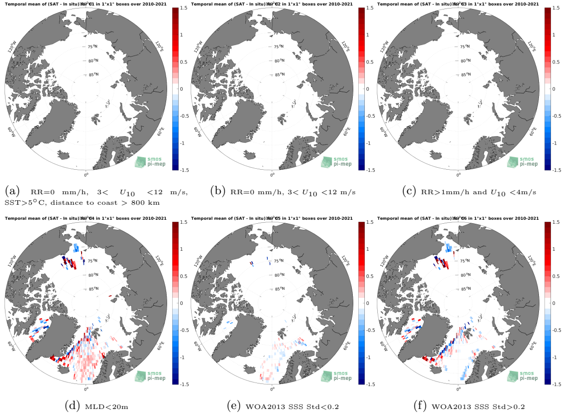
Figure 12: Temporal mean gridded over spatial boxes of size 1^{\circ}\times 1^{\circ} of \Delta\text{SSS} (SMOS SSS L3 v7 - 18 Days (CATDS-CECOS-LOCEAN) - Argo) for 6 different subdatasets corresponding to: RR=0 mm/h, 3 < U_{10} < 12 m/s, SST > 5^{\circ}\text{C} , distance to coast > 800 km (a), RR=0 mm/h, 3 < U_{10} < 12 m/s (b), RR > 1\text{mm/h} and U_{10} < 4\text{m/s} (c), MLD < 20\text{m} (d), WOA2013 SSS Std < 0.2 (e), WOA2013 SSS Std > 0.2 (f).
