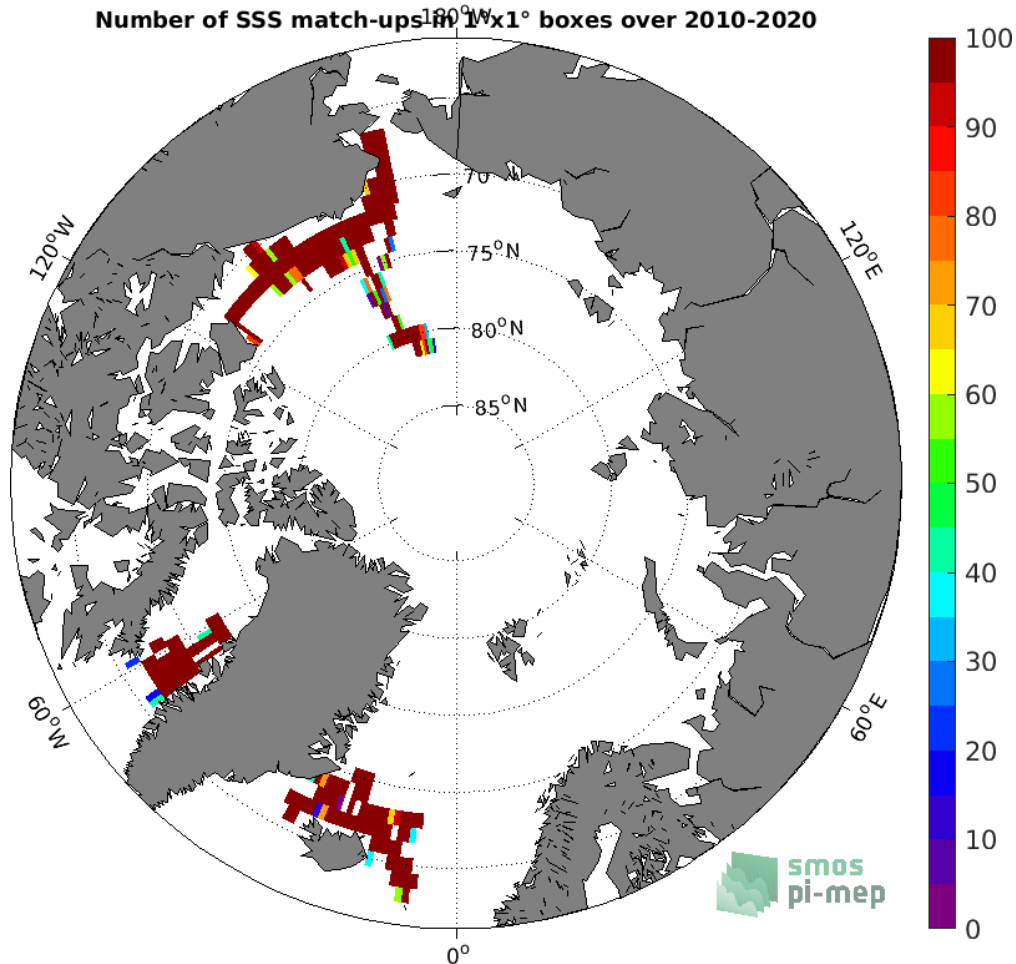
Figure 4: Number of SSS match-ups between TSG (SAMOS) SSS and the SMOS SSS L3 v5 - 9 Days (CATDS-CECOS-LOCEAN) SSS product for the Arctic Ocean Pi-MEP region over 1^\circ \times 1^\circ boxes and for the full satellite product period.
