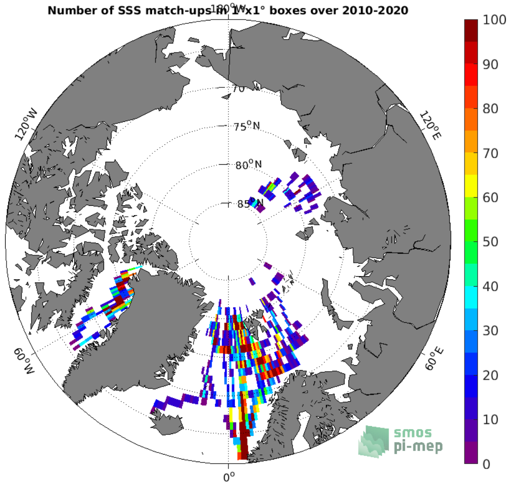
Figure 4: Number of SSS match-ups between TSG (Polarstern) SSS and the SMOS SSS L3 v5 - 9 Days (CATDS-CECOS-LOCEAN) SSS product for the Arctic Ocean Pi-MEP region over 1^\circ \times 1^\circ boxes and for the full satellite product period.
