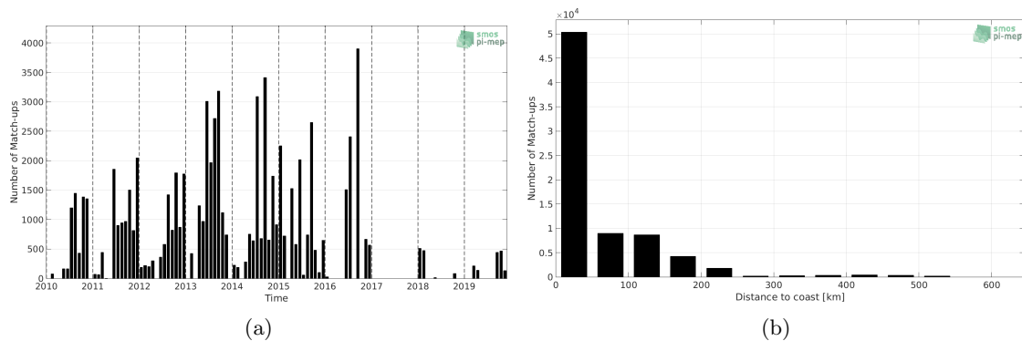
Figure 1: Number of match-ups between TSG (LEGOS-DM) and SMOS SSS L3 v5 - 9 Days (CATDS-CECOS-LOCEAN) SSS as a function of time (a) and as function of the distance to coast (b) over the Arctic Ocean Pi-MEP region and for the full satellite product period.
