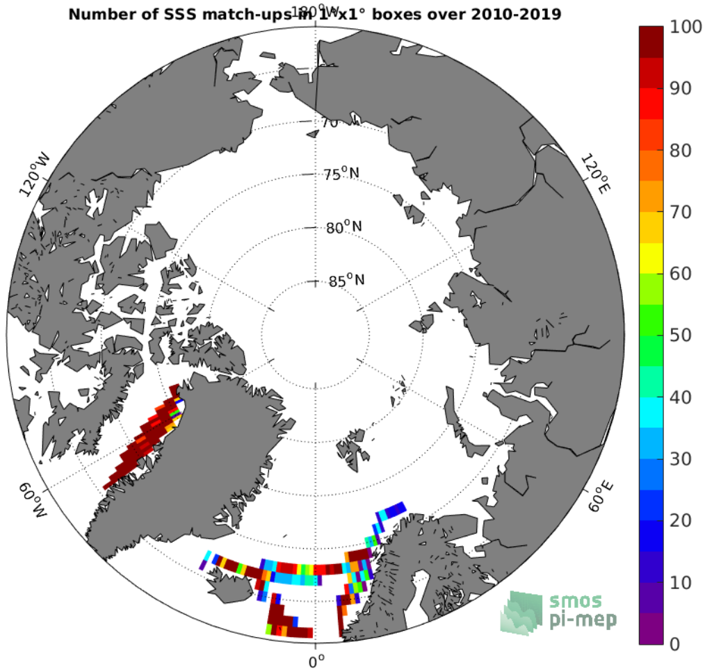
Figure 4: Number of SSS match-ups between TSG (LEGOS-DM) SSS and the SMOS SSS L3 v5 - 9 Days (CATDS-CECOS-LOCEAN) SSS product for the Arctic Ocean Pi-MEP region over 1^\circ \times 1^\circ boxes and for the full satellite product period.
