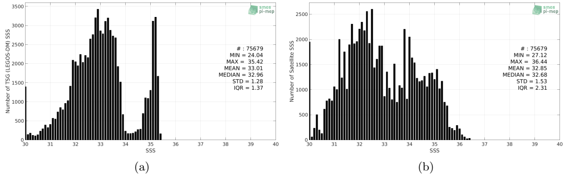
Figure 2: Histograms of SSS from TSG (LEGOS-DM) (a) and SMOS SSS L3 v5 - 9 Days (CATDS-CECOS-LOCEAN) (b) considering all match-up pairs per bins of 0.1 over the Arctic Ocean Pi-MEP region and for the full satellite product period.
