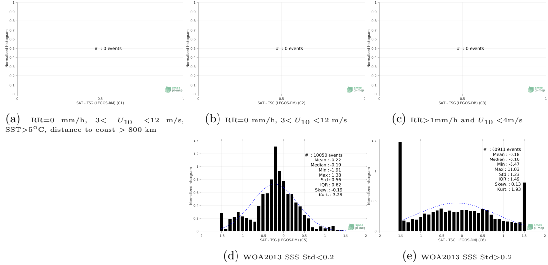
Figure 13: Normalized histogram of \Delta SSS (SMOS SSS L3 v5 - 9 Days (CATDS-CECOS-LOCEAN) - TSG (LEGOS-DM)) for 5 different subdatasets corresponding to: RR=0 mm/h, 3 < U_{10} < 12 m/s, SST > 5°C, distance to coast > 800 km (a), RR=0 mm/h, 3 < U_{10} < 12 m/s (b), RR > 1mm/h and U_{10} < 4 m/s (c), WOA2013 SSS Std < 0.2 (d), WOA2013 SSS Std > 0.2 (e).
