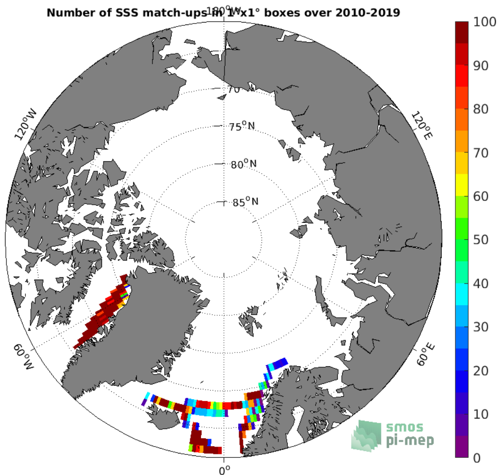
Figure 4: Number of SSS match-ups between TSG (LEGOS-DM) SSS and the SMOS SSS L3 v5 - 9 Days (CATDS-CECOS-LOCEAN) SSS product for the Arctic Ocean Pi-MEP region over 1°x1° boxes and for the full satellite product period.
