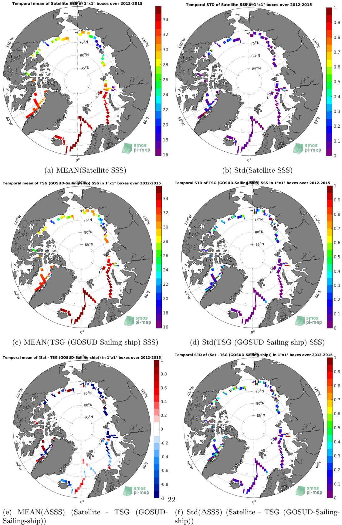
Figure 6: Temporal mean (left) and Std (right) of SSS from SMOS SSS L3 v5 - 9 Days (CATDS-CECOS-LOCEAN) (top), TSG (GOSUD-Sailing-ship) (middle), and of \Delta SSS (Satellite - TSG (GOSUD-Sailing-ship)). Only match-up pairs are used to generate these maps.
