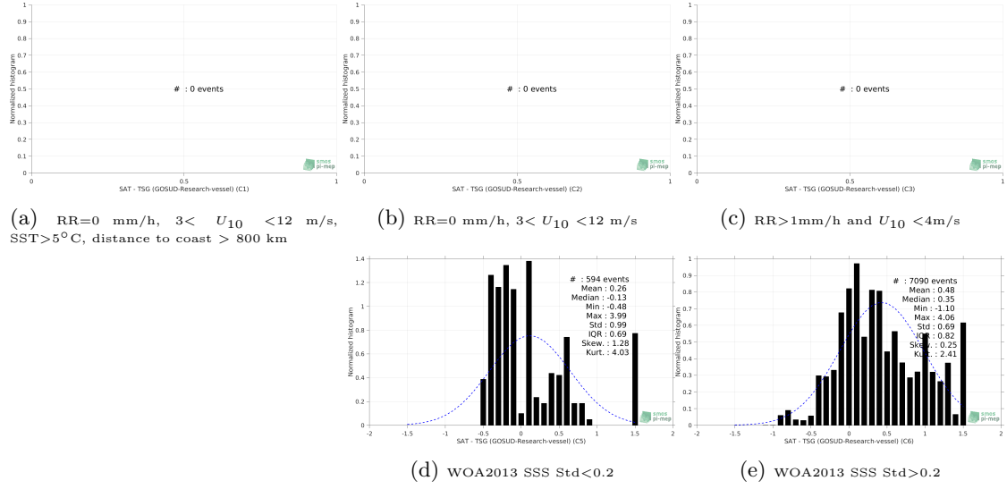
Figure 13: Normalized histogram of \Delta\text{SSS} (SMOS SSS L3 v5 - 9 Days (CATDS-CECOS-LOCEAN) - TSG (GOSUD-Research-vessel)) for 5 different subdatasets corresponding to: RR=0 mm/h, 3 < U_{10} < 12 m/s, SST > 5^\circ\text{C} , distance to coast > 800 km (a), RR=0 mm/h, 3 < U_{10} < 12 m/s (b), RR > 1\text{mm/h} and U_{10} < 4\text{m/s} (c), WOA2013 SSS Std < 0.2 (d), WOA2013 SSS Std > 0.2 (e).
