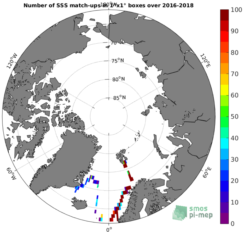
Figure 4: Number of SSS match-ups between TSG (GOSUD-Research-vessel) SSS and the SMOS SSS L3 v5 - 9 Days (CATDS-CECOS-LOCEAN) SSS product for the Arctic Ocean Pi-MEP region over 1^\circ \times 1^\circ boxes and for the full satellite product period.
