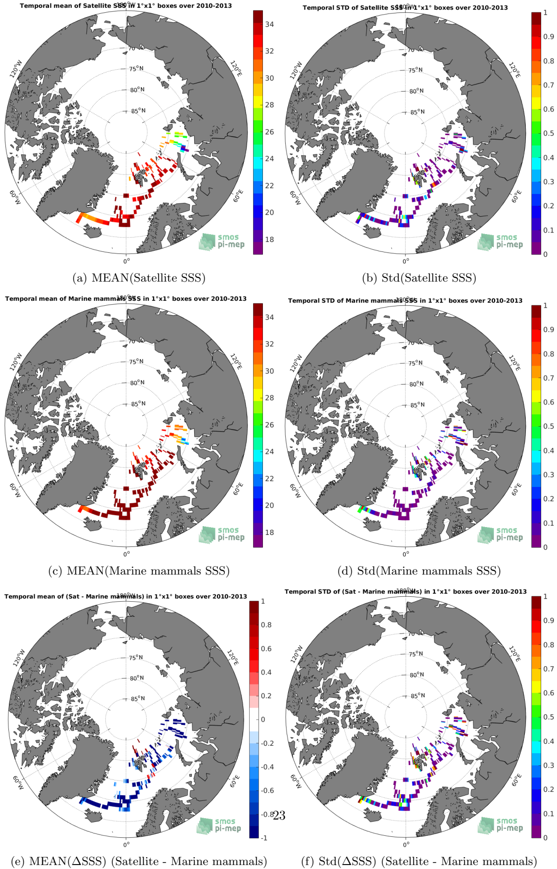
Figure 6: Temporal mean (left) and Std (right) of SSS from SMOS SSS L3 v5 - 9 Days (CATDS-CECOS-LOCEAN) (top), Marine mammals (middle), and of \Delta SSS (Satellite - Marine mammals). Only match-up pairs are used to generate these maps.
