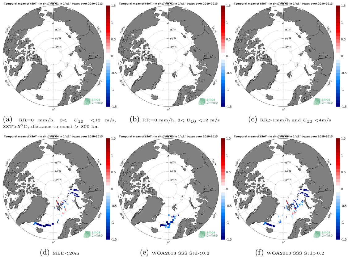
Figure 12: Temporal mean gridded over spatial boxes of size 1^{\circ}\times 1^{\circ} of \Delta\text{SSS} (SMOS SSS L3 v5 - 9 Days (CATDS-CECOS-LOCEAN) - Marine mammals) for 6 different subdatasets corresponding to:RR=0 mm/h, 3 < U_{10} < 12 m/s, SST >5^{\circ}\text{C} , distance to coast > 800 km (a), RR=0 mm/h, 3 < U_{10} < 12 m/s (b), RR >1 mm/h and U_{10} < 4 m/s (c),MLD <20 m (d),WOA2013 SSS Std <0.2 (e),WOA2013 SSS Std >0.2 (f).
