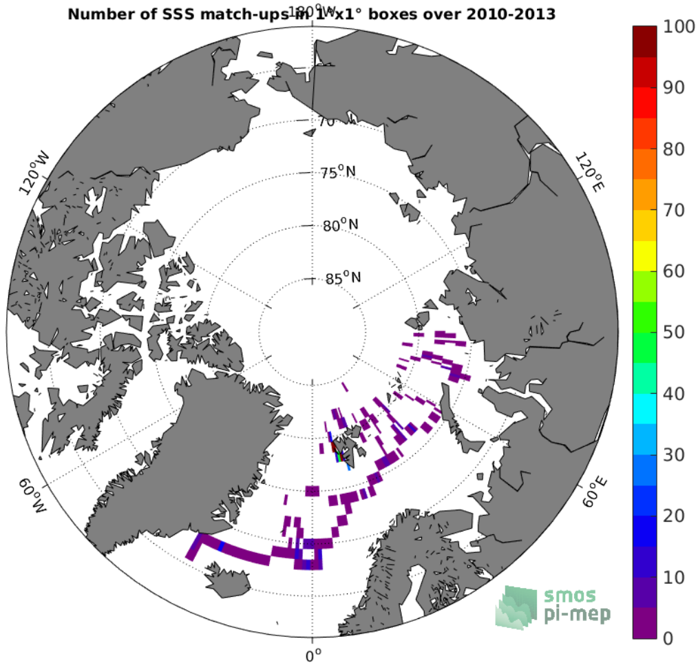
Figure 4: Number of SSS match-ups between Marine mammals SSS and the SMOS SSS L3 v5 - 9 Days (CATDS-CECOS-LOCEAN) SSS product for the Arctic Ocean Pi-MEP region over 1^\circ \times 1^\circ boxes and for the full satellite product period.
