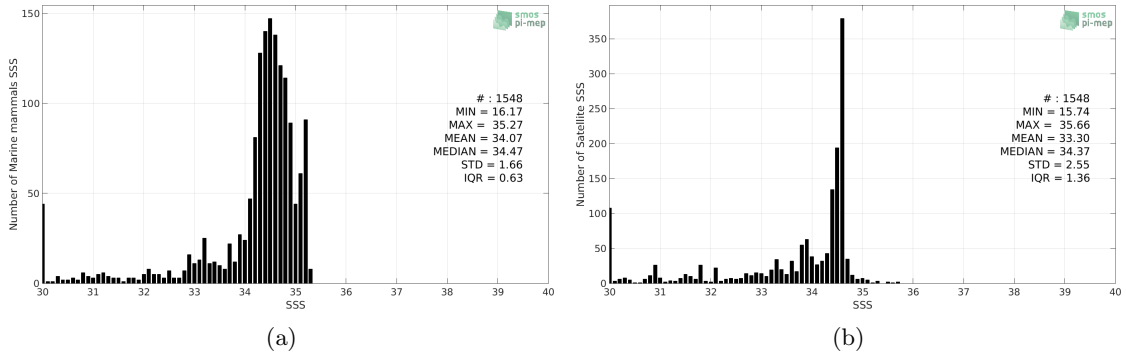
Figure 2: Histograms of SSS from Marine mammals (a) and SMOS SSS L3 v5 - 9 Days (CATDS-CECOS-LOCEAN) (b) considering all match-up pairs per bins of 0.1 over the Arctic Ocean Pi-MEP region and for the full satellite product period.
