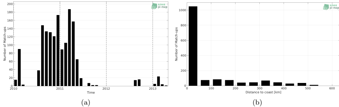
Figure 1: Number of match-ups between Marine mammals and SMOS SSS L3 v5 - 9 Days (CATDS-CECOS-LOCEAN) SSS as a function of time (a) and as function of the distance to coast (b) over the Arctic Ocean Pi-MEP region and for the full satellite product period.
