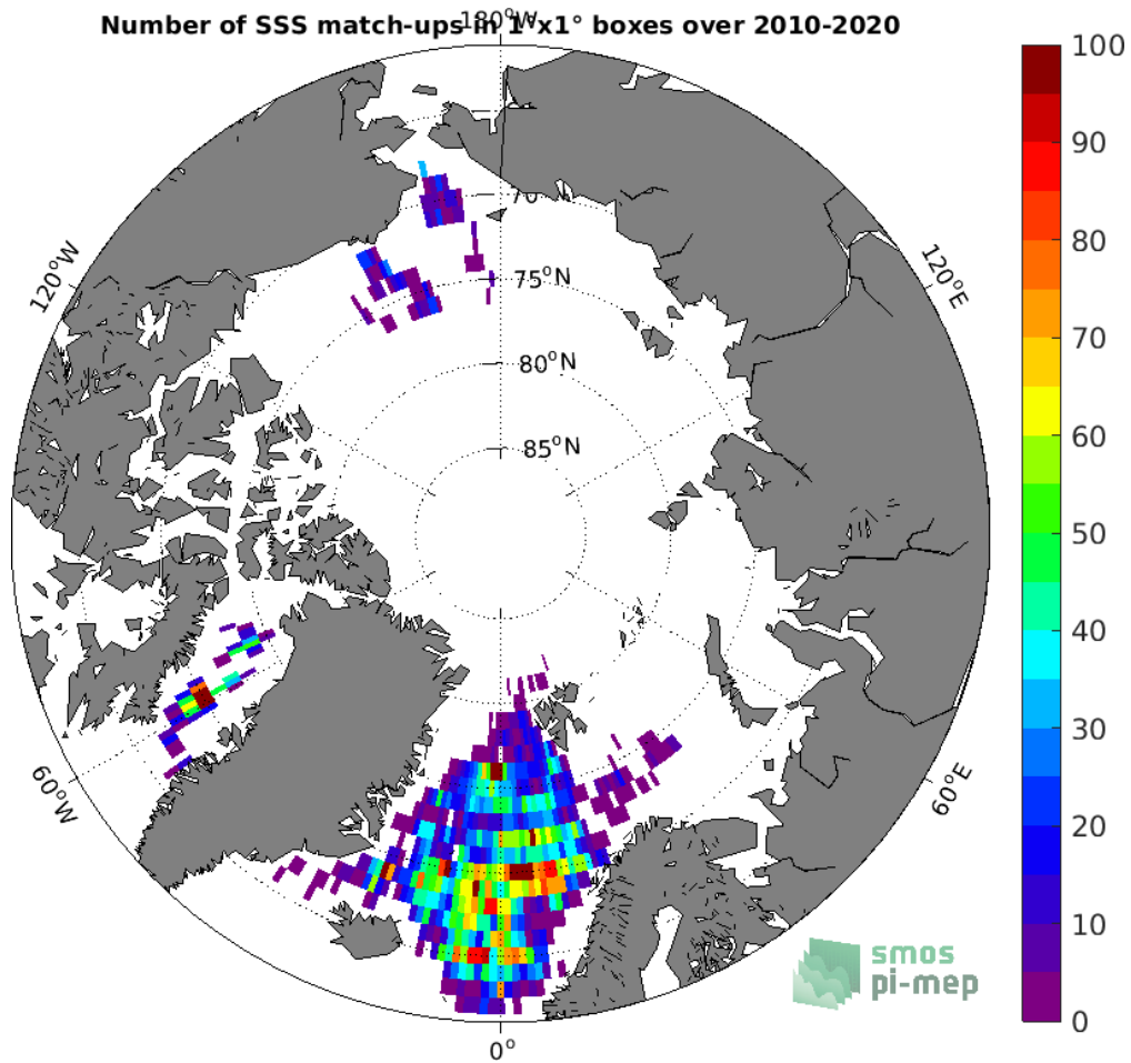
Figure 4: Number of SSS match-ups between Argo SSS and the SMOS SSS L3 v5 - 9 Days (CATDS-CECOS-LOCEAN) SSS product for the Arctic Ocean Pi-MEP region over 1°x1° boxes and for the full satellite product period.
