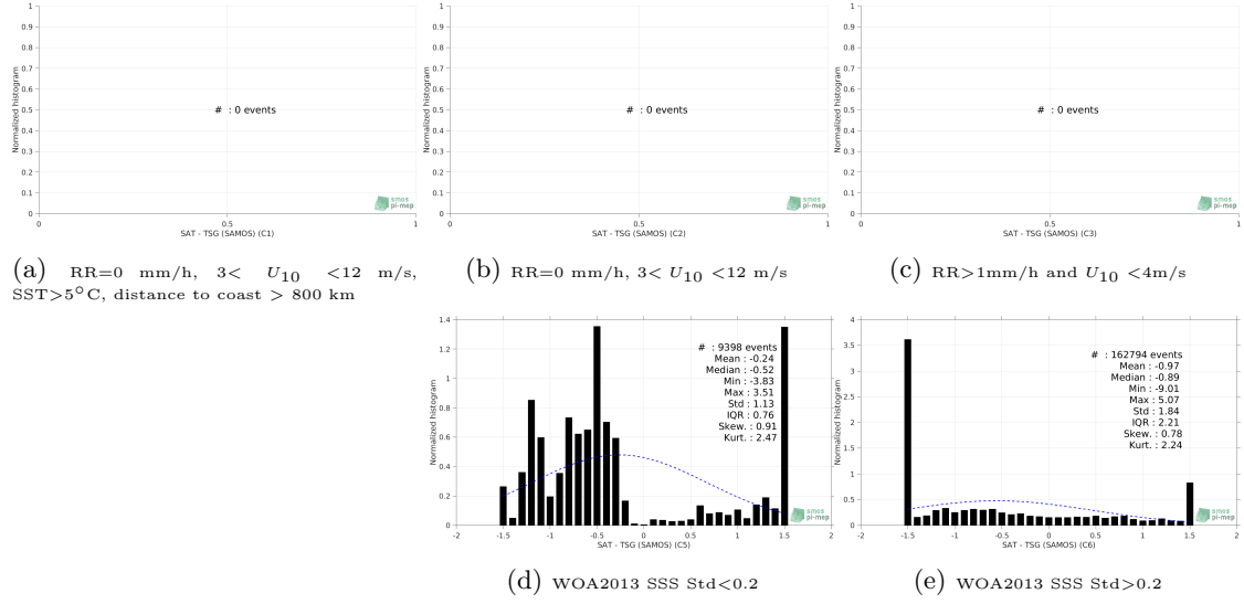
Figure 13: Normalized histogram of \Delta\text{SSS} (SMOS SSS L3 v5 - 18 Days (CATDS-CECOS-LOCEAN) - TSG (SAMOS)) for 5 different subdatasets corresponding to: RR=0 mm/h, 3 < U_{10} < 12 m/s, SST > 5^\circ\text{C} , distance to coast > 800 km (a), RR=0 mm/h, 3 < U_{10} < 12 m/s (b), RR > 1 mm/h and U_{10} < 4 m/s (c), WOA2013 SSS Std < 0.2 (d), WOA2013 SSS Std > 0.2 (e).
