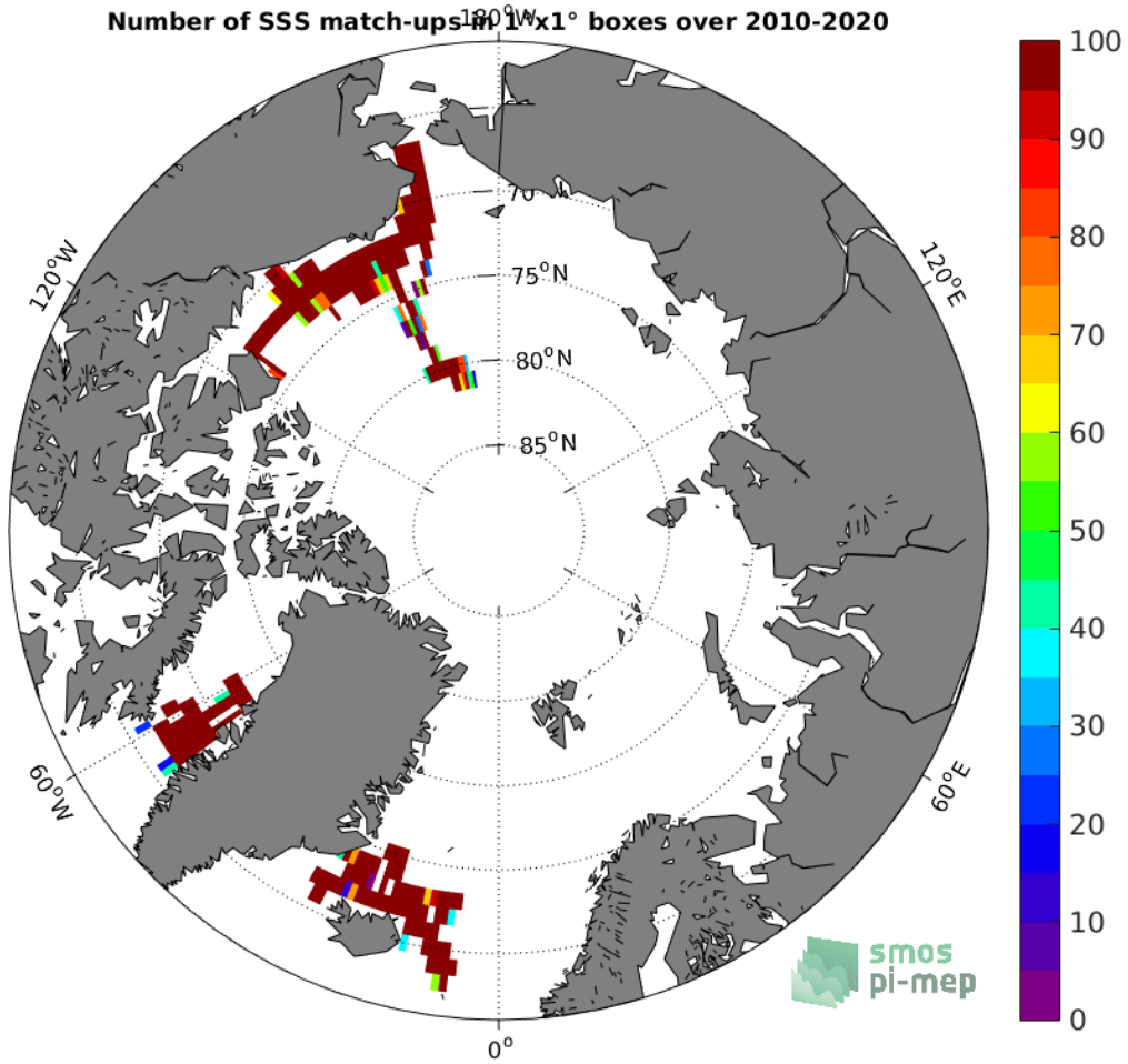
Figure 4: Number of SSS match-ups between TSG (SAMOS) SSS and the SMOS SSS L3 v5 - 18 Days (CATDS-CECOS-LOCEAN) SSS product for the Arctic Ocean Pi-MEP region over 1^\circ \times 1^\circ boxes and for the full satellite product period.
