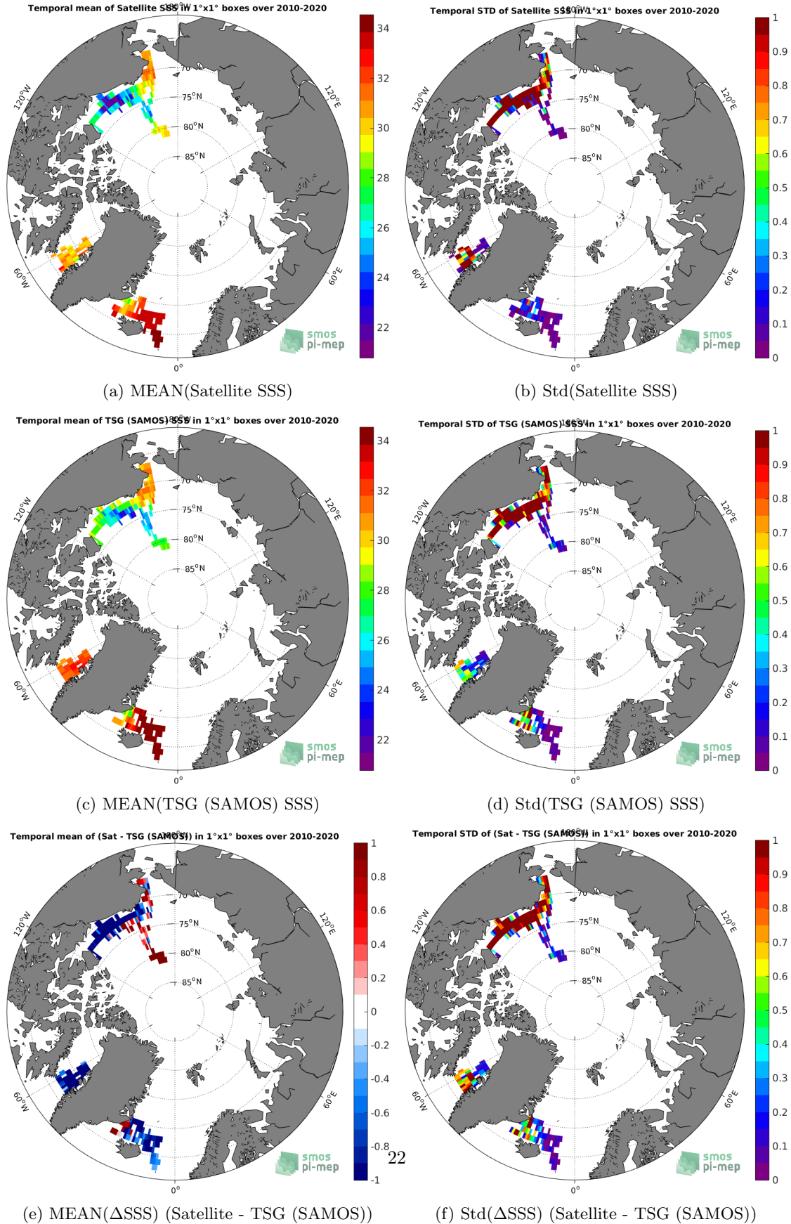
Figure 6: Temporal mean (left) and Std (right) of SSS from SMOS SSS L3 v5 - 18 Days (CATDS-CECOS-LOCEAN) (top), TSG (SAMOS) (middle), and of \Delta SSS (Satellite - TSG (SAMOS)). Only match-up pairs are used to generate these maps.
