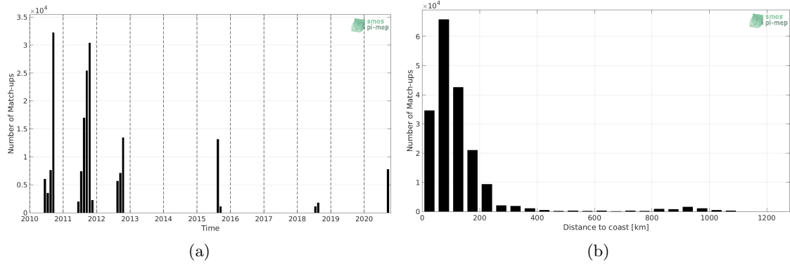
Figure 1: Number of match-ups between TSG (SAMOS) and SMOS SSS L3 v5 - 18 Days (CATDS-CECOS-LOCEAN) SSS as a function of time (a) and as function of the distance to coast (b) over the Arctic Ocean Pi-MEP region and for the full satellite product period.
