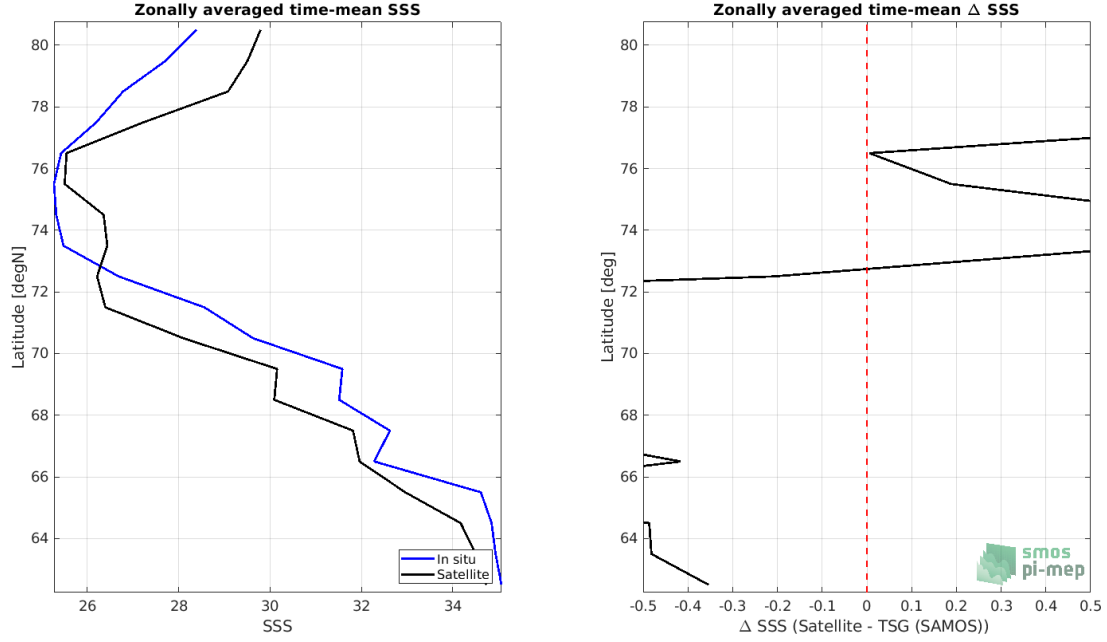
Figure 8: Left panel: Zonal mean SSS from SMOS SSS L3 v5 - 18 Days (CATDS-CECOS-LOCEAN) satellite product (black) and from TSG (SAMOS) (blue). Right panel: Zonal mean of \Delta\text{SSS} (Satellite - TSG (SAMOS)) for all the collected Pi-MEP match-up pairs estimated over the full satellite product period.
