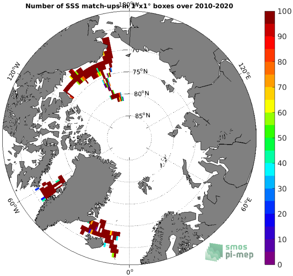
Figure 4: Number of SSS match-ups between TSG (SAMOS) SSS and the SMOS SSS L3 v5 - 18 Days (CATDS-CECOS-LOCEAN) SSS product for the Arctic Ocean Pi-MEP region over 1°x1° boxes and for the full satellite product period.
