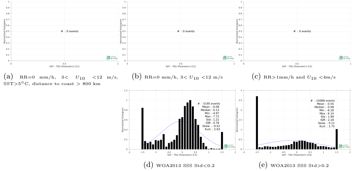
Figure 13: Normalized histogram of \Delta\text{SSS} (SMOS SSS L3 v5 - 18 Days (CATDS-CECOS-LOCEAN) - TSG (Polarstern)) for 5 different subdatasets corresponding to: RR=0 mm/h, 3 < U_{10} < 12 m/s, SST > 5^\circ\text{C} , distance to coast > 800 km (a), RR=0 mm/h, 3 < U_{10} < 12 m/s (b), RR > 1 mm/h and U_{10} < 4 m/s (c), WOA2013 SSS Std < 0.2 (d), WOA2013 SSS Std > 0.2 (e).
