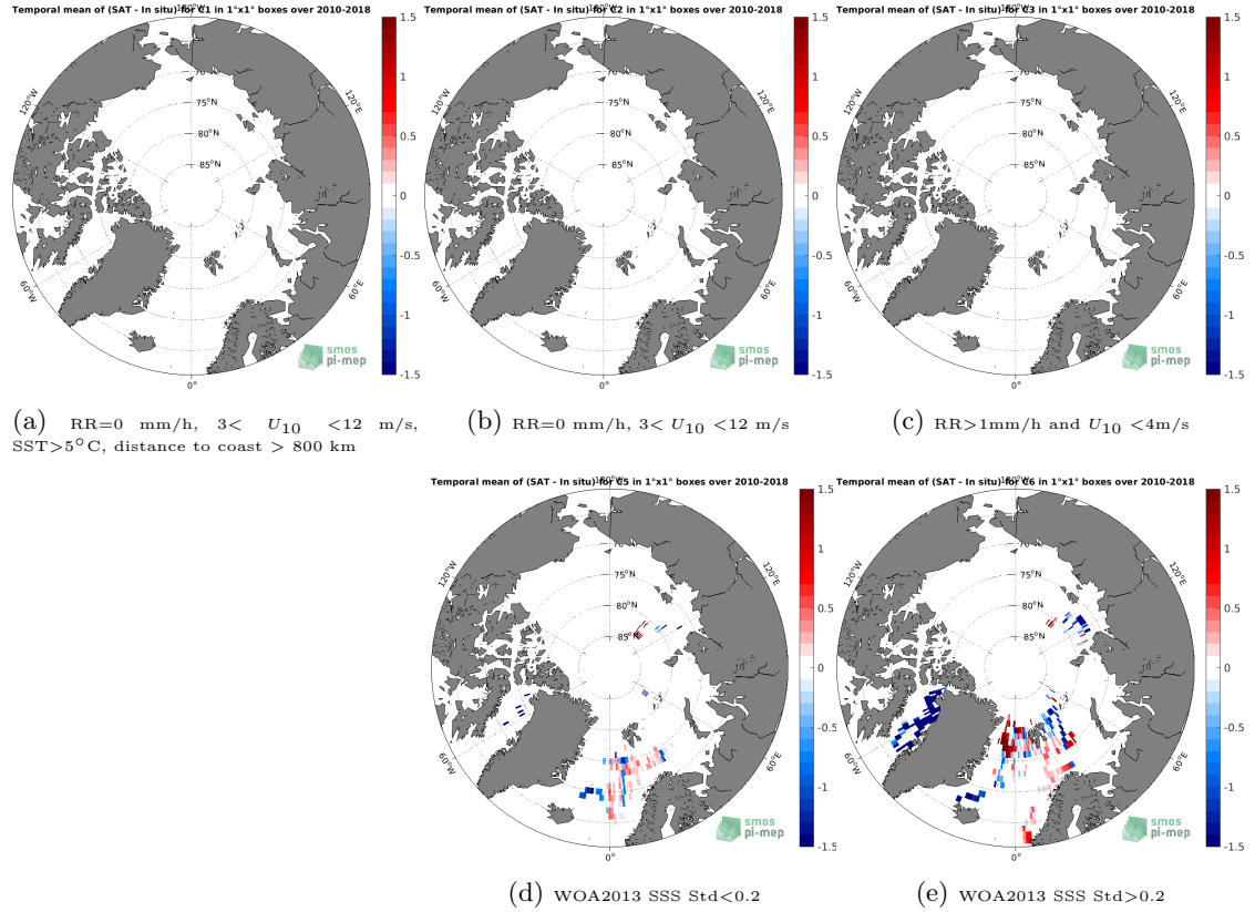
Figure 12: Temporal mean gridded over spatial boxes of size 1^{\circ}\times 1^{\circ} of \Delta\text{SSS} (SMOS SSS L3 v5 - 18 Days (CATDS-CECOS-LOCEAN) - TSG (Polarstern)) for 5 different subdatasets corresponding to: RR=0 mm/h, 3 < U_{10} < 12 m/s, SST >5^{\circ}\text{C} , distance to coast > 800 km (a), RR=0 mm/h, 3 < U_{10} < 12 m/s (b), RR >1 mm/h and U_{10} < 4 m/s (c), WOA2013 SSS Std <0.2 (d), WOA2013 SSS Std >0.2 (e).
