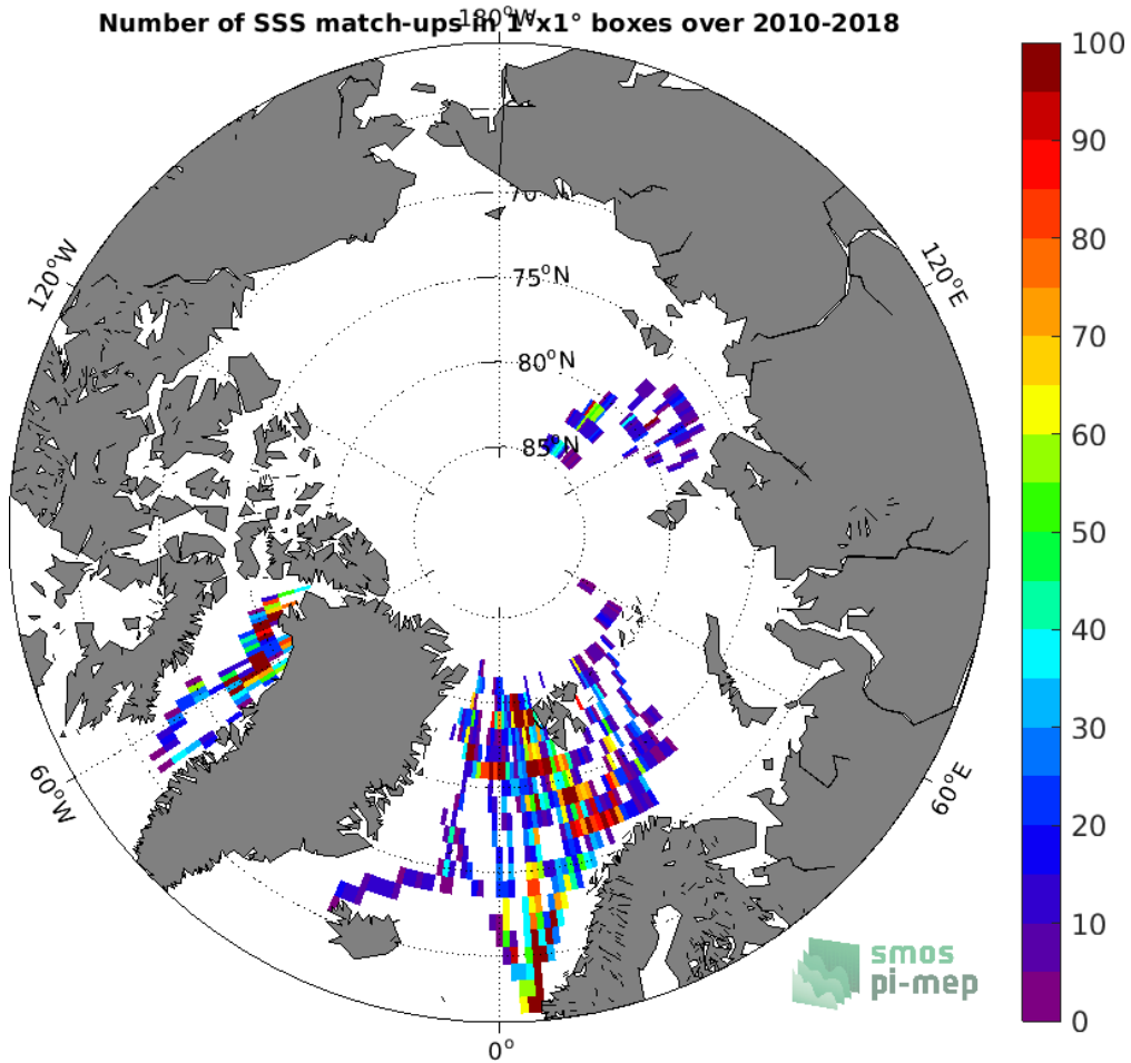
Figure 4: Number of SSS match-ups between TSG (Polarstern) SSS and the SMOS SSS L3 v5 - 18 Days (CATDS-CECOS-LOCEAN) SSS product for the Arctic Ocean Pi-MEP region over 1^\circ \times 1^\circ boxes and for the full satellite product period.
