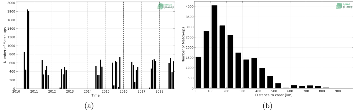
Figure 1: Number of match-ups between TSG (Polarstern) and SMOS SSS L3 v5 - 18 Days (CATDS-CECOS-LOCEAN) SSS as a function of time (a) and as function of the distance to coast (b) over the Arctic Ocean Pi-MEP region and for the full satellite product period.
