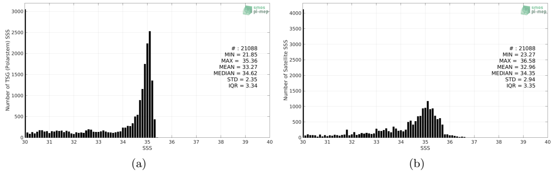
Figure 2: Histograms of SSS from TSG (Polarstern) (a) and SMOS SSS L3 v5 - 18 Days (CATDS-CECOS-LOCEAN) (b) considering all match-up pairs per bins of 0.1 over the Arctic Ocean Pi-MEP region and for the full satellite product period.
