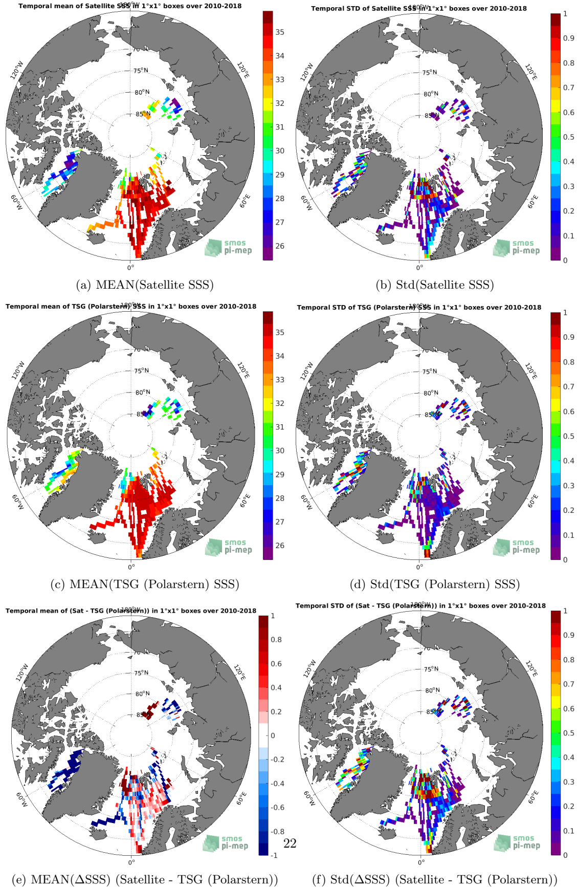
Figure 6: Temporal mean (left) and Std (right) of SSS from SMOS SSS L3 v5 - 18 Days (CATDS-CECOS-LOCEAN) (top), TSG (Polarstern) (middle), and of \Delta SSS (Satellite - TSG (Polarstern)). Only match-up pairs are used to generate these maps.
