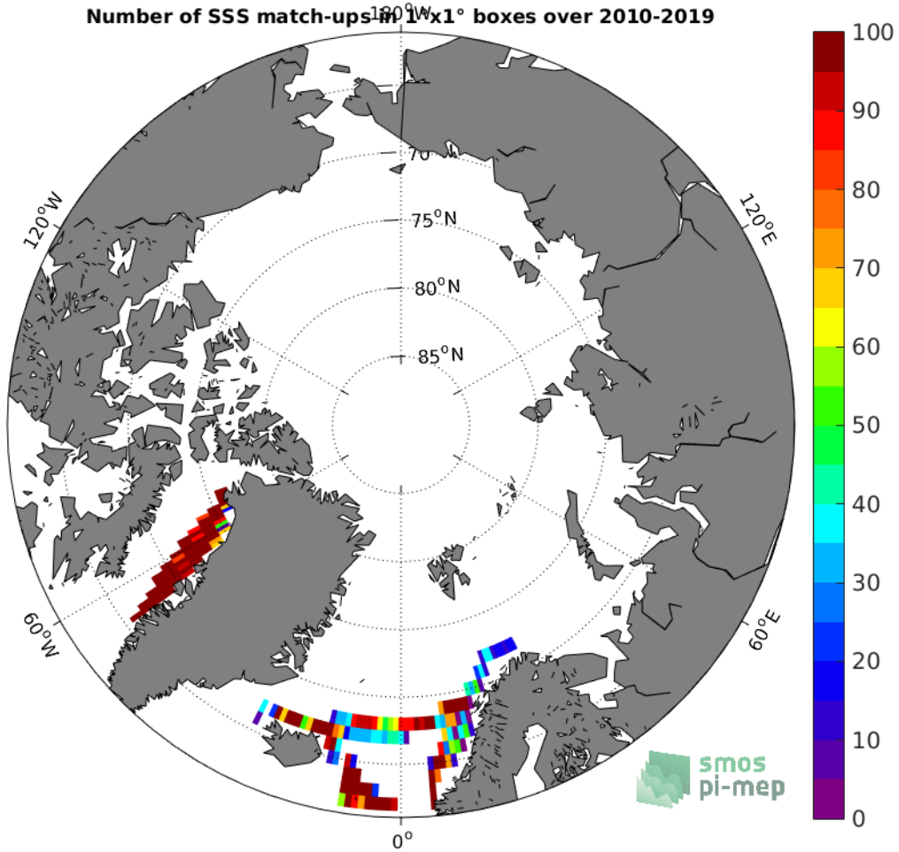
Figure 4: Number of SSS match-ups between TSG (LEGOS-DM) SSS and the SMOS SSS L3 v5 - 18 Days (CATDS-CECOS-LOCEAN) SSS product for the Arctic Ocean Pi-MEP region over 1^\circ \times 1^\circ boxes and for the full satellite product period.
