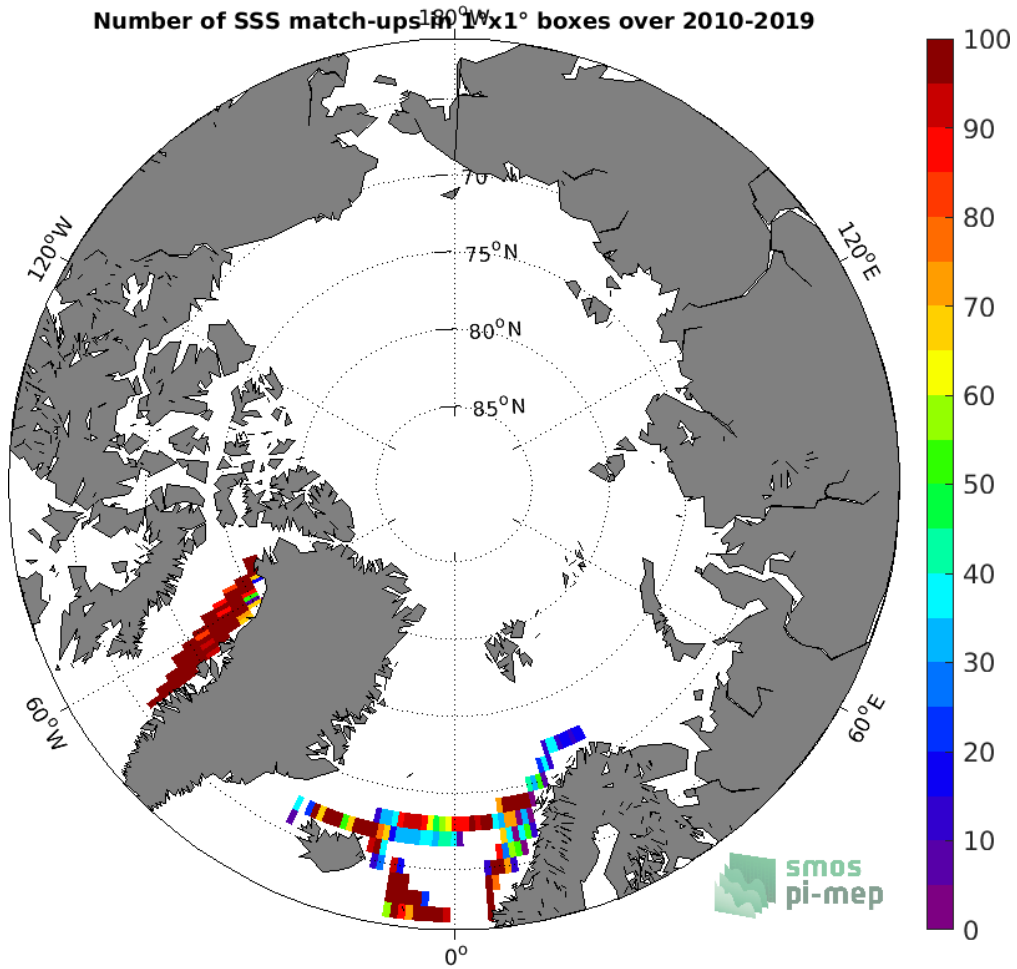
Figure 4: Number of SSS match-ups between TSG (LEGOS-DM) SSS and the SMOS SSS L3 v5 - 18 Days (CATDS-CECOS-LOCEAN) SSS product for the Arctic Ocean Pi-MEP region over 1°x1° boxes and for the full satellite product period.
