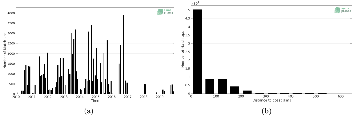
Figure 1: Number of match-ups between TSG (LEGOS-DM) and SMOS SSS L3 v5 - 18 Days (CATDS-CECOS-LOCEAN) SSS as a function of time (a) and as function of the distance to coast (b) over the Arctic Ocean Pi-MEP region and for the full satellite product period.
