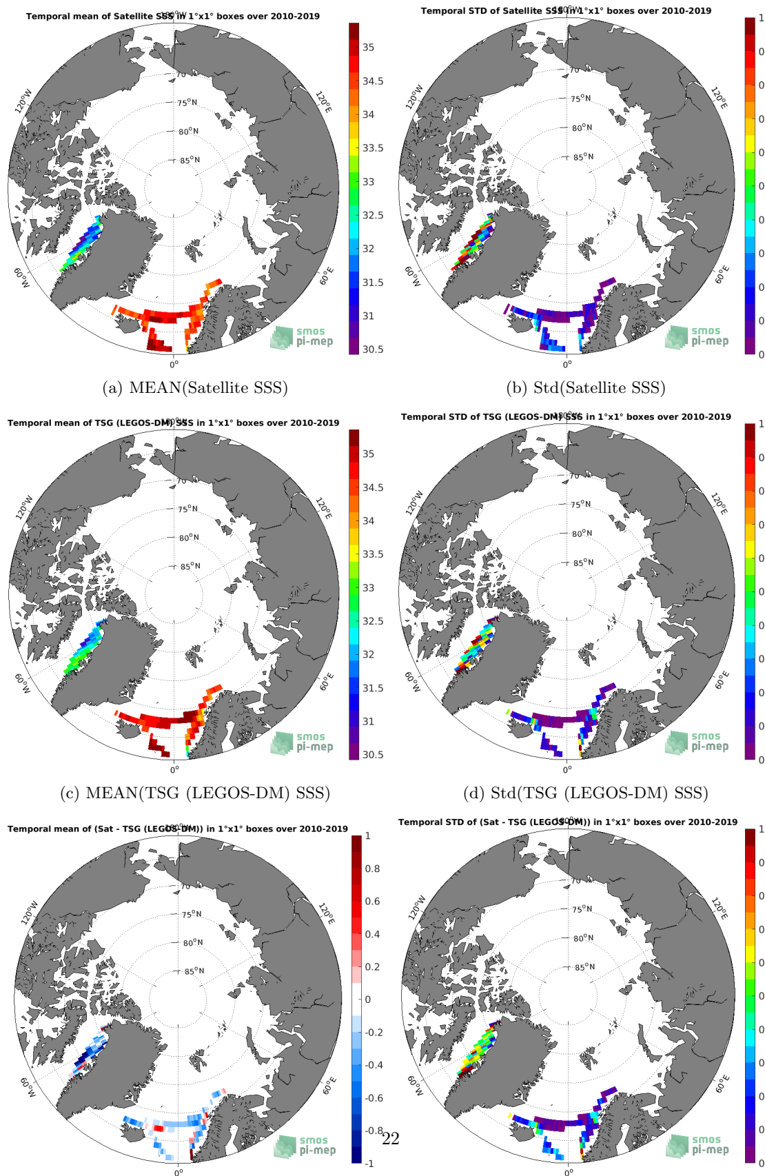
Figure 6: Temporal mean (left) and Std (right) of SSS from SMOS SSS L3 v5 - 18 Days (CATDS-CECOS-LOCEAN) (top), TSG (LEGOS-DM) (middle), and of \Delta SSS (Satellite - TSG (LEGOS-DM)). Only match-up pairs are used to generate these maps.
