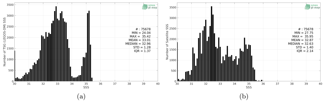
Figure 2: Histograms of SSS from TSG (LEGOS-DM) (a) and SMOS SSS L3 v5 - 18 Days (CATDS-CECOS-LOCEAN) (b) considering all match-up pairs per bins of 0.1 over the Arctic Ocean Pi-MEP region and for the full satellite product period.
