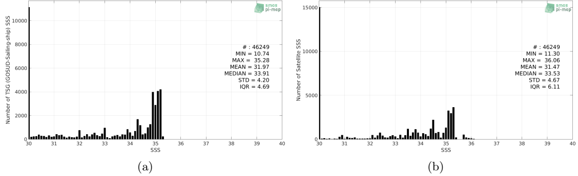
Figure 2: Histograms of SSS from TSG (GOSUD-Sailing-ship) (a) and SMOS SSS L3 v5 - 18 Days (CATDS-CECOS-LOCEAN) (b) considering all match-up pairs per bins of 0.1 over the Arctic Ocean Pi-MEP region and for the full satellite product period.
