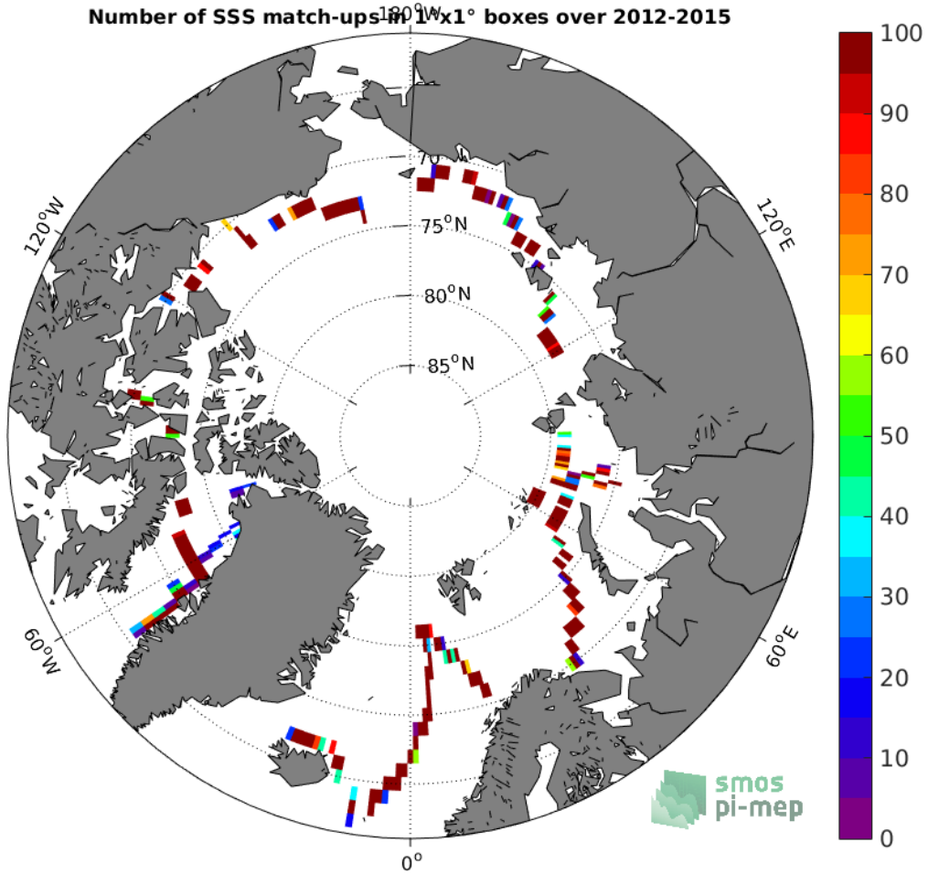
Figure 4: Number of SSS match-ups between TSG (GOSUD-Sailing-ship) SSS and the SMOS SSS L3 v5 - 18 Days (CATDS-CECOS-LOCEAN) SSS product for the Arctic Ocean Pi-MEP region over 1^\circ \times 1^\circ boxes and for the full satellite product period.
