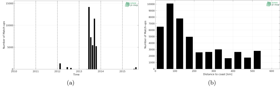
Figure 1: Number of match-ups between TSG (GOSUD-Sailing-ship) and SMOS SSS L3 v5 - 18 Days (CATDS-CECOS-LOCEAN) SSS as a function of time (a) and as function of the distance to coast (b) over the Arctic Ocean Pi-MEP region and for the full satellite product period.
