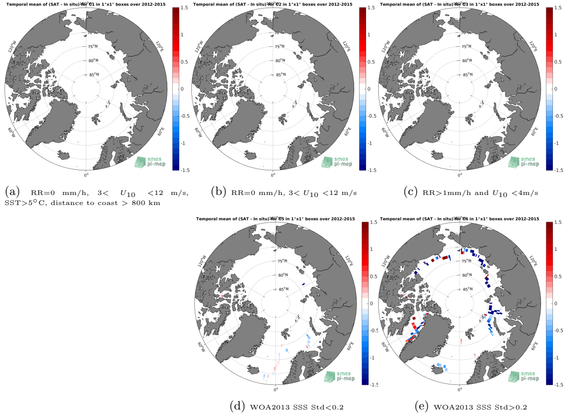
Figure 12: Temporal mean gridded over spatial boxes of size 1^{\circ} \times 1^{\circ} of \Delta\text{SSS} (SMOS SSS L3 v5 - 18 Days (CATDS-CECOS-LOCEAN) - TSG (GOSUD-Sailing-ship)) for 5 different subdatasets corresponding to: RR=0 mm/h, 3 < U_{10} < 12 m/s, SST > 5^{\circ}\text{C} , distance to coast > 800 km (a), RR=0 mm/h, 3 < U_{10} < 12 m/s (b), RR > 1\text{mm/h} and U_{10} < 4\text{m/s} (c), WOA2013 SSS Std < 0.2 (d), WOA2013 SSS Std > 0.2 (e).
