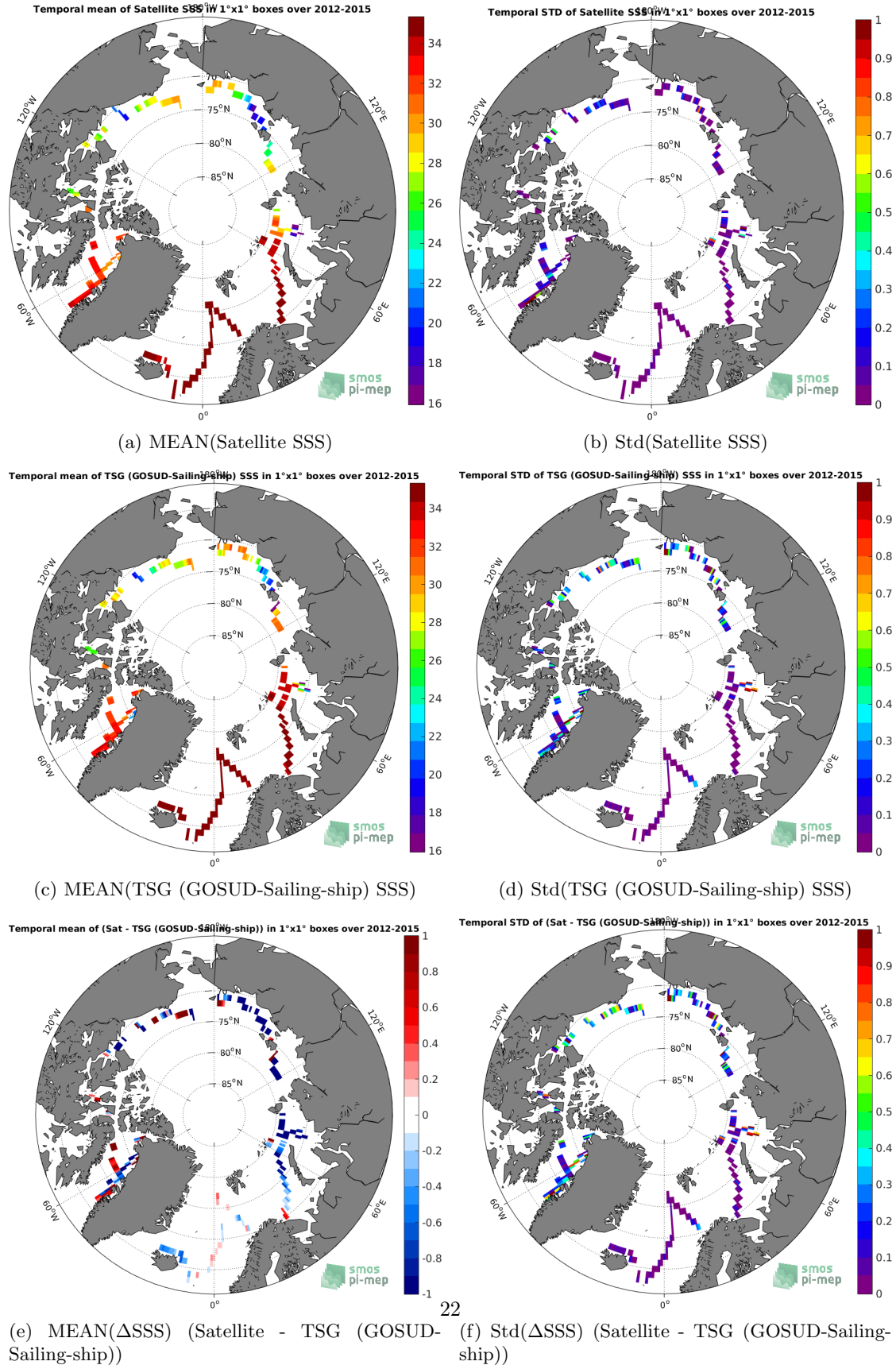
Figure 6: Temporal mean (left) and Std (right) of SSS from SMOS SSS L3 v5 - 18 Days (CATDS-CECOS-LOCEAN) (top), TSG (GOSUD-Sailing-ship) (middle), and of \Delta SSS (Satellite - TSG (GOSUD-Sailing-ship)). Only match-up pairs are used to generate these maps.
