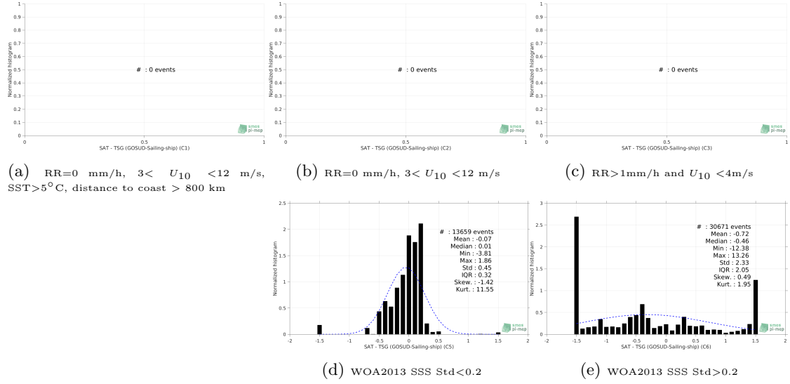
Figure 13: Normalized histogram of \Delta\text{SSS} (SMOS SSS L3 v5 - 18 Days (CATDS-CECOS-LOCEAN) - TSG (GOSUD-Sailing-ship)) for 5 different subdatasets corresponding to: RR=0 mm/h, 3 < U_{10} < 12 m/s, SST > 5^\circ\text{C} , distance to coast > 800 km (a), RR=0 mm/h, 3 < U_{10} < 12 m/s (b), RR > 1\text{mm/h} and U_{10} < 4\text{m/s} (c), WOA2013 SSS Std<0.2 (d), WOA2013 SSS Std>0.2 (e).
