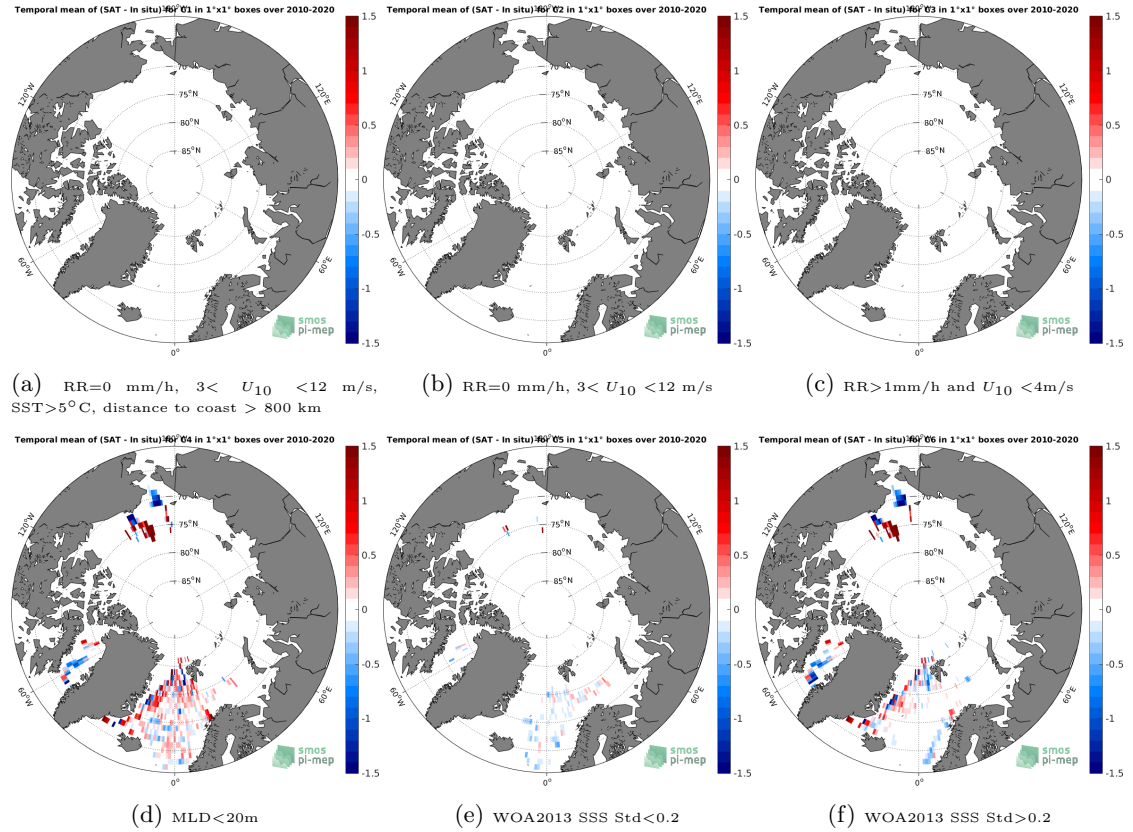
Figure 12: Temporal mean gridded over spatial boxes of size 1^{\circ} \times 1^{\circ} of \Delta\text{SSS} (SMOS SSS L3 v5 - 18 Days (CATDS-CECOS-LOCEAN) - Argo) for 6 different subdatasets corresponding to: RR=0 mm/h, 3 < U_{10} < 12 m/s, SST > 5^{\circ}\text{C} , distance to coast > 800 km (a), RR=0 mm/h, 3 < U_{10} < 12 m/s (b), RR > 1 mm/h and U_{10} < 4 m/s (c), MLD < 20\text{m} (d), WOA2013 SSS Std < 0.2 (e), WOA2013 SSS Std > 0.2 (f).
