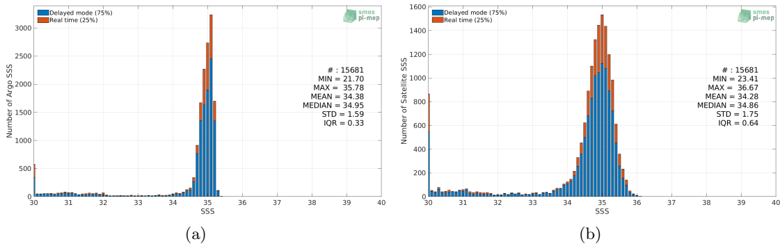
Figure 2: Histograms of SSS from Argo (a) and SMOS SSS L3 v5 - 18 Days (CATDS-CECOS-LOCEAN) (b) considering all match-up pairs per bins of 0.1 over the Arctic Ocean Pi-MEP region and for the full satellite product period.
