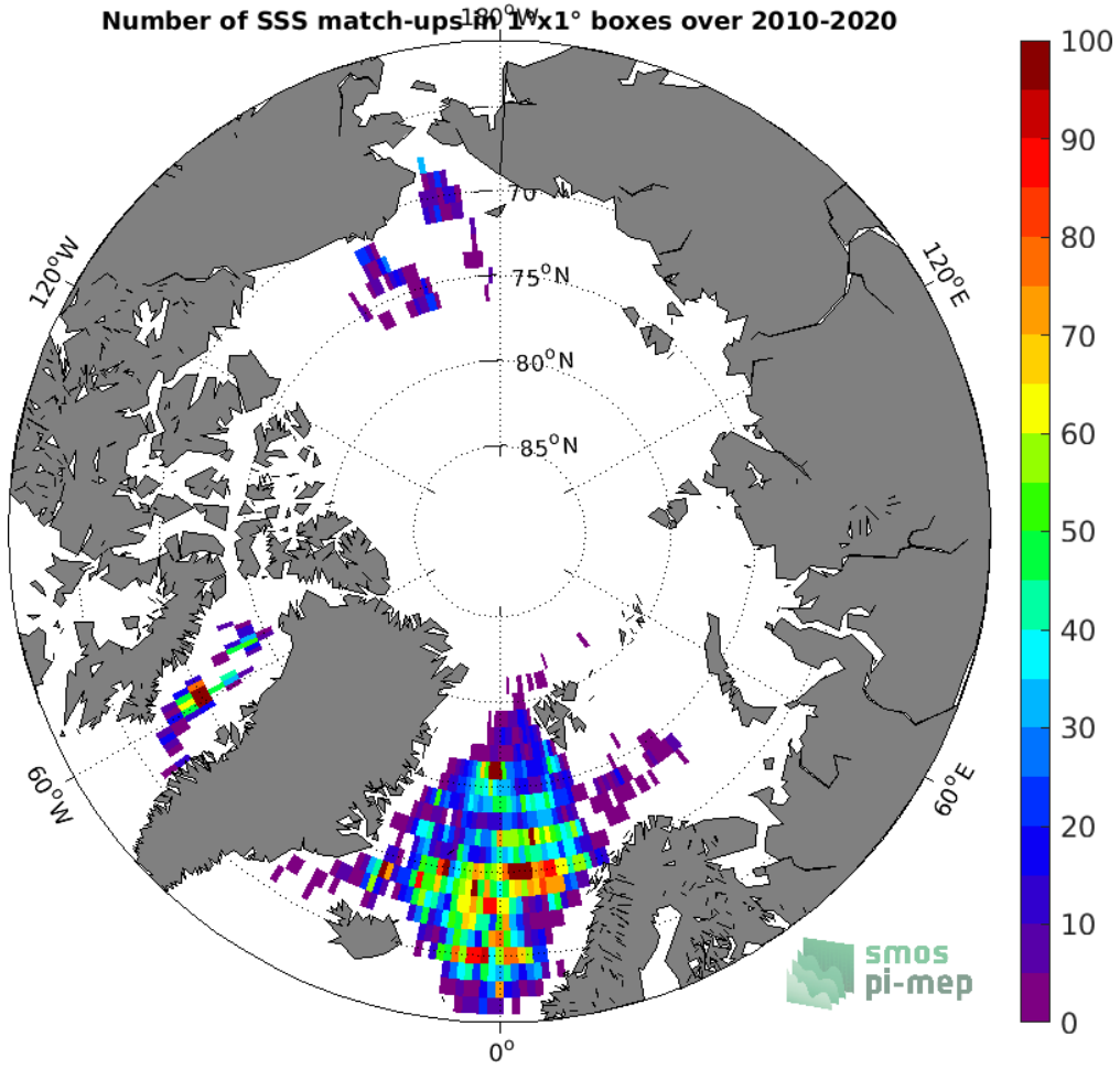
Figure 4: Number of SSS match-ups between Argo SSS and the SMOS SSS L3 v5 - 18 Days (CATDS-CECOS-LOCEAN) SSS product for the Arctic Ocean Pi-MEP region over 1^\circ \times 1^\circ boxes and for the full satellite product period.
