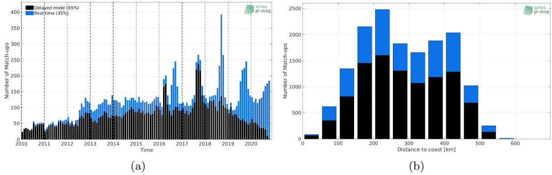
Figure 1: Number of match-ups between Argo and SMOS SSS L3 v5 - 18 Days (CATDS-CECOS-LOCEAN) SSS as a function of time (a) and as function of the distance to coast (b) over the Arctic Ocean Pi-MEP region and for the full satellite product period.
