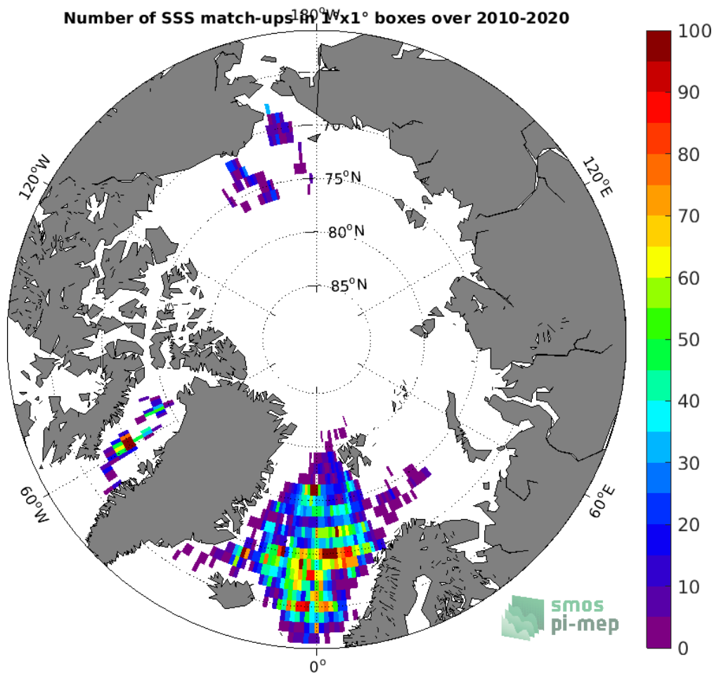
Figure 4: Number of SSS match-ups between Argo SSS and the SMOS SSS L3 v5 - 18 Days (CATDS-CECOS-LOCEAN) SSS product for the Arctic Ocean Pi-MEP region over 1°x1° boxes and for the full satellite product period.
