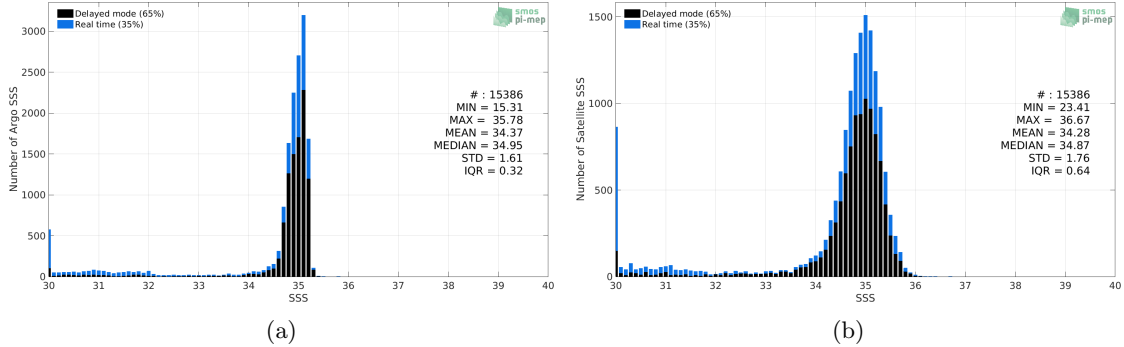
Figure 2: Histograms of SSS from Argo (a) and SMOS SSS L3 v5 - 18 Days (CATDS-CECOS-LOCEAN) (b) considering all match-up pairs per bins of 0.1 over the Arctic Ocean Pi-MEP region and for the full satellite product period.
