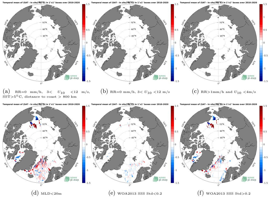
Figure 12: Temporal mean gridded over spatial boxes of size 1^{\circ}\times 1^{\circ} of \Delta\text{SSS} (SMOS SSS L3 v5 - 18 Days (CATDS-CECOS-LOCEAN) - Argo) for 6 different subdatasets corresponding to:RR=0 mm/h, 3 < U_{10} < 12 m/s, SST >5^{\circ}\text{C} , distance to coast > 800 km (a), RR=0 mm/h, 3 < U_{10} < 12 m/s (b), RR >1 mm/h and U_{10} < 4 m/s (c),MLD <20 m (d),WOA2013 SSS Std <0.2 (e),WOA2013 SSS Std >0.2 (f).
