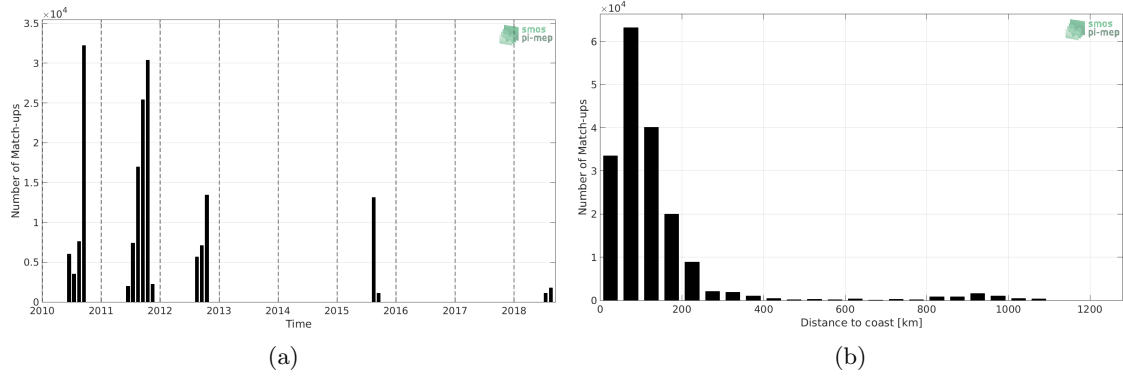
Figure 1: Number of match-ups between TSG (SAMOS) and SMOS SSS L3 v4 - 9 Days (CATDS-CECOS-LOCEAN) SSS as a function of time (a) and as function of the distance to coast (b) over the Arctic Ocean Pi-MEP region and for the full satellite product period.
