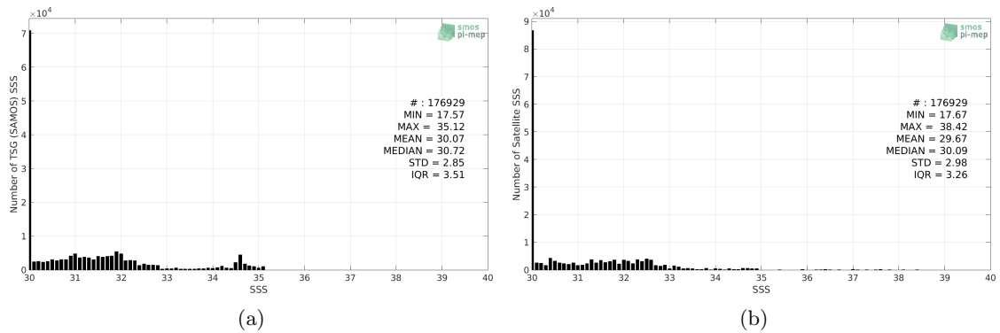
Figure 2: Histograms of SSS from TSG (SAMOS) (a) and SMOS SSS L3 v4 - 9 Days (CATDS-CECOS-LOCEAN) (b) considering all match-up pairs per bins of 0.1 over the Arctic Ocean Pi-MEP region and for the full satellite product period.
