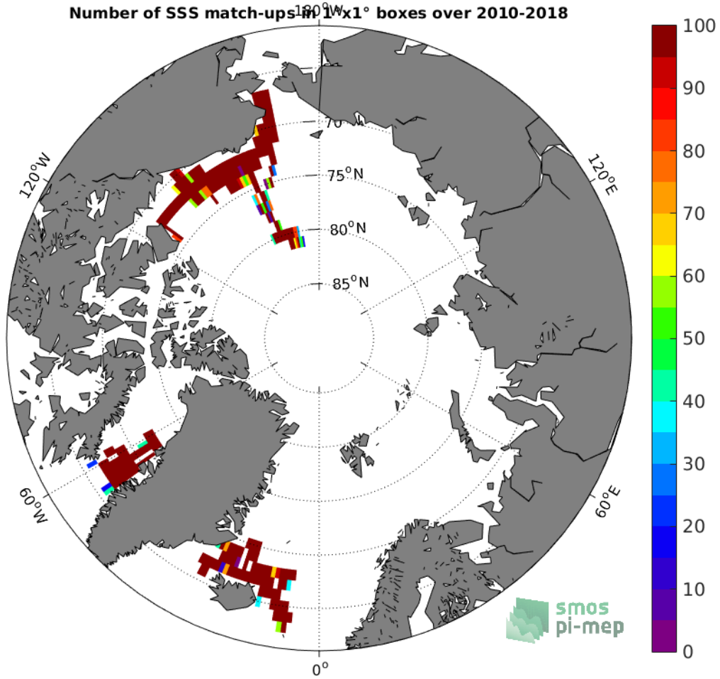
Figure 4: Number of SSS match-ups between TSG (SAMOS) SSS and the SMOS SSS L3 v4 - 9 Days (CATDS-CECOS-LOCEAN) SSS product for the Arctic Ocean Pi-MEP region over 1°x1° boxes and for the full satellite product period.
