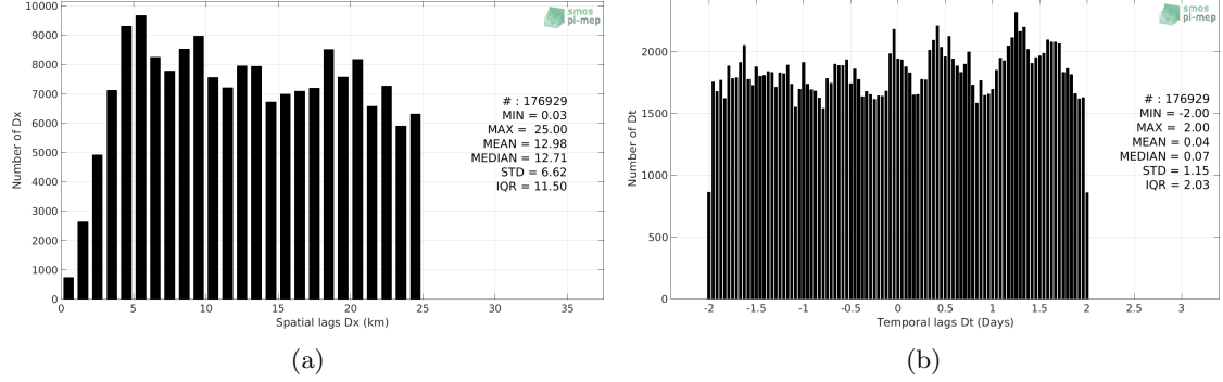
Figure 5: Histograms of the spatial (a) and temporal (b) lags between the time of the TSG (SAMOS) measurements and the date of the corresponding SMOS SSS L3 v4 - 9 Days (CATDS-CECOS-LOCEAN) SSS product.
