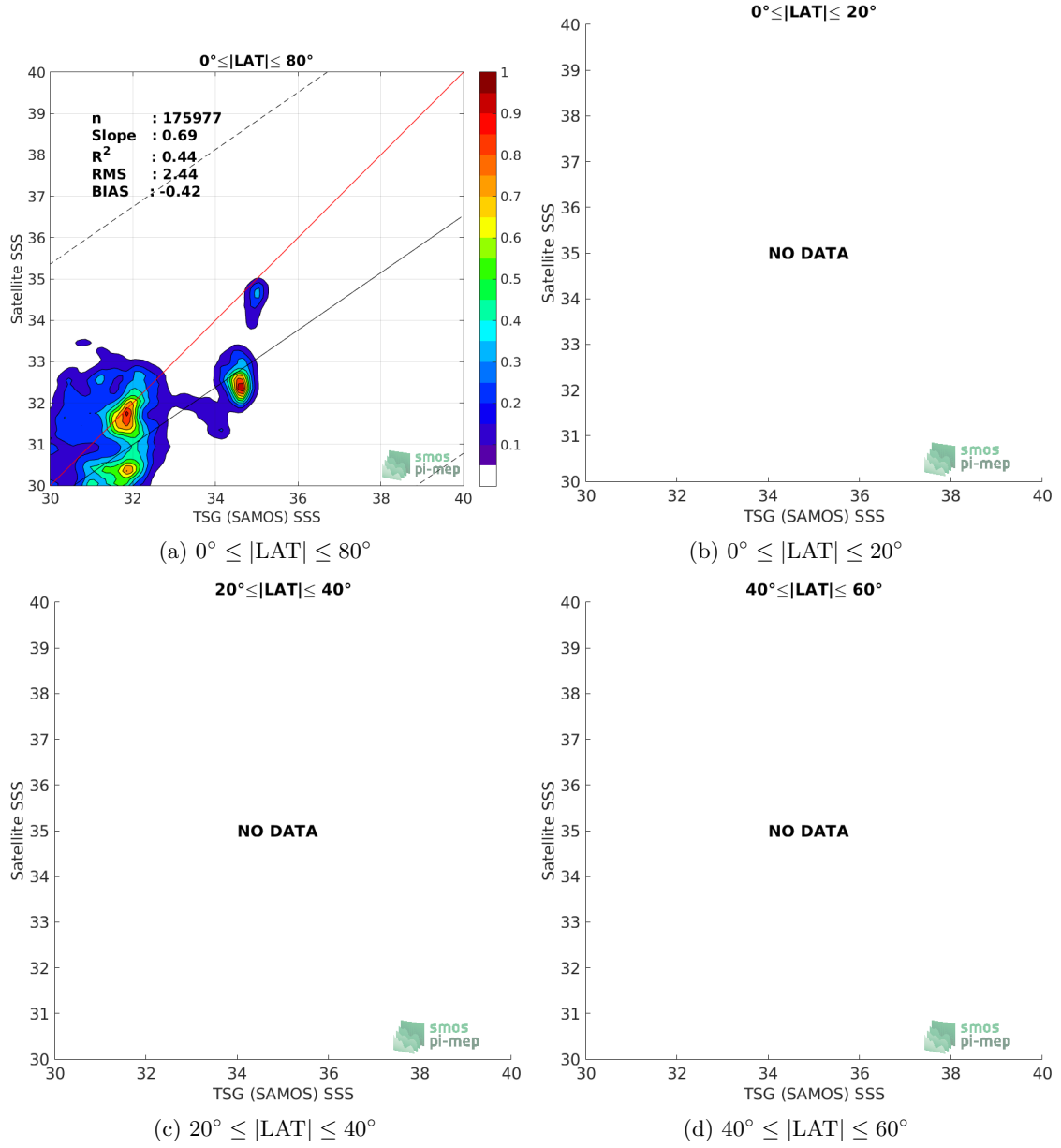
Figure 9: Contour maps of the concentration of SMOS SSS L3 v4 - 9 Days (CATDS-CECOS-LOCEAN) SSS (y-axis) versus TSG (SAMOS) SSS (x-axis) at match-up pairs for different latitude bands. For each plot, the red line shows x=y . The black thin and dashed lines indicate a linear fit through the data cloud and the \pm 95\% confidence levels, respectively. The number match-up pairs n , the slope and R^2 coefficient of the linear fit, the root mean square (RMS) and the mean bias between satellite and in situ data are indicated for each latitude band in each plots.
