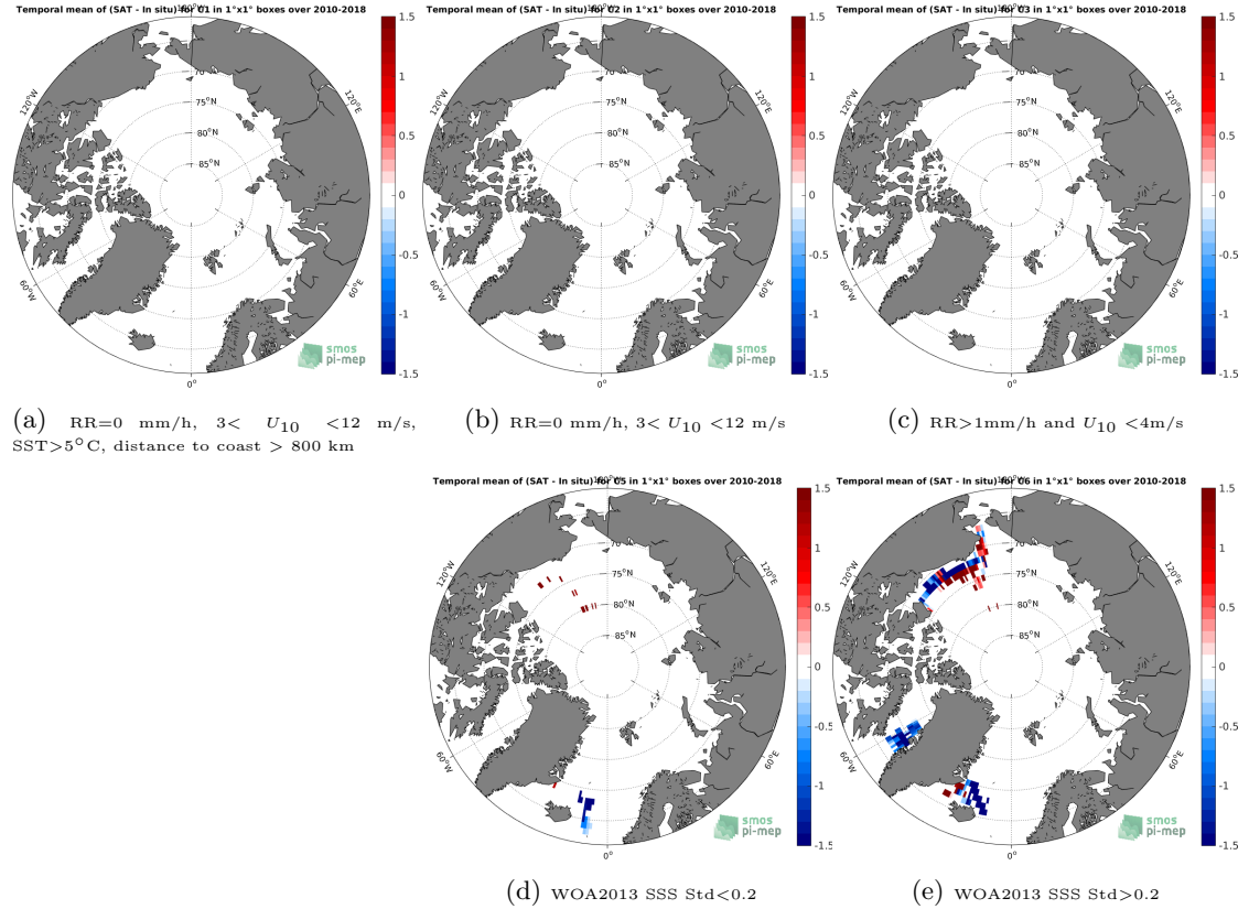
Figure 12: Temporal mean gridded over spatial boxes of size 1^{\circ}\times 1^{\circ} of \Delta\text{SSS} (SMOS SSS L3 v4 - 9 Days (CATDS-CECOS-LOCEAN) - TSG (SAMOS)) for 5 different subdatasets corresponding to: \text{RR}=0 mm/h, 3 < U_{10} < 12 m/s, \text{SST} > 5^{\circ}\text{C} , distance to coast > 800 km (a), \text{RR}=0 mm/h, 3 < U_{10} < 12 m/s (b), \text{RR} > 1 mm/h and U_{10} < 4 m/s (c), WOA2013 SSS Std < 0.2 (d), WOA2013 SSS Std > 0.2 (e).
