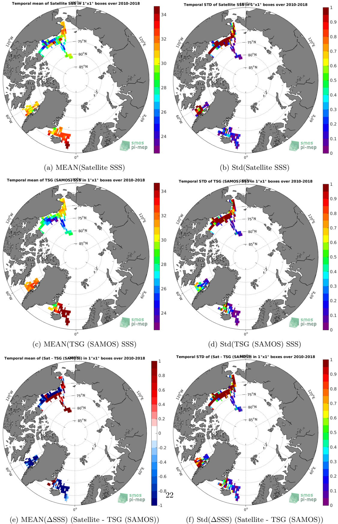
Figure 6: Temporal mean (left) and Std (right) of SSS from SMOS SSS L3 v4 - 9 Days (CATDS-CECOS-LOCEAN) (top), TSG (SAMOS) (middle), and of \Delta SSS (Satellite - TSG (SAMOS)). Only match-up pairs are used to generate these maps.
