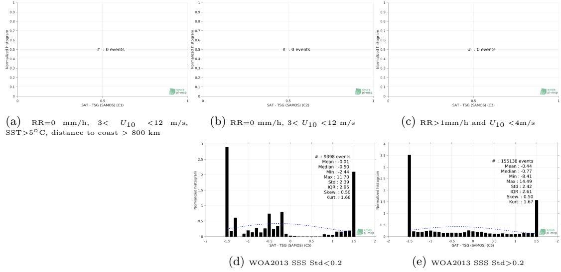
Figure 13: Normalized histogram of \Delta\text{SSS} (SMOS SSS L3 v4 - 9 Days (CATDS-CECOS-LOCEAN) - TSG (SAMOS)) for 5 different subdatasets corresponding to: RR=0 mm/h, 3 < U_{10} < 12 m/s, SST > 5^\circ\text{C} , distance to coast > 800 km (a), RR=0 mm/h, 3 < U_{10} < 12 m/s (b), RR > 1\text{mm/h} and U_{10} < 4\text{m/s} (c), WOA2013 SSS Std < 0.2 (d), WOA2013 SSS Std > 0.2 (e).
