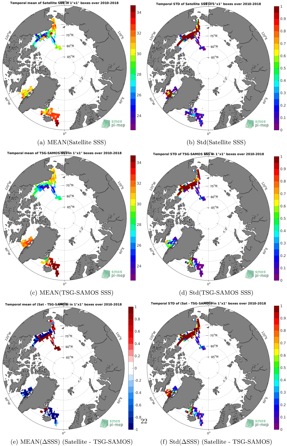
Figure 6: Temporal mean (left) and Std (right) of SSS from SMOS-L3-CATDS-CECOS-LOCEAN-V4-9DAYS-25KM (top), TSG-SAMOS (middle), and of \Delta SSS (Satellite - TSG-SAMOS). Only match-up pairs are used to generate these maps.
