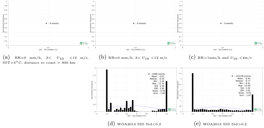
Figure 13: Normalized histogram of \Delta\text{SSS} (SMOS-L3-CATDS-CECOS-LOCEAN-V4-9DAYS-25KM - TSG-SAMOS) for 5 different subdatasets corresponding to: RR=0 mm/h, 3 < U_{10} < 12 m/s, SST > 5^\circ\text{C} , distance to coast > 800 km (a), RR=0 mm/h, 3 < U_{10} < 12 m/s (b), RR > 1 mm/h and U_{10} < 4 m/s (c), WOA2013 SSS Std < 0.2 (d), WOA2013 SSS Std > 0.2 (e).
