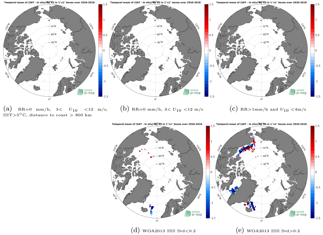
Figure 12: Temporal mean gridded over spatial boxes of size 1^{\circ}\times 1^{\circ} of \Delta\text{SSS} (SMOS-L3-CATDS-CECOS-LOCEAN-V4-9DAYS-25KM - TSG-SAMOS) for 5 different subdatasets corresponding to: RR=0 mm/h, 3 < U_{10} < 12 m/s, SST > 5^{\circ}\text{C} , distance to coast > 800 km (a), RR=0 mm/h, 3 < U_{10} < 12 m/s (b), RR > 1 mm/h and U_{10} < 4 m/s (c), WOA2013 SSS Std < 0.2 (d), WOA2013 SSS Std > 0.2 (e).
