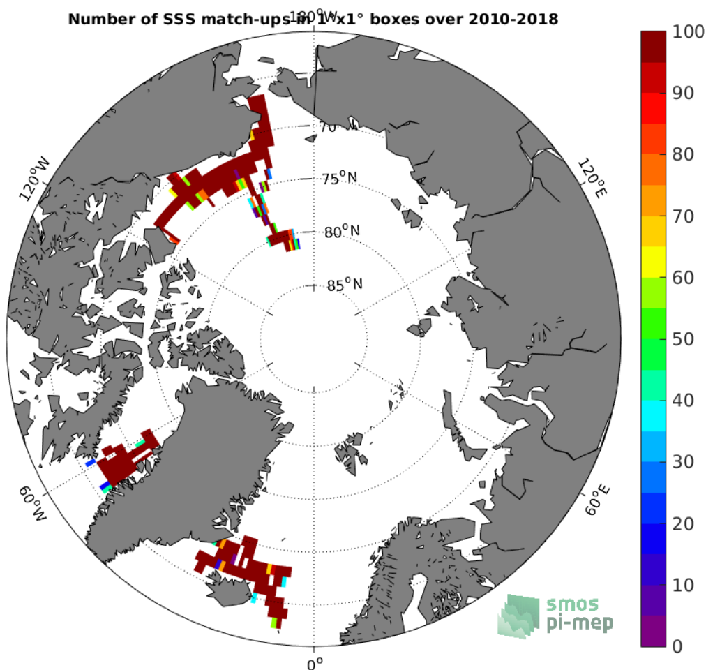
Figure 4: Number of SSS match-ups between TSG-SAMOS SSS and the SMOS-L3-CATDS-CECOS-LOCEAN-V4-9DAYS-25KM SSS product for the Arctic Ocean Pi-MEP region over 1^\circ \times 1^\circ boxes and for the full satellite product period.
