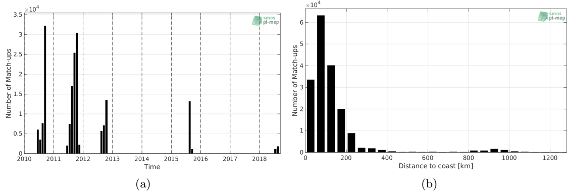
Figure 1: Number of match-ups between TSG-SAMOS and SMOS-L3-CATDS-CECOS-LOCEAN-V4-9DAYS-25KM SSS as a function of time (a) and as function of the distance to coast (b) over the Arctic Ocean Pi-MEP region and for the full satellite product period.
