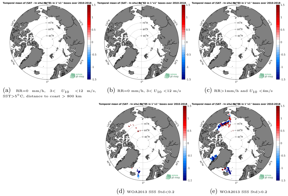
Figure 12: Temporal mean gridded over spatial boxes of size 1^\circ \times 1^\circ of \Delta SSS (SMOS-L3-CATDS-CECOS-LOCEAN-V4-9DAYS-25KM - TSG-SAMOS) for 5 different subdatasets corresponding to: RR=0 mm/h, 3 < U_{10} < 12 m/s, SST >5^\circ C, distance to coast > 800 km (a), RR=0 mm/h, 3 < U_{10} < 12 m/s (b), RR >1 mm/h and U_{10} < 4 m/s (c), WOA2013 SSS Std <0.2 (d), WOA2013 SSS Std >0.2 (e).
