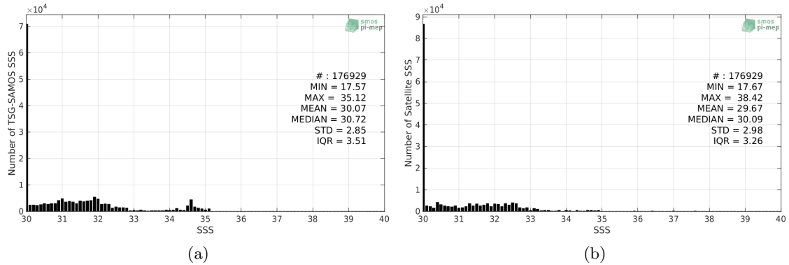
Figure 2: Histograms of SSS from TSG-SAMOS (a) and SMOS-L3-CATDS-CECOS-LOCEAN-V4-9DAYS-25KM (b) considering all match-up pairs per bins of 0.1 over the Arctic Ocean Pi-MEP region and for the full satellite product period.
