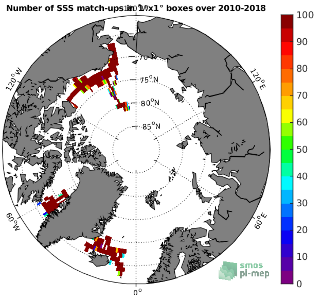
Figure 4: Number of SSS match-ups between TSG-SAMOS SSS and the SMOS-L3-CATDS-CECOS-LOCEAN-V4-9DAYS-25KM SSS product for the Arctic Ocean Pi-MEP region over 1°x1° boxes and for the full satellite product period.
