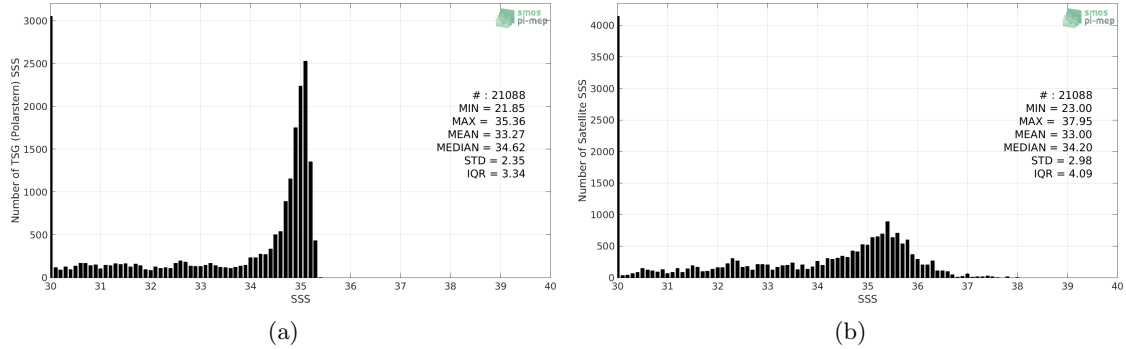
Figure 2: Histograms of SSS from TSG (Polarstern) (a) and SMOS SSS L3 v4 - 9 Days (CATDS-CECOS-LOCEAN) (b) considering all match-up pairs per bins of 0.1 over the Arctic Ocean Pi-MEP region and for the full satellite product period.
