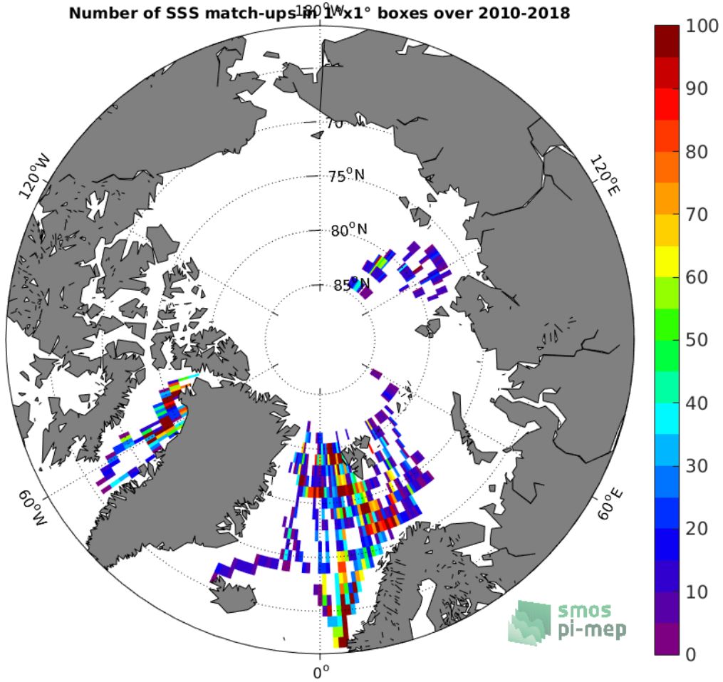
Figure 4: Number of SSS match-ups between TSG (Polarstern) SSS and the SMOS SSS L3 v4 - 9 Days (CATDS-CECOS-LOCEAN) SSS product for the Arctic Ocean Pi-MEP region over 1^\circ \times 1^\circ boxes and for the full satellite product period.
