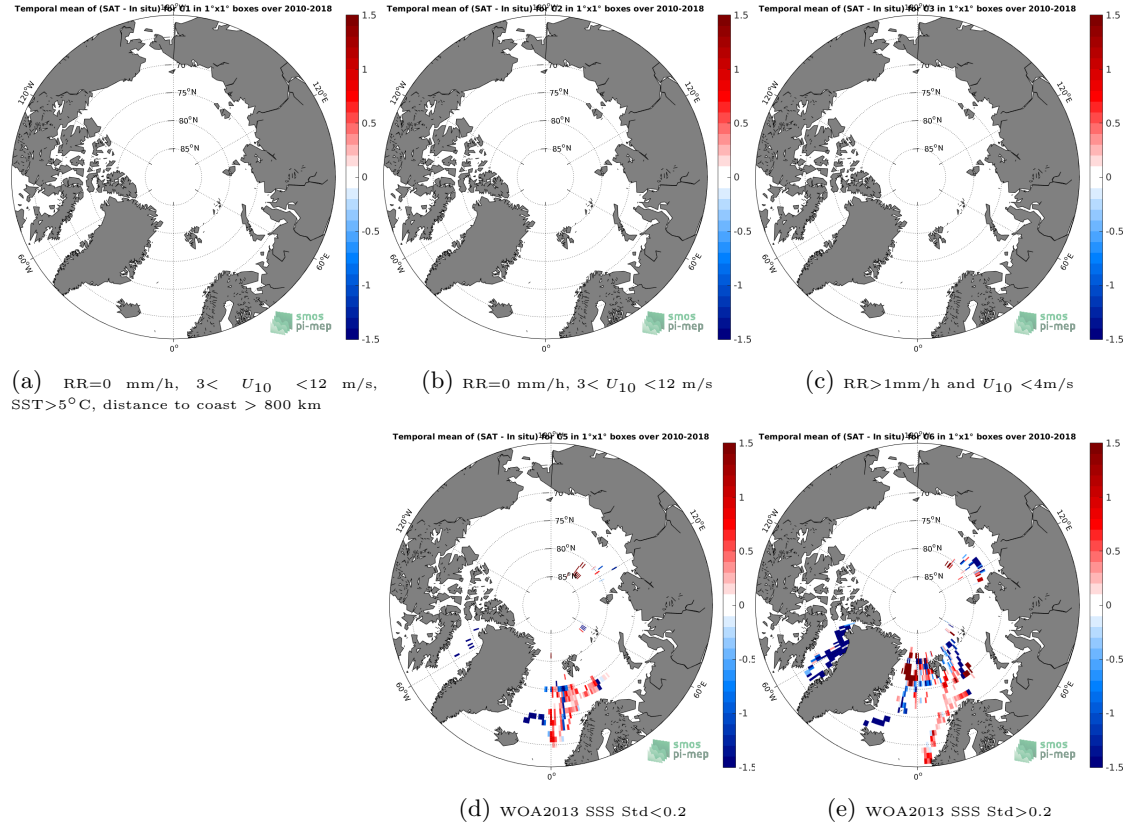
Figure 12: Temporal mean gridded over spatial boxes of size 1^{\circ}\times 1^{\circ} of \Delta\text{SSS} (SMOS SSS L3 v4 - 9 Days (CATDS-CECOS-LOCEAN) - TSG (Polarstern)) for 5 different subdatasets corresponding to: \text{RR}=0 mm/h, 3 < U_{10} < 12 m/s, \text{SST} > 5^{\circ}\text{C} , distance to coast > 800 km (a), \text{RR}=0 mm/h, 3 < U_{10} < 12 m/s (b), \text{RR} > 1 mm/h and U_{10} < 4 m/s (c), WOA2013 SSS Std < 0.2 (d), WOA2013 SSS Std > 0.2 (e).
