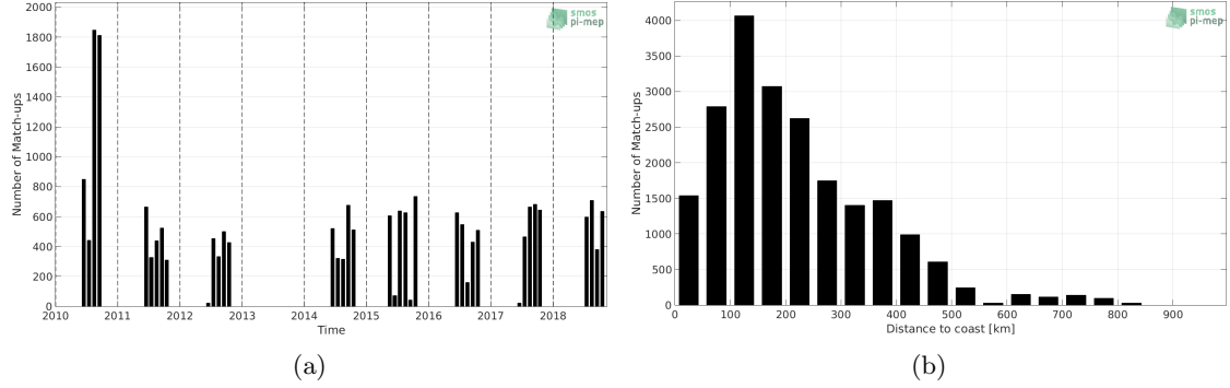
Figure 1: Number of match-ups between TSG (Polarstern) and SMOS SSS L3 v4 - 9 Days (CATDS-CECOS-LOCEAN) SSS as a function of time (a) and as function of the distance to coast (b) over the Arctic Ocean Pi-MEP region and for the full satellite product period.
