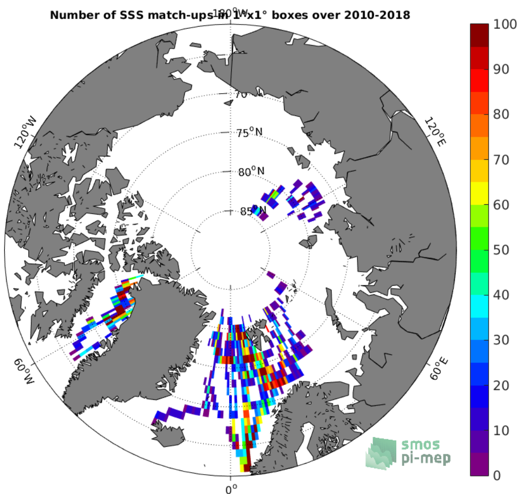
Figure 4: Number of SSS match-ups between TSG-POLARSTERN SSS and the SMOS-L3-CATDS-CECOS-LOCEAN-V4-9DAYS-25KM SSS product for the Arctic Ocean Pi-MEP region over 1^\circ \times 1^\circ boxes and for the full satellite product period.
