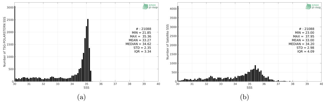
Figure 2: Histograms of SSS from TSG-POLARSTERN (a) and SMOS-L3-CATDS-CECOS-LOCEAN-V4-9DAYS-25KM (b) considering all match-up pairs per bins of 0.1 over the Arctic Ocean Pi-MEP region and for the full satellite product period.
