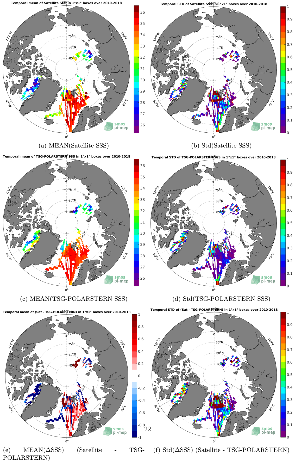
Figure 6: Temporal mean (left) and Std (right) of SSS from SMOS-L3-CATDS-CECOS-LOCEAN-V4-9DAYS-25KM (top), TSG-POLARSTERN (middle), and of \Delta SSS (Satellite - TSG-POLARSTERN). Only match-up pairs are used to generate these maps.
