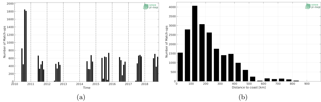
Figure 1: Number of match-ups between TSG-POLARSTERN and SMOS-L3-CATDS-CECOS-LOCEAN-V4-9DAYS-25KM SSS as a function of time (a) and as function of the distance to coast (b) over the Arctic Ocean Pi-MEP region and for the full satellite product period.
