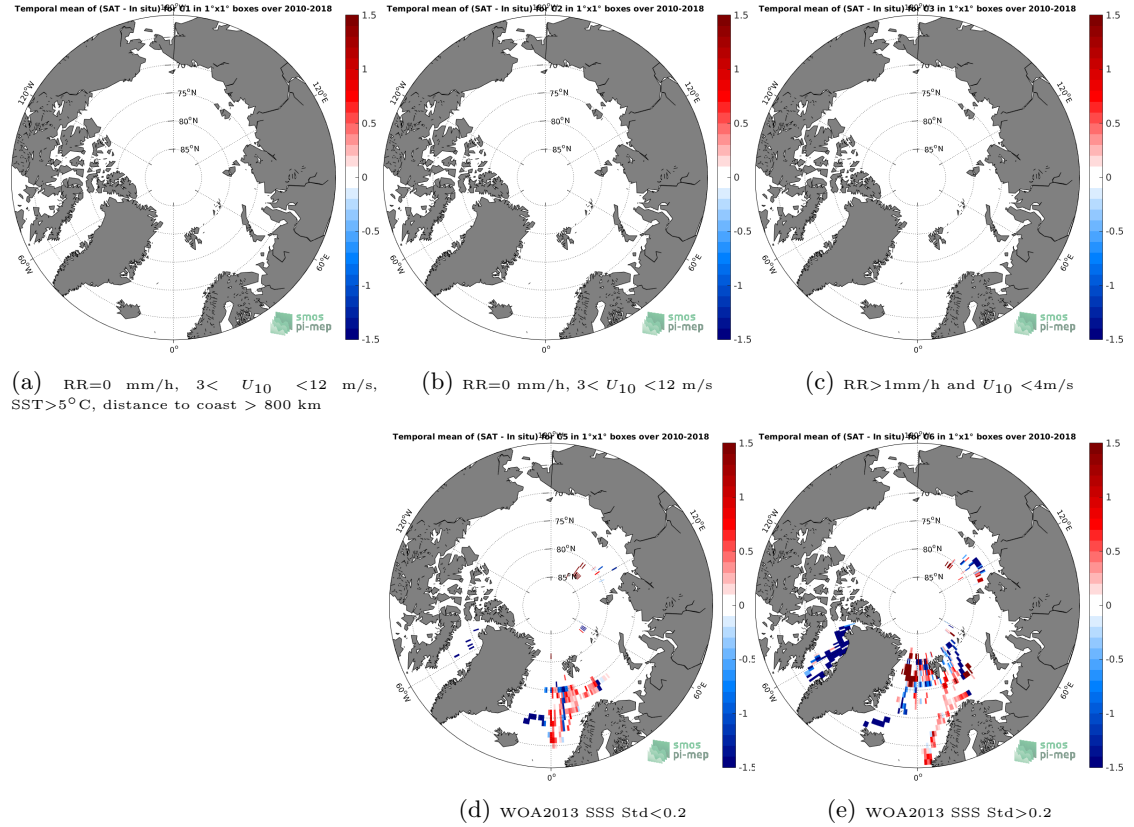
Figure 12: Temporal mean gridded over spatial boxes of size 1^{\circ}\times 1^{\circ} of \Delta\text{SSS} (SMOS-L3-CATDS-CECOS-LOCEAN-V4-9DAYS-25KM - TSG-POLARSTERN) for 5 different subdatasets corresponding to:RR=0 mm/h, 3 < U_{10} < 12 m/s, SST >5^{\circ}\text{C} , distance to coast > 800 km (a), RR=0 mm/h, 3 < U_{10} < 12 m/s (b), RR >1 mm/h and U_{10} < 4 m/s (c), WOA2013 SSS Std <0.2 (d), WOA2013 SSS Std >0.2 (e).
