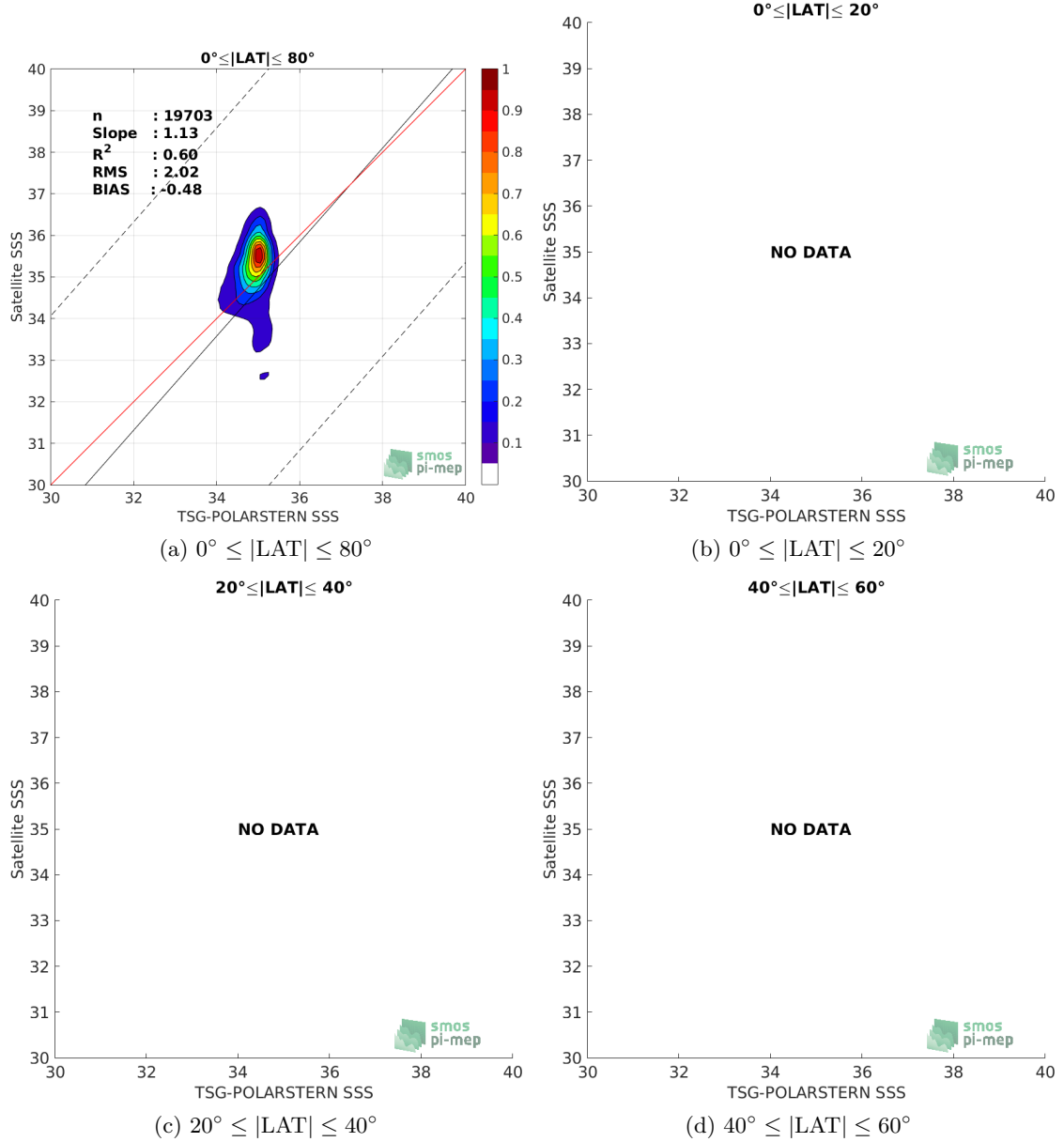
Figure 9: Contour maps of the concentration of SMOS-L3-CATDS-CECOS-LOCEAN-V4-9DAYS-25KM SSS (y-axis) versus TSG-POLARSTERN SSS (x-axis) at match-up pairs for different latitude bands. For each plot, the red line shows x=y . The black thin and dashed lines indicate a linear fit through the data cloud and the \pm 95\% confidence levels, respectively. The number match-up pairs n , the slope and R^2 coefficient of the linear fit, the root mean square (RMS) and the mean bias between satellite and in situ data are indicated for each latitude band in each plots.
