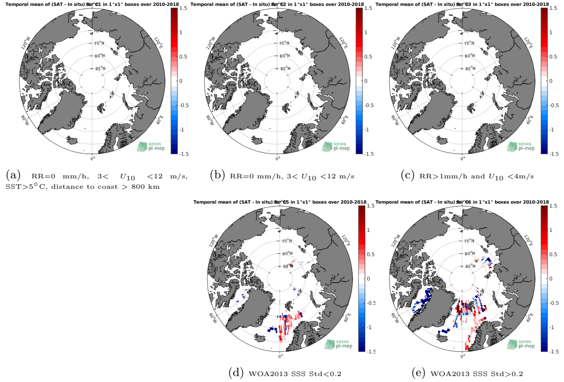
Figure 12: Temporal mean gridded over spatial boxes of size 1^\circ \times 1^\circ of \Delta SSS (SMOS-L3-CATDS-CECOS-LOCEAN-V4-9DAYS-25KM - TSG-POLARSTERN) for 5 different subdatasets corresponding to:RR=0 mm/h, 3 < U_{10} < 12 m/s, SST >5^\circ\text{C} , distance to coast > 800 km (a), RR=0 mm/h, 3 < U_{10} < 12 m/s (b), RR >1 mm/h and U_{10} < 4 m/s (c), WOA2013 SSS Std <0.2 (d), WOA2013 SSS Std >0.2 (e).
