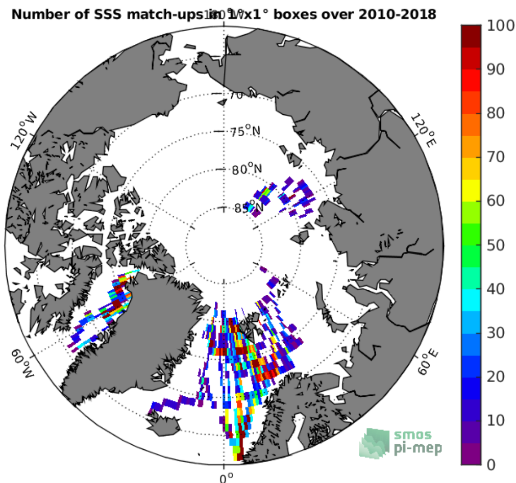
Figure 4: Number of SSS match-ups between TSG-POLARSTERN SSS and the SMOS-L3-CATDS-CECOS-LOCEAN-V4-9DAYS-25KM SSS product for the Arctic Ocean Pi-MEP region over 1°x1° boxes and for the full satellite product period.
