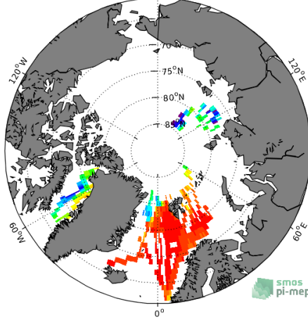
(c) MEAN(TSG-POLARSTERN SSS)
