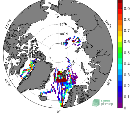
(f) Std( \Delta SSS) (Satellite - TSG-POLARSTERN)
