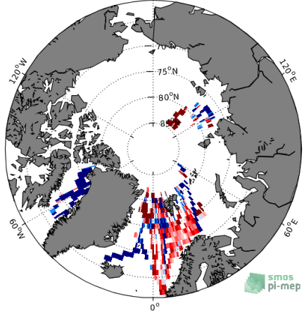
(e) MEAN( \Delta SSS) (Satellite - TSG-POLARSTERN)
