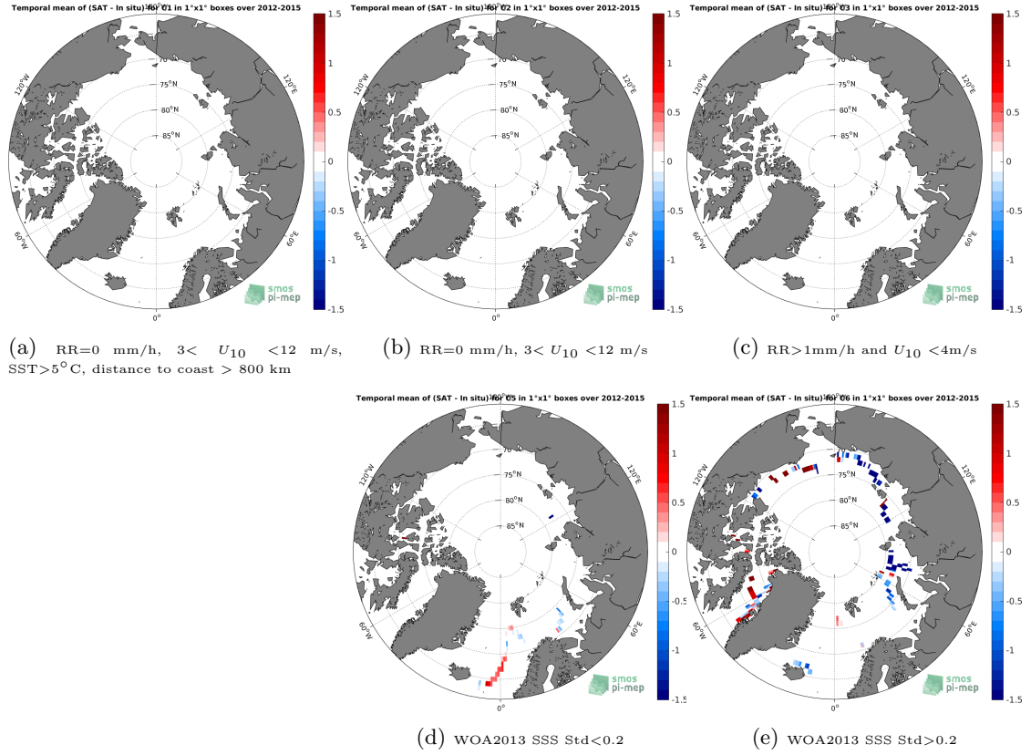
Figure 12: Temporal mean gridded over spatial boxes of size 1°x1° of \Delta SSS (SMOS SSS L3 v4 - 9 Days (CATDS-CECOS-LOCEAN) - TSG (GOSUD-Sailing-ship)) for 5 different subdatasets corresponding to: RR=0 mm/h, 3 < U_{10} < 12 m/s, SST>5°C, distance to coast > 800 km (a), RR=0 mm/h, 3 < U_{10} < 12 m/s (b), RR>1mm/h and U_{10} < 4 m/s (c), WOA2013 SSS Std<0.2 (d), WOA2013 SSS Std>0.2 (e).
