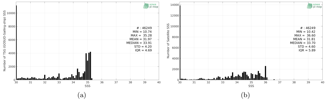
Figure 2: Histograms of SSS from TSG (GOSUD-Sailing-ship) (a) and SMOS SSS L3 v4 - 9 Days (CATDS-CECOS-LOCEAN) (b) considering all match-up pairs per bins of 0.1 over the Arctic Ocean Pi-MEP region and for the full satellite product period.
