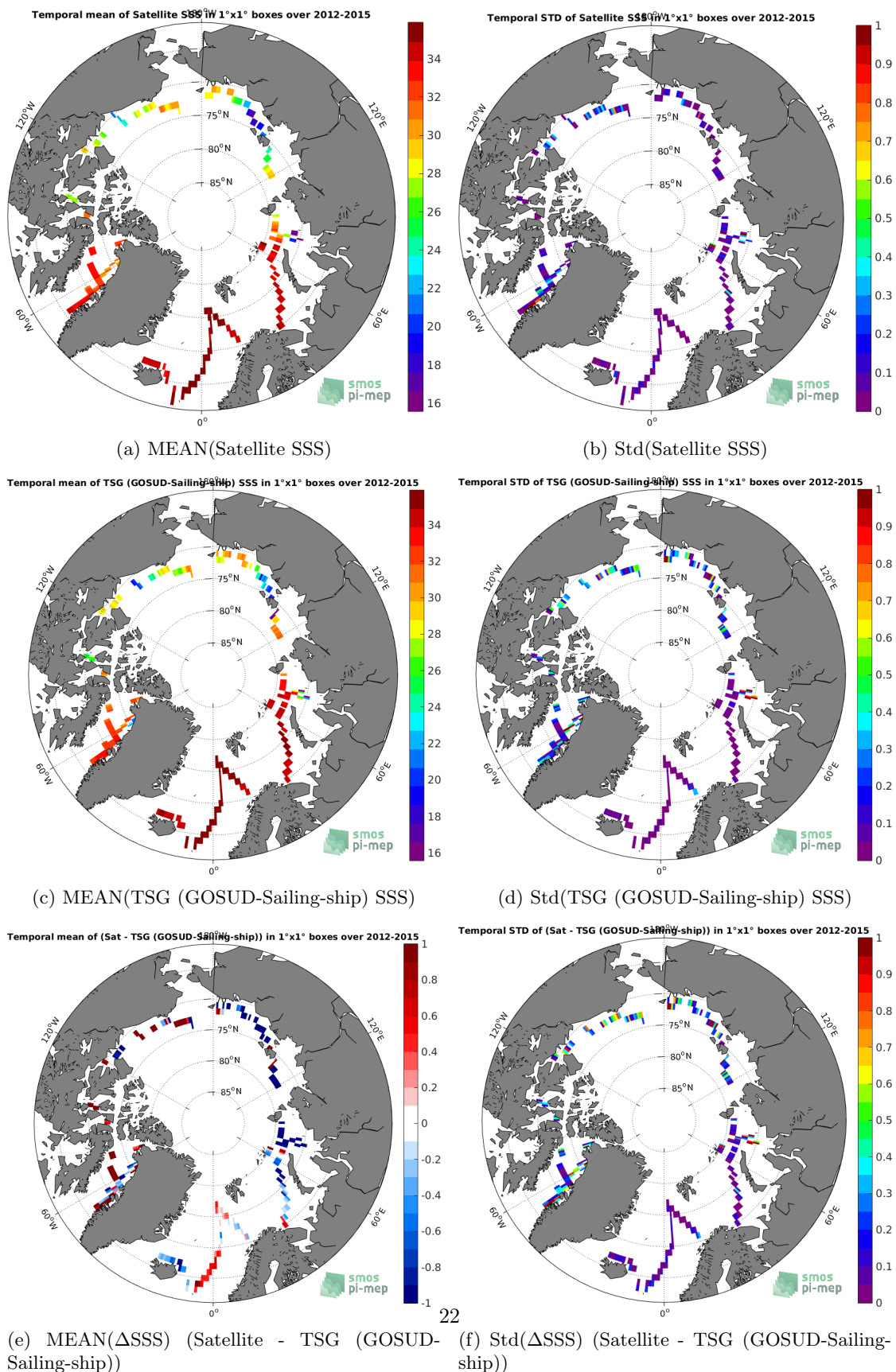
Figure 6: Temporal mean (left) and Std (right) of SSS from SMOS SSS L3 v4 - 9 Days (CATDS-CECOS-LOCEAN) (top), TSG (GOSUD-Sailing-ship) (middle), and of \Delta SSS (Satellite - TSG (GOSUD-Sailing-ship)). Only match-up pairs are used to generate these maps.
