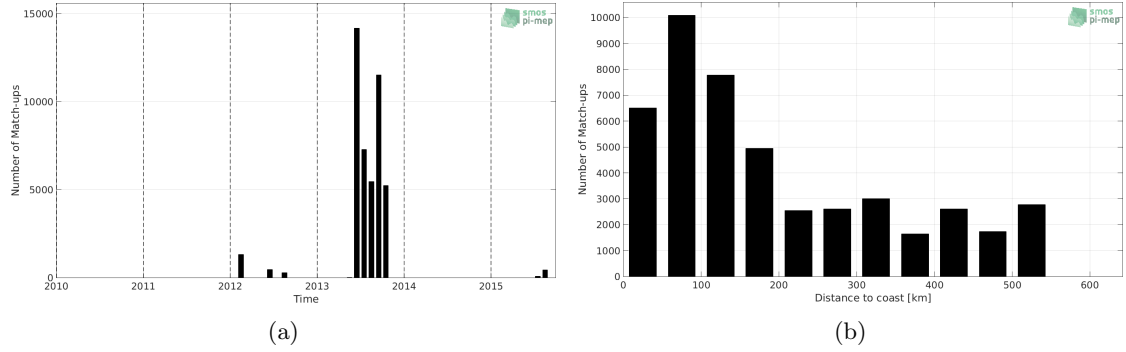
Figure 1: Number of match-ups between TSG (GOSUD-Sailing-ship) and SMOS SSS L3 v4 - 9 Days (CATDS-CECOS-LOCEAN) SSS as a function of time (a) and as function of the distance to coast (b) over the Arctic Ocean Pi-MEP region and for the full satellite product period.
