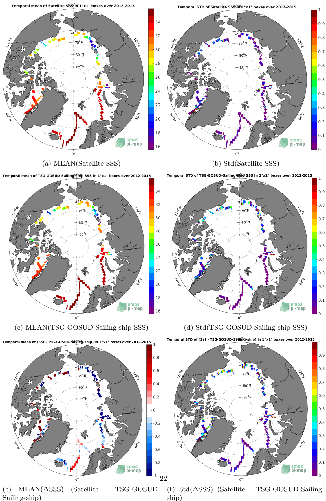
Figure 6: Temporal mean (left) and Std (right) of SSS from SMOS-L3-CATDS-CECOS-LOCEAN-V4-9DAYS-25KM (top), TSG-GOSUD-Sailing-ship (middle), and of \Delta SSS (Satellite - TSG-GOSUD-Sailing-ship). Only match-up pairs are used to generate these maps.
