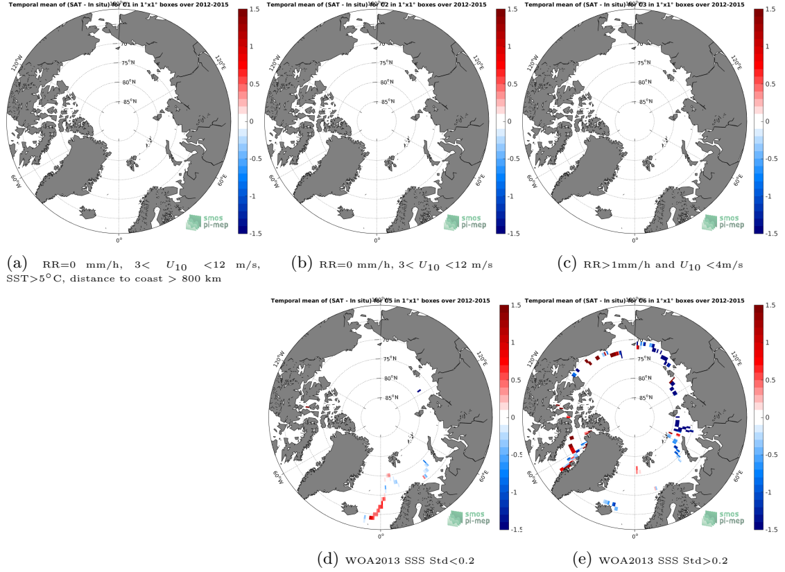
Figure 12: Temporal mean gridded over spatial boxes of size 1^{\circ} \times 1^{\circ} of \Delta\text{SSS} (SMOS-L3-CATDS-CECOS-LOCEAN-V4-9DAYS-25KM - TSG-GOSUD-Sailing-ship) for 5 different subdatasets corresponding to: RR=0 mm/h, 3 < U_{10} < 12 m/s, SST > 5^{\circ}\text{C} , distance to coast > 800 km (a), RR=0 mm/h, 3 < U_{10} < 12 m/s (b), RR > 1\text{mm/h} and U_{10} < 4\text{m/s} (c), WOA2013 SSS Std < 0.2 (d), WOA2013 SSS Std > 0.2 (e).
